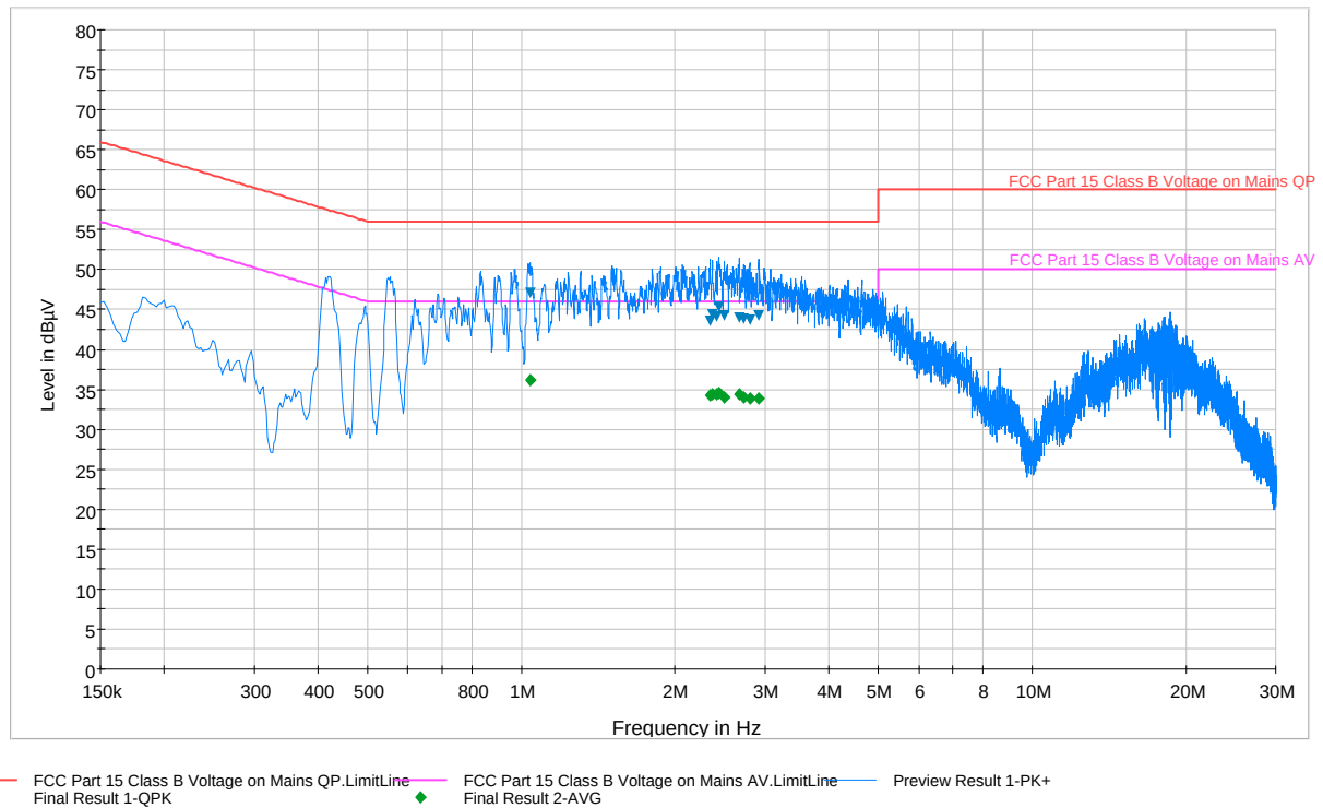
Plot 6-25. Line-Conducted Test Plot (N)
