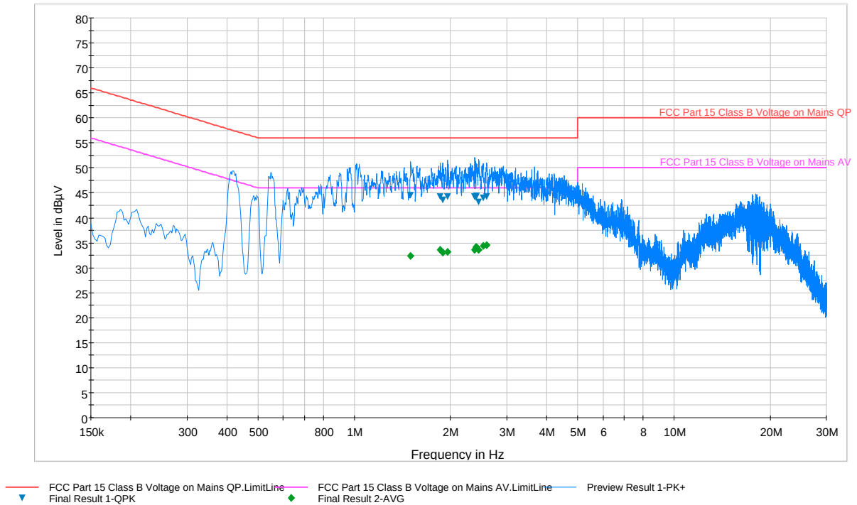
Plot 6-61. Line Conducted Plot with 802.11b (N)
