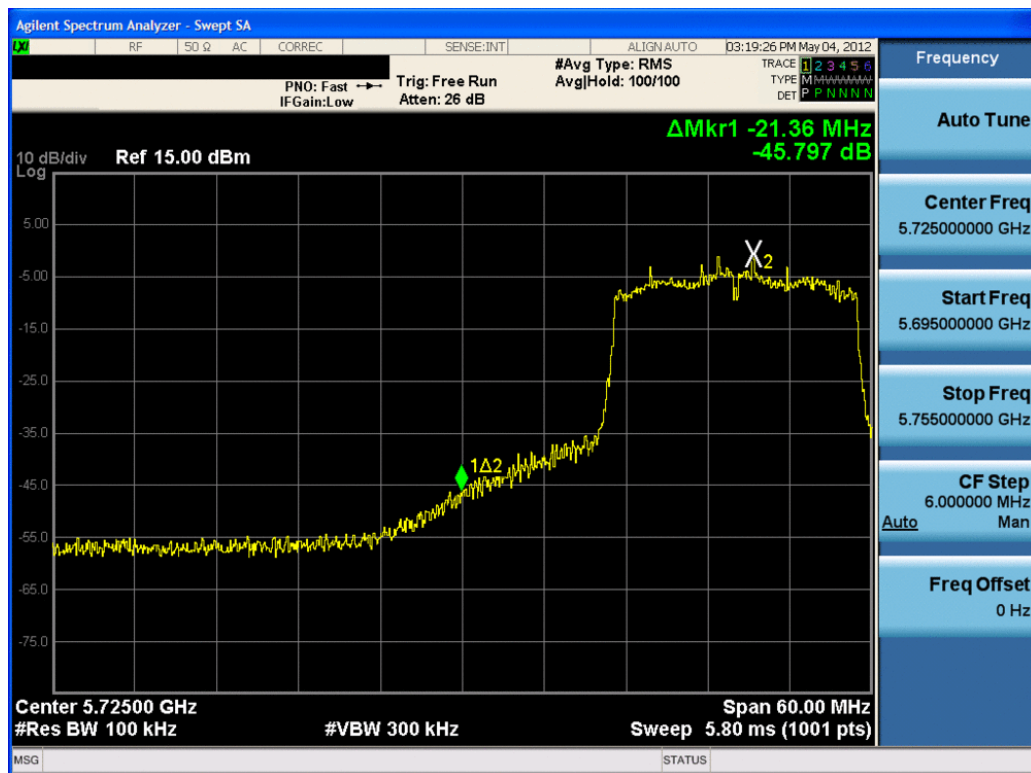
Plot 6-43. Band Edge Plot (802.11n (5.8GHz – 20MHz) – Ch. 149)
