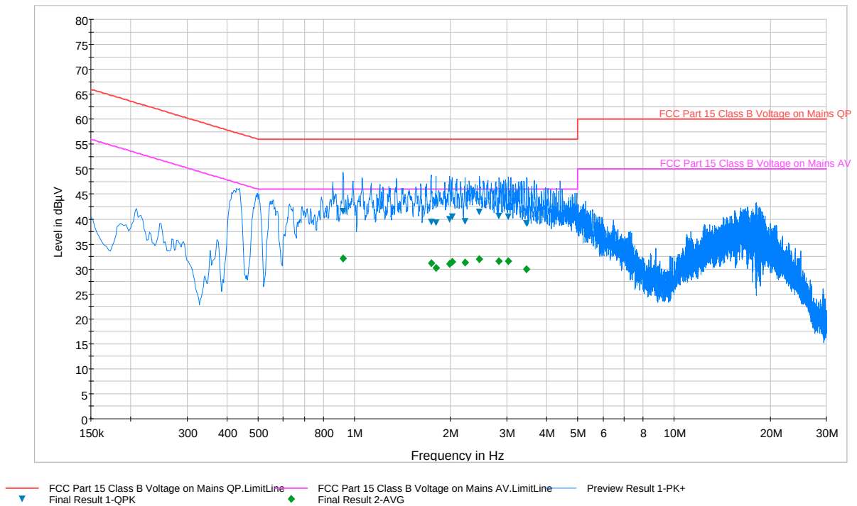
Plot 6-62. Line Conducted Plot with 802.11a (L1)
