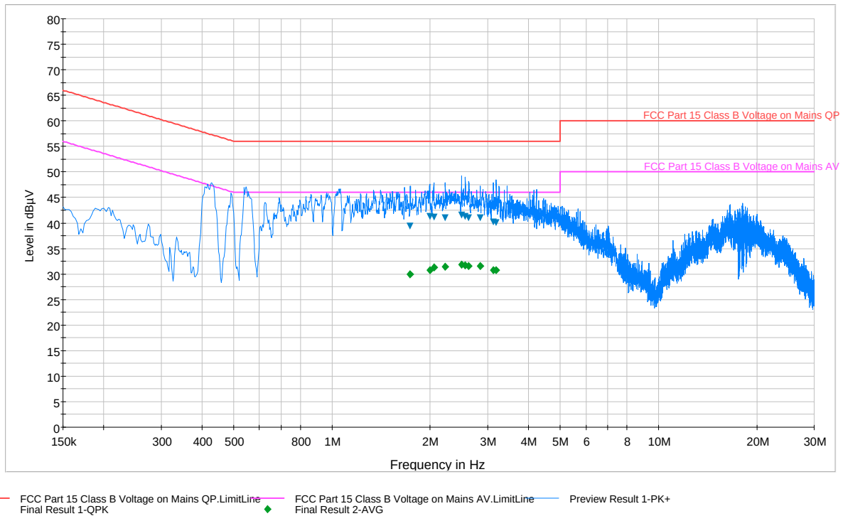
Plot 6-57. Line Conducted Plot with 802.11b (L1)
