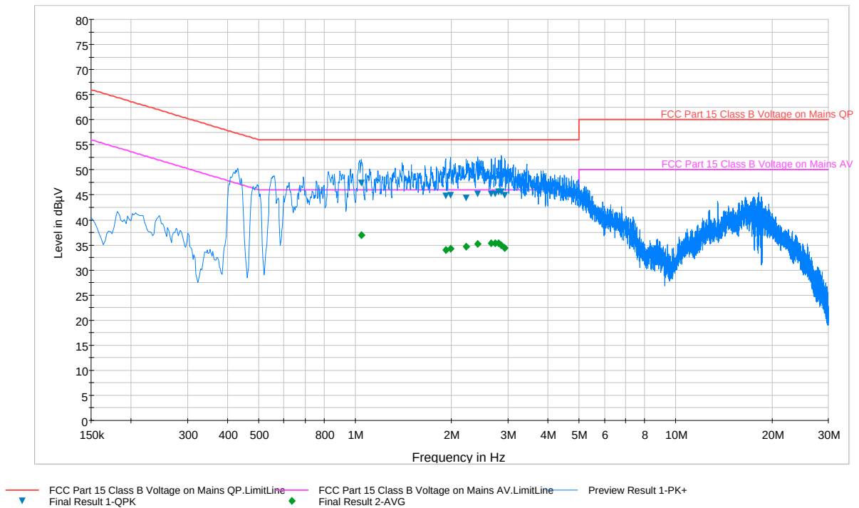
Plot 6-63. Line Conducted Plot with 802.11a (N)
