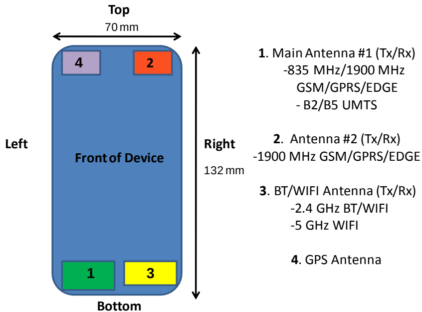
Figure 1-1 DUT Antenna Locations
