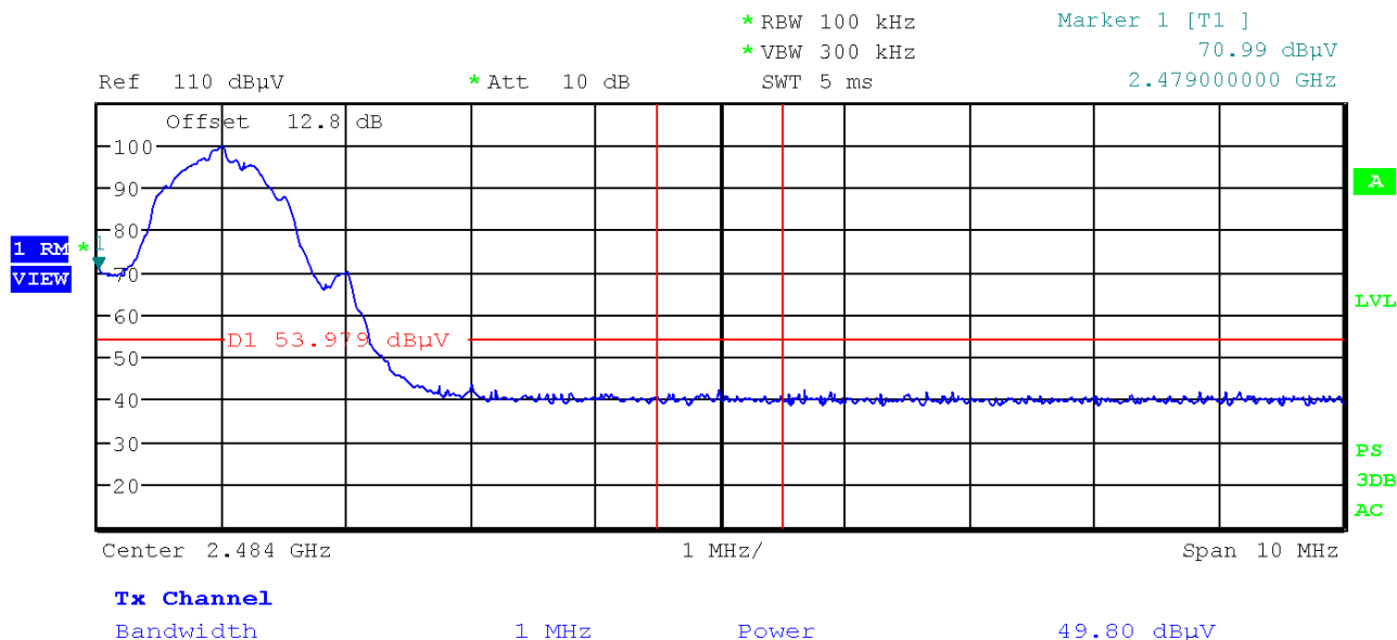
Plot 6-1515. Radiated Restricted Upper Band Edge Measurement (Average)
