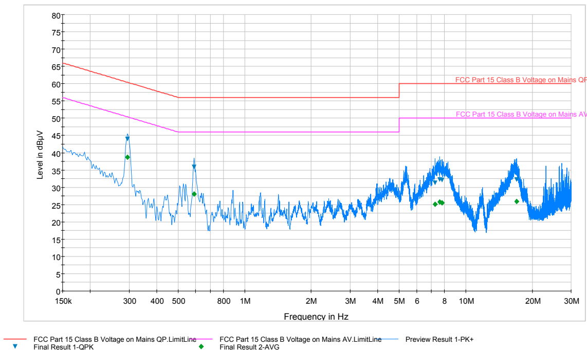
Plot 6-18. Line Conducted Plot with Bluetooth LE (N)
