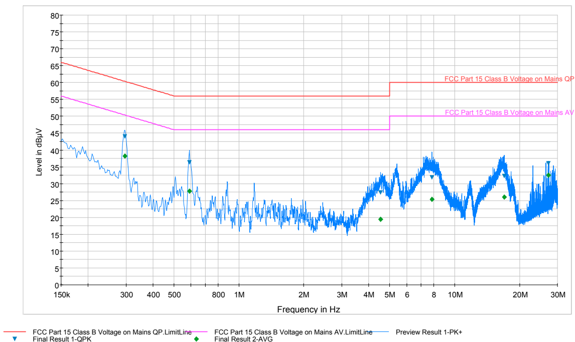
Plot 6-17. Line Conducted Plot with Bluetooth LE (L1)
