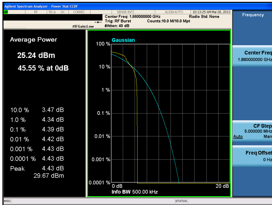
Plot 7-34. Peak-Average Ratio Plot (EDGE1900 Mode, Ant. 2 – Ch. 661)
