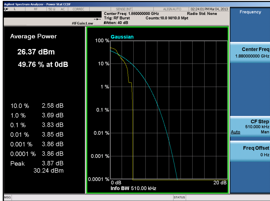
Plot 7-22. Peak-Average Ratio Plot (EDGE1900 Mode, Ant. 1 – Ch. 661)
