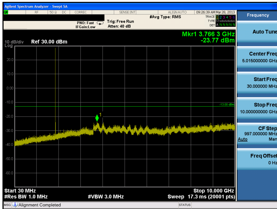
Plot 7-26. Conducted Spurious Plot (PCS GSM Mode, Ant. 2 – Ch. 661)
