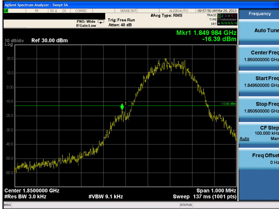
Plot 7-25. Band Edge Plot (PCS GSM Mode, Ant. 2 – Ch. 512)
