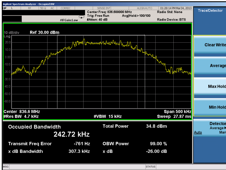
Plot 7-10. Occupied Bandwidth Plot (EDGE850 Mode – Ch. 190)
