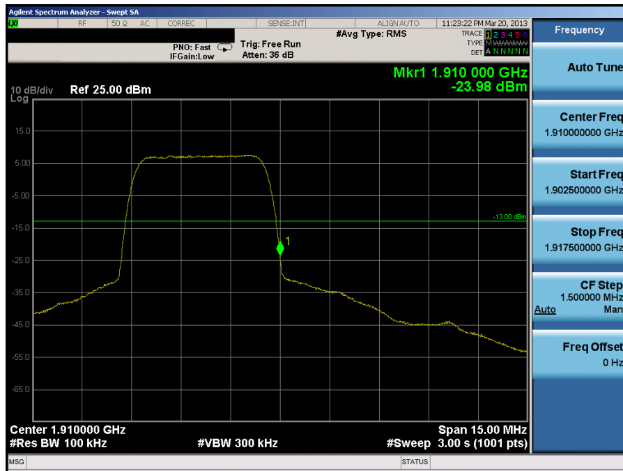
Plot 7-54. Band Edge Plot (PCS WCDMA Mode – Ch. 9538)
