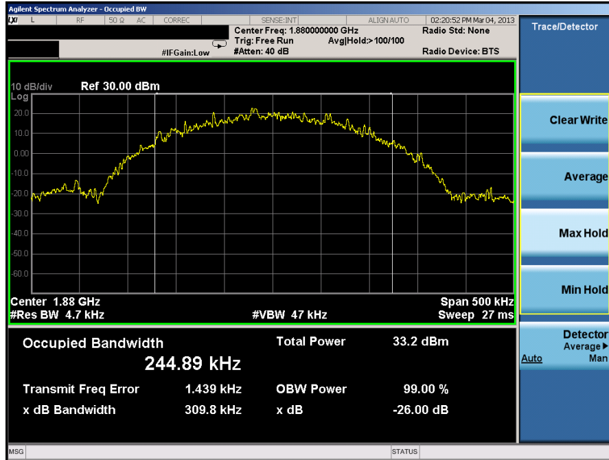
Plot 7-21. Occupied Bandwidth Plot (EDGE1900 Mode, Ant. 1 – Ch. 661)
