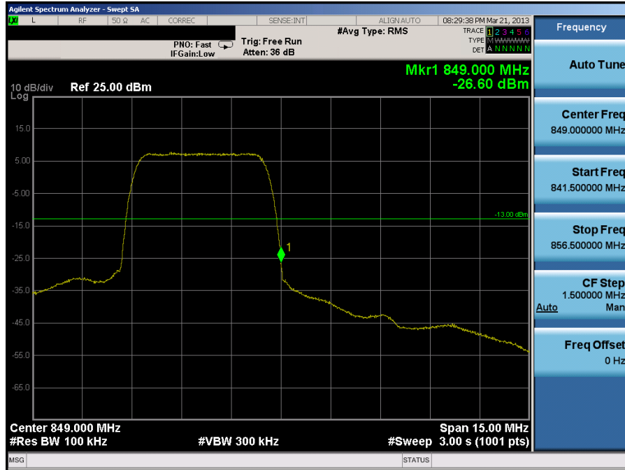
Plot 7-43. Band Edge Plot (Cellular WCDMA Mode – Ch. 4233)
