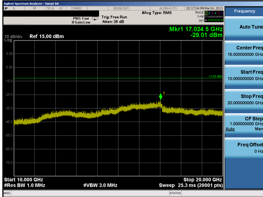
Plot 7-19. Conducted Spurious Plot (PCS GSM Mode, Ant. 1 - Ch. 810)
