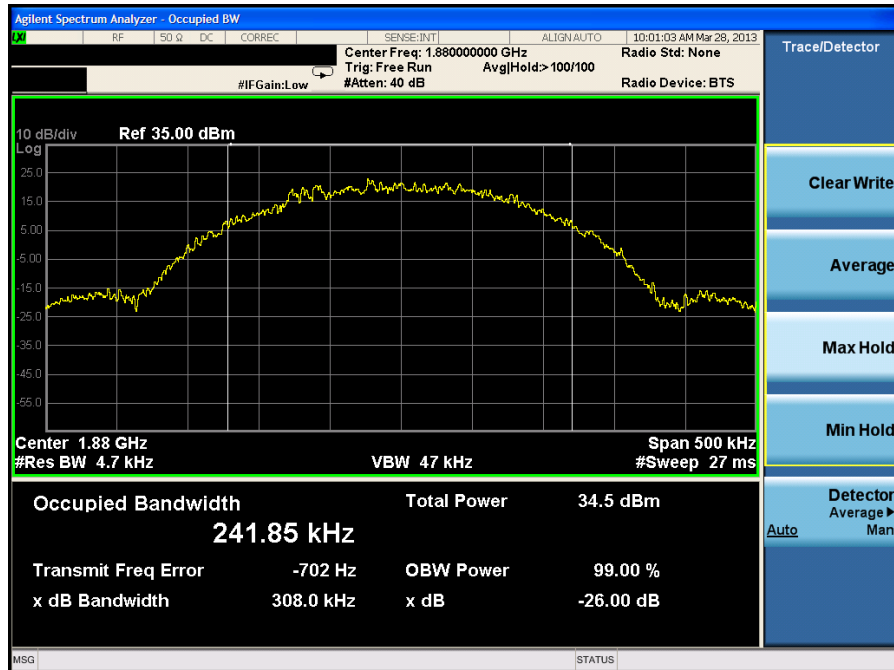
Plot 7-33. Occupied Bandwidth Plot (EDGE1900 Mode, Ant. 2 – Ch. 661)
