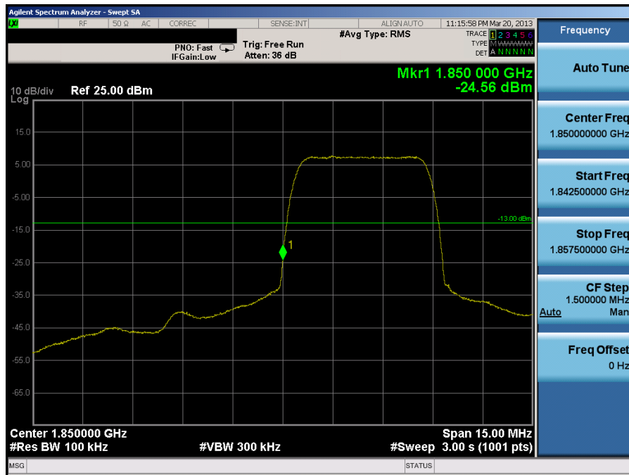
Plot 7-46. Band Edge Plot (PCS WCDMA Mode – Ch. 9262)
