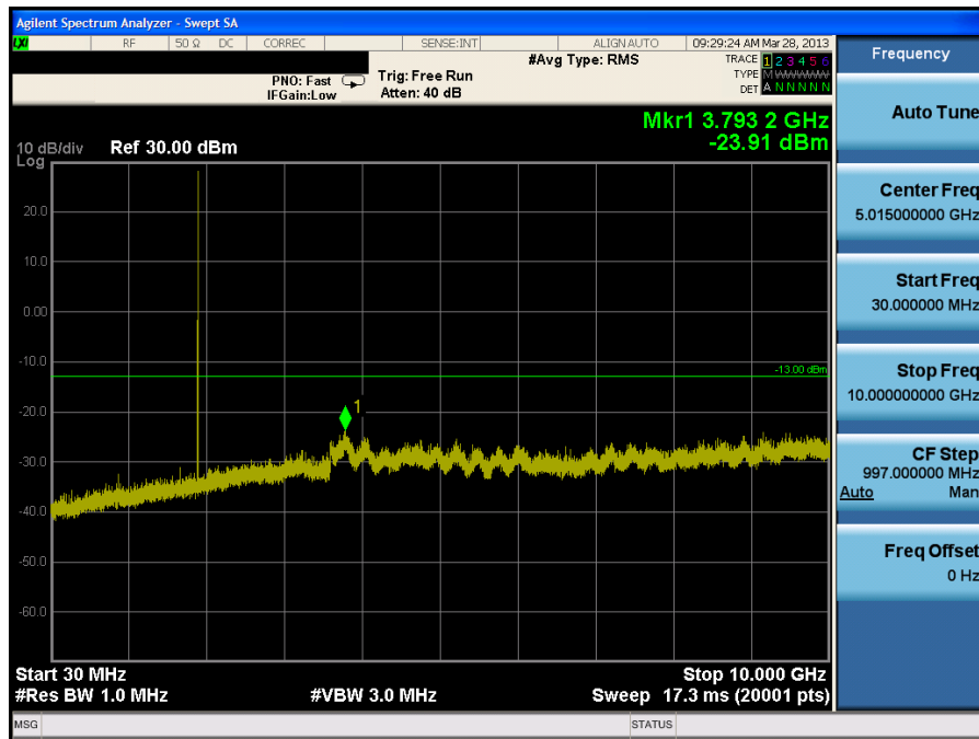
Plot 7-30. Conducted Spurious Plot (PCS GSM Mode, Ant. 2 – Ch. 810)
