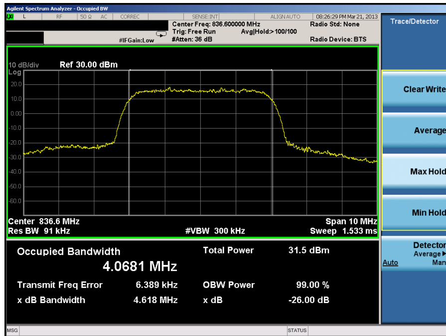
Plot 7-40. Occupied Bandwidth Plot (Cellular WCDMA Mode – Ch. 4183)
