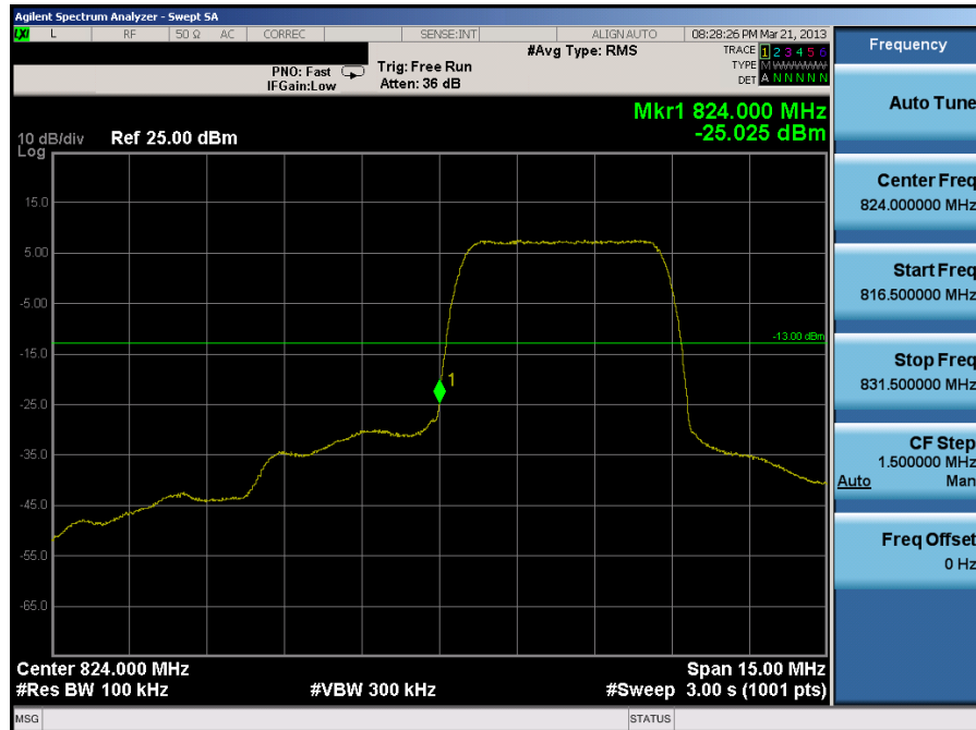
Plot 7-37. Band Edge Plot (Cellular WCDMA Mode – Ch. 4132)
