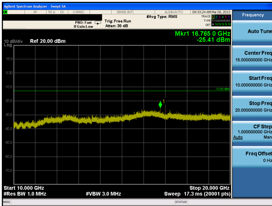
Plot 7-24. Conducted Spurious Plot (PCS GSM Mode, Ant. 2 – Ch. 512)
