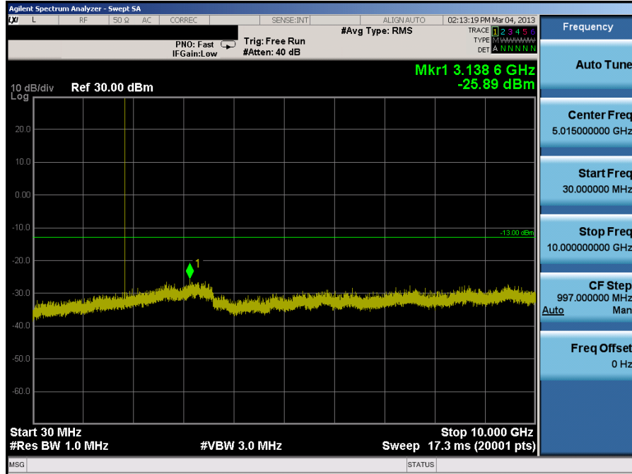
Plot 7-11. Conducted Spurious Plot (PCS GSM Mode, Ant. 1 – Ch. 512)
