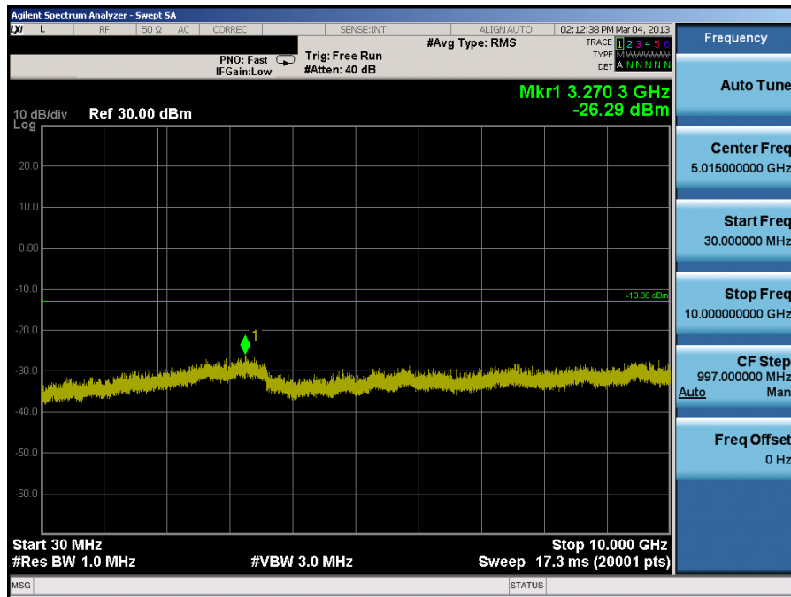
Plot 7-14. Conducted Spurious Plot (PCS GSM Mode, Ant. 1 – Ch. 661)
