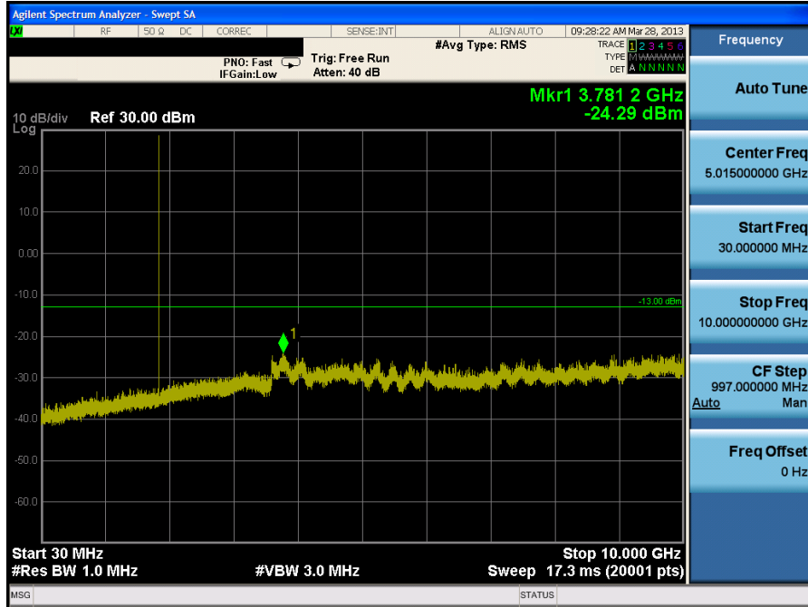
Plot 7-23. Conducted Spurious Plot (PCS GSM Mode, Ant. 2 – Ch. 512)
