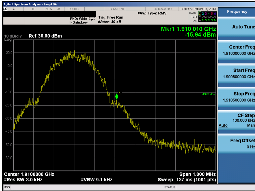
Plot 7-20. Band Edge Plot (PCS GSM Mode, Ant. 1 - Ch. 810)
