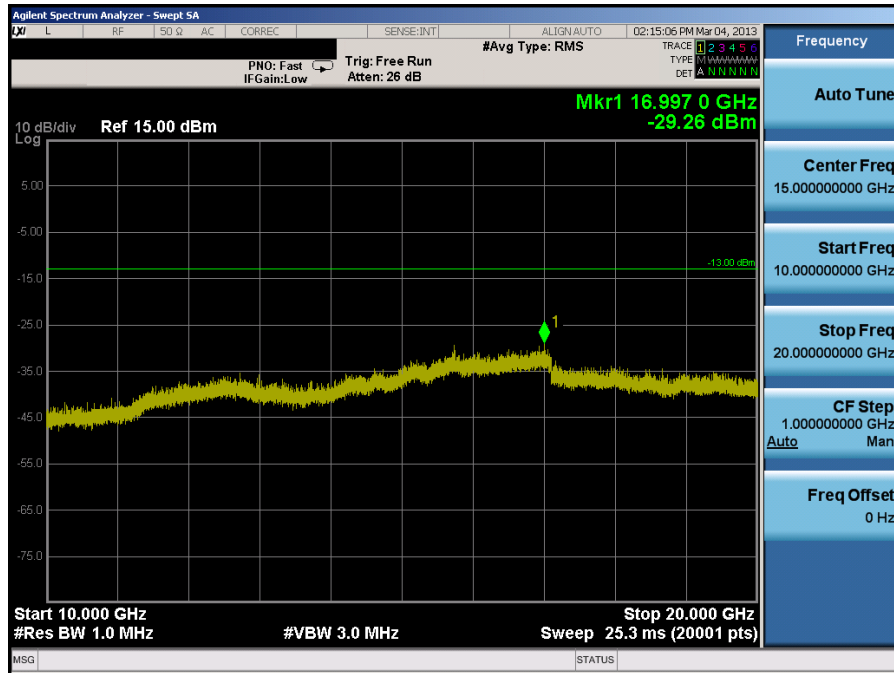
Plot 7-12. Conducted Spurious Plot (PCS GSM Mode, Ant. 1 – Ch. 512)
