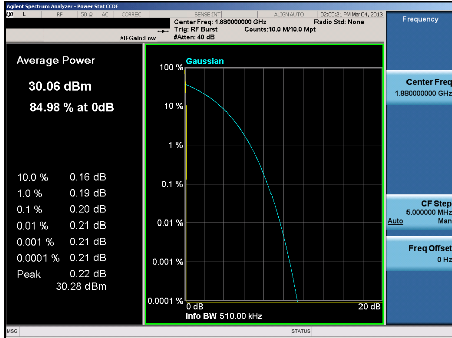
Plot 7-17. Peak-Average Ratio Plot (PCS GSM Mode, Ant. 1 – Ch. 661)
