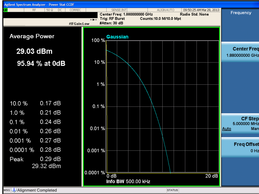
Plot 7-29. Peak-Average Ratio Plot (PCS GSM Mode, Ant. 2 – Ch. 661)
