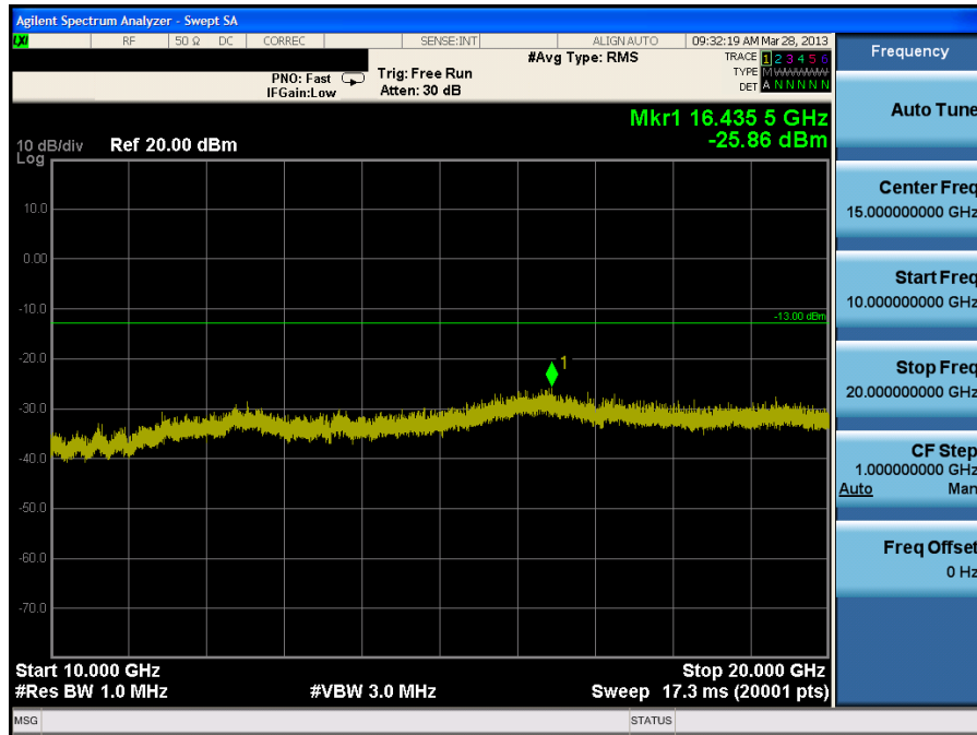
Plot 7-27. Conducted Spurious Plot (PCS GSM Mode, Ant. 2 – Ch. 661)
