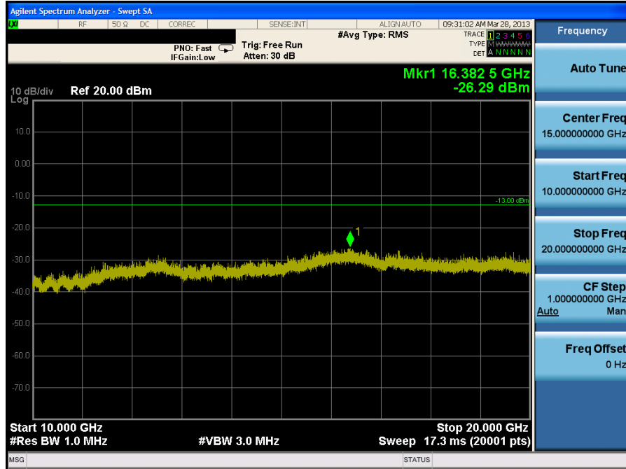
Plot 7-31. Conducted Spurious Plot (PCS GSM Mode, Ant. 2 – Ch. 810)
