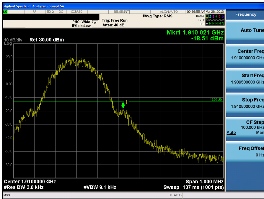
Plot 7-32. Band Edge Plot (PCS GSM Mode, Ant. 2 – Ch. 810)
