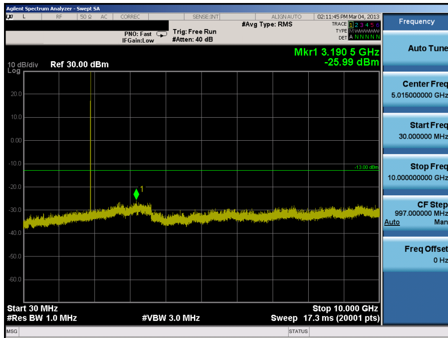
Plot 7-18. Conducted Spurious Plot (PCS GSM Mode, Ant. 1 – Ch. 810)
