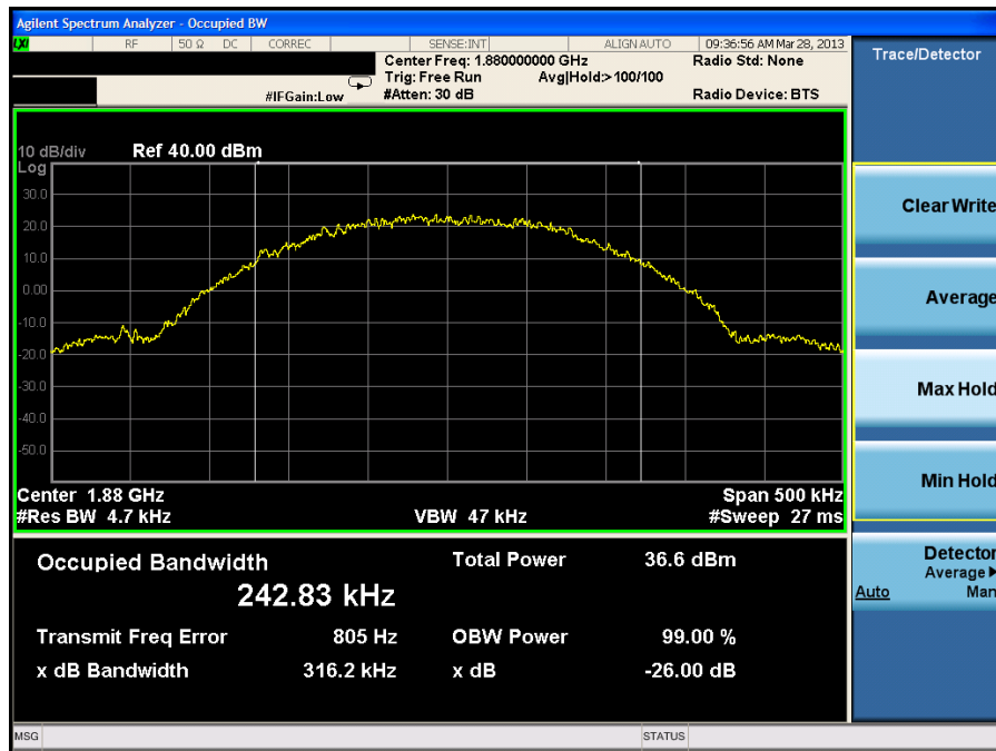
Plot 7-28. Occupied Bandwidth Plot (PCS GSM Mode, Ant. 2 – Ch. 661)
