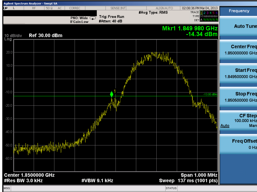
Plot 7-13. Band Edge Plot (PCS GSM Mode, Ant. 1 – Ch. 512)
