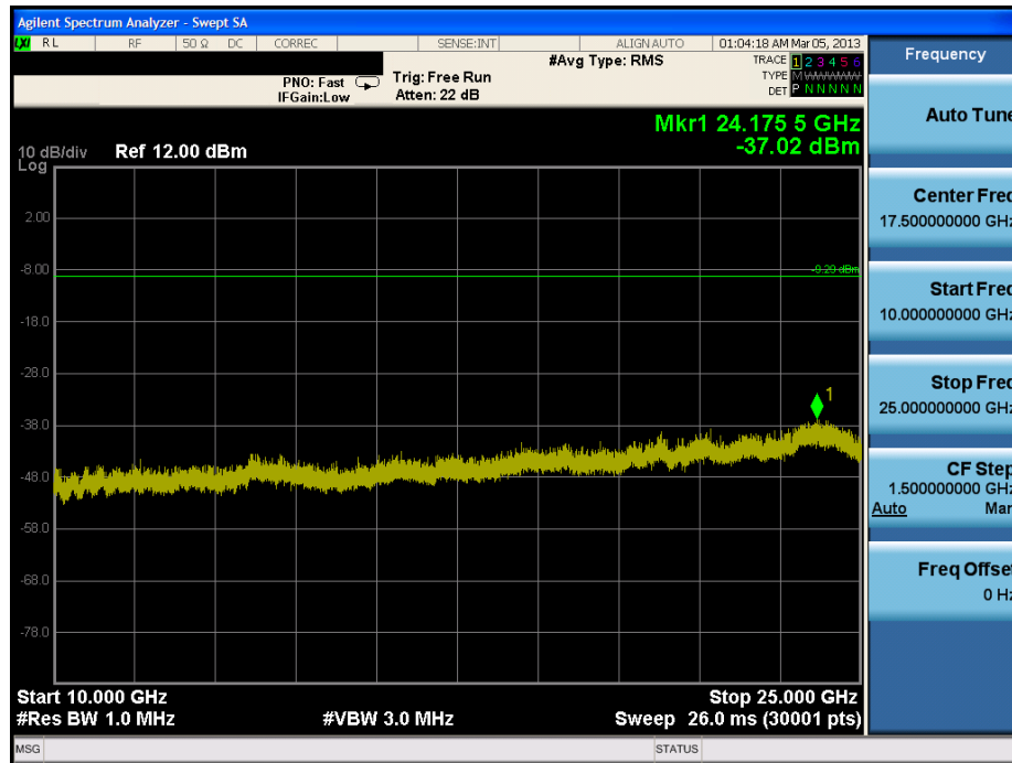
Plot 6-39. Conducted Spurious Plot (Bluetooth, 3Mbps – Ch. 39)
