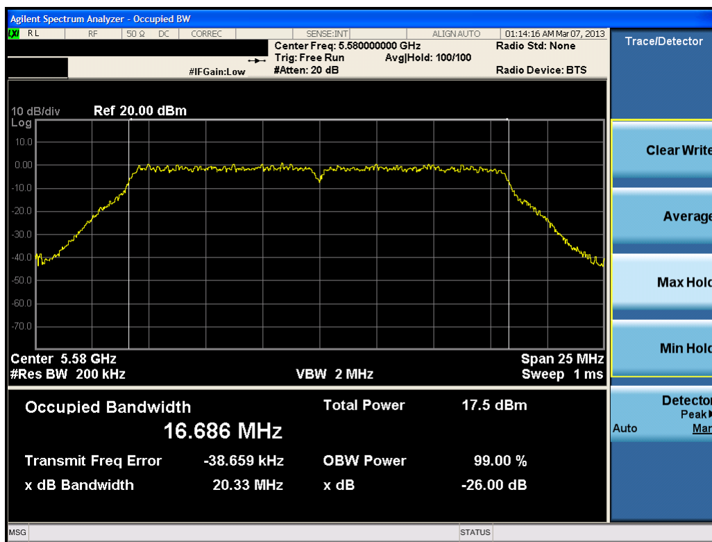
Plot 6-18. 26dB Bandwidth Plot (802.11a (UNII Band 3) – Ch. 116)
