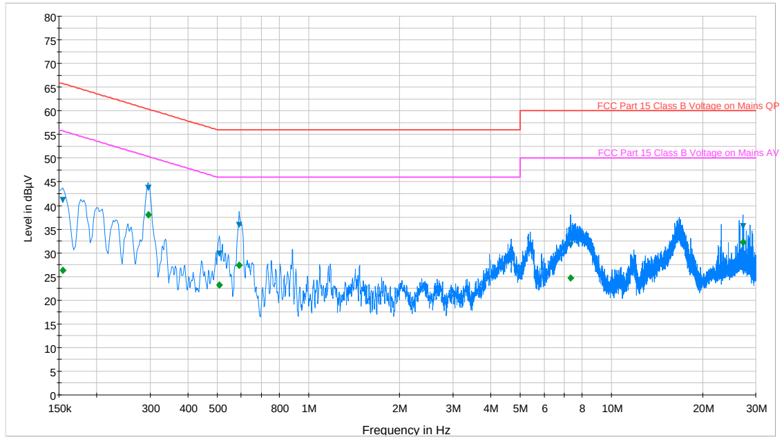
Plot 6-83. Line Conducted Plot with 802.11a UNII Band 2 (L1)
