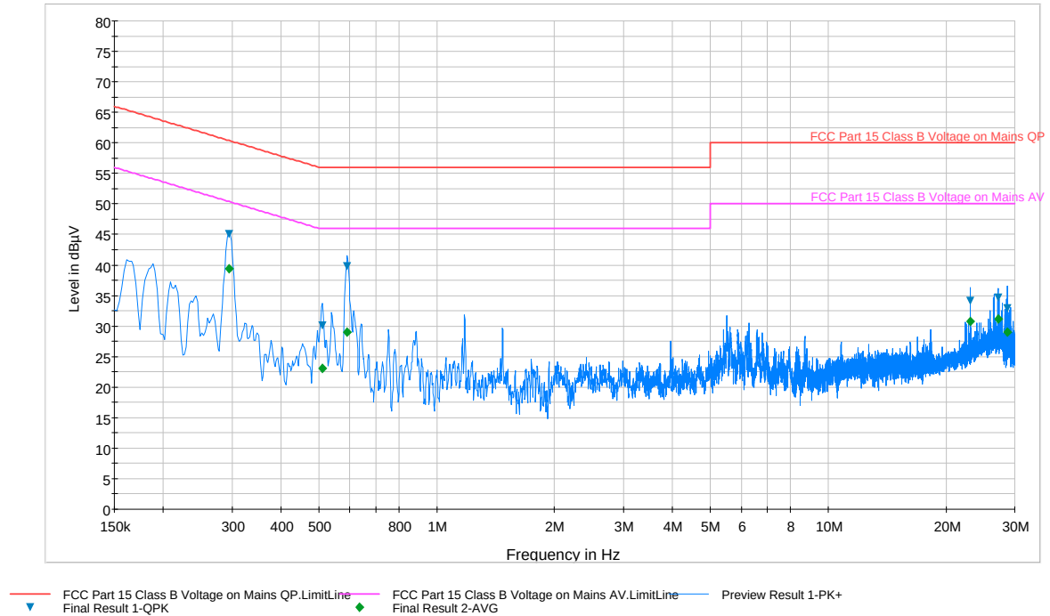
Plot 6-81. Line Conducted Plot with 802.11a UNII Band 1 (L1)
