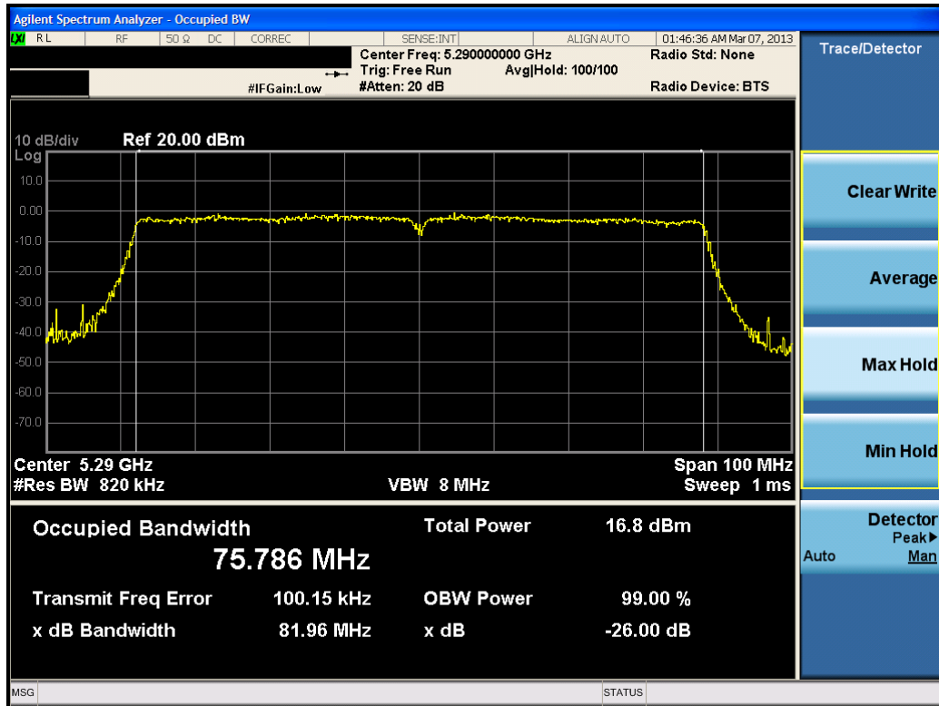
Plot 6-27. 26dB Bandwidth Plot (80MHz BW 802.11ac (UNII Band 2) – Ch. 58)
