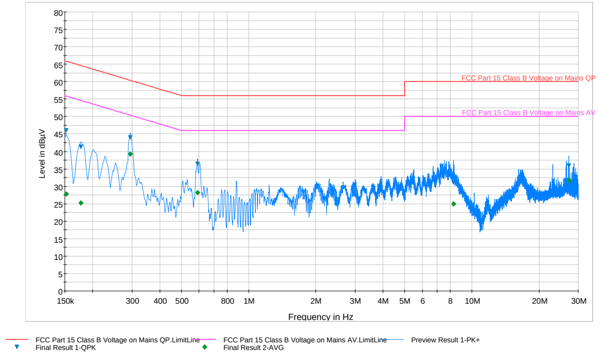
Plot 6-86. Line Conducted Plot with 802.11a UNII Band 3 (N)
