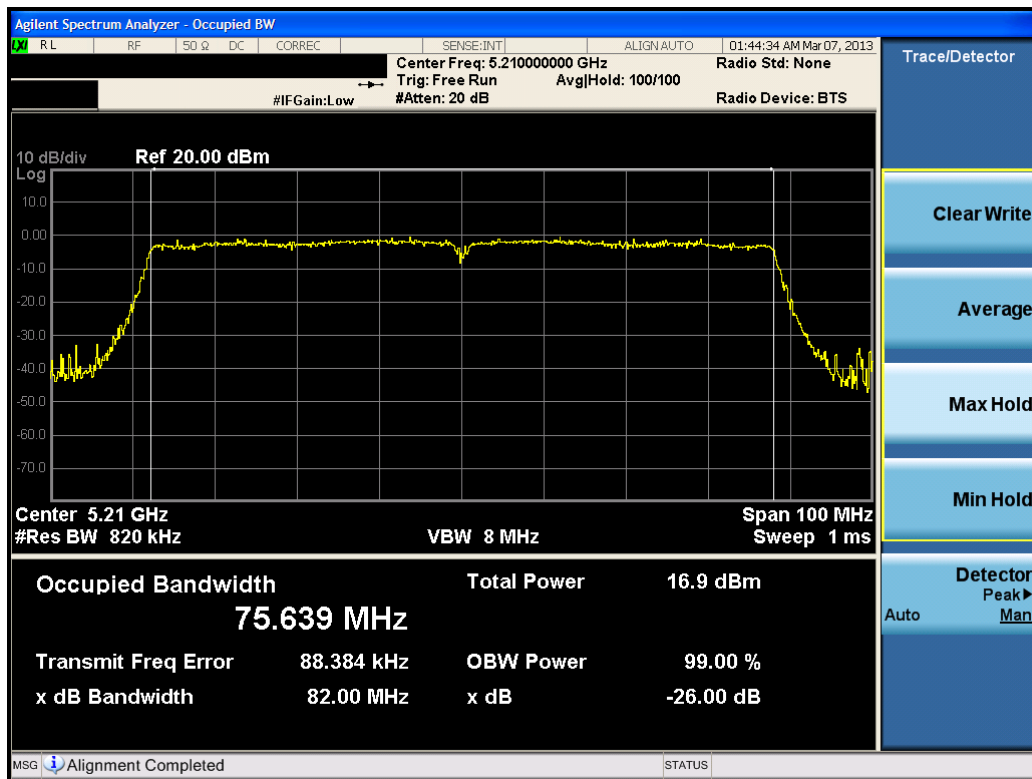
Plot 6-26. 26dB Bandwidth Plot (80MHz BW 802.11ac (UNII Band 1) – Ch. 42)
