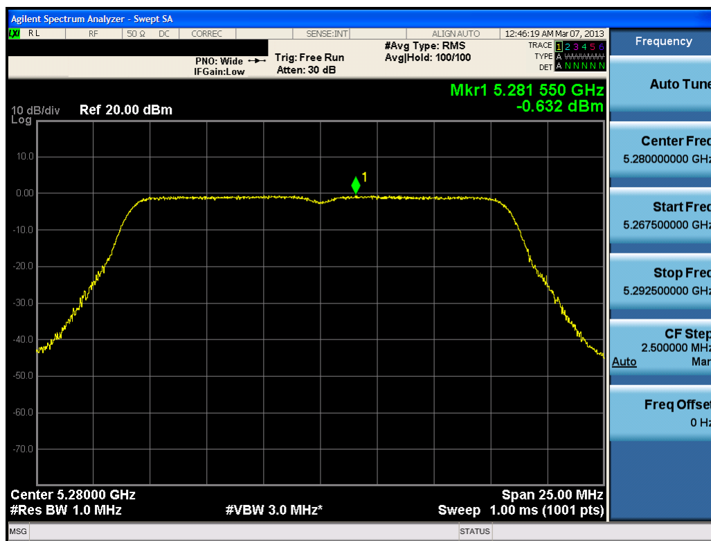
Plot 6-38. Peak Power Spectral Density Plot (802.11a (UNII Band 2) – Ch. 56)
