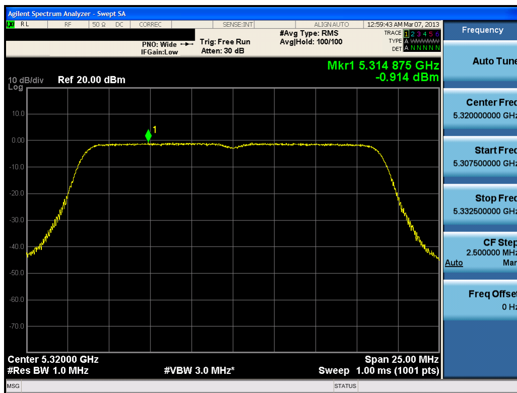
Plot 6-42. Peak Power Spectral Density Plot (20MHz BW 802.11n (UNII Band 2) – Ch. 64)
