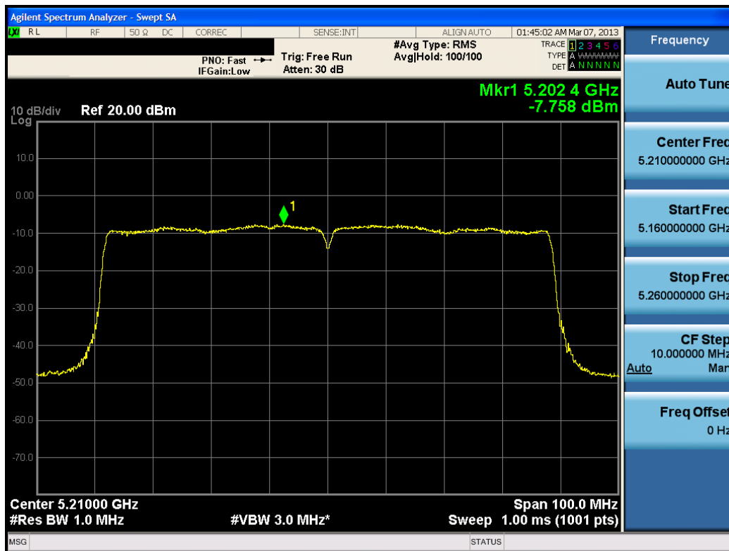
Plot 6-54. Peak Power Spectral Density Plot (80MHz BW 802.11ac (UNII Band 1) – Ch. 42)
