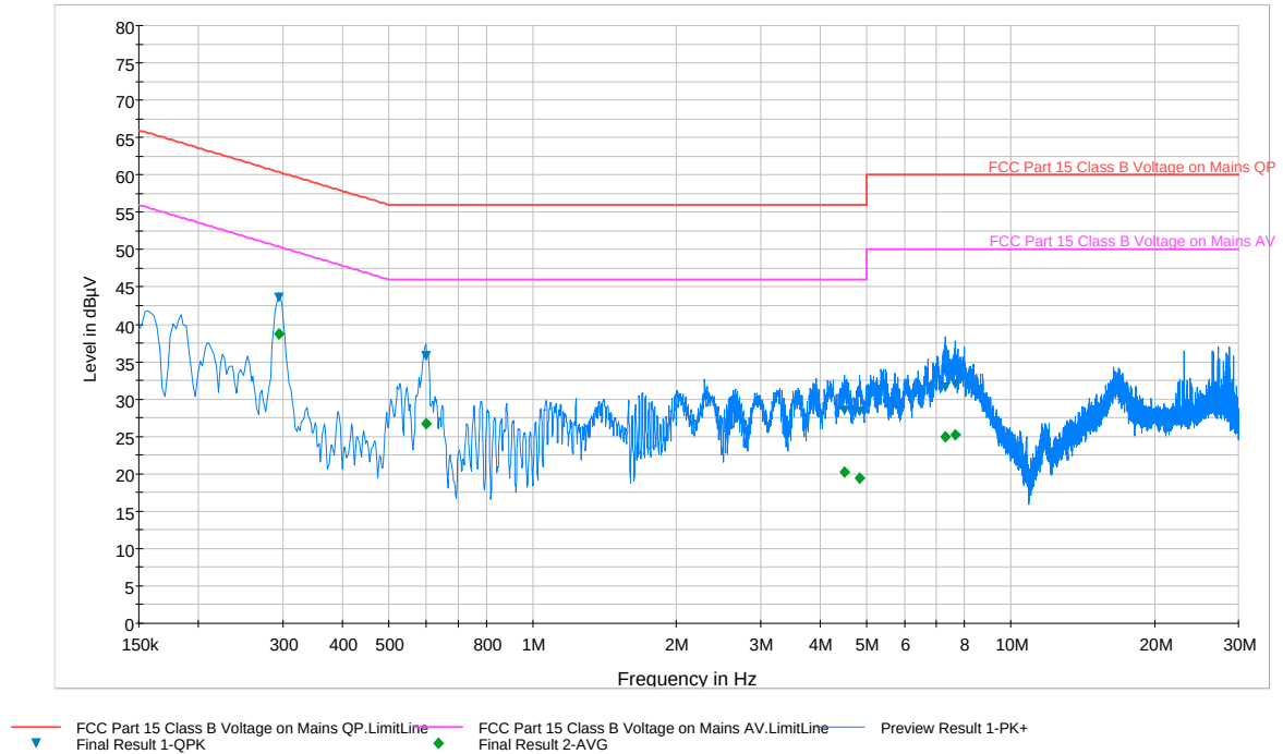
Plot 6-82. Line Conducted Plot with 802.11a UNII Band 1 (N)
