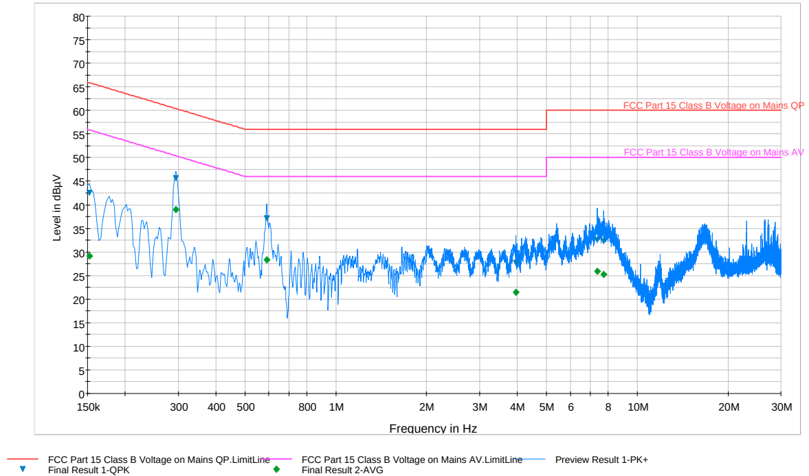
Plot 6-84. Line Conducted Plot with 802.11a UNII Band 2 (N)
