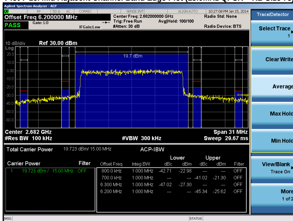
Plot 7-17. High Adjacent Channel Band Edge Plot (15.0MHz QPSK – RB Size 75)
