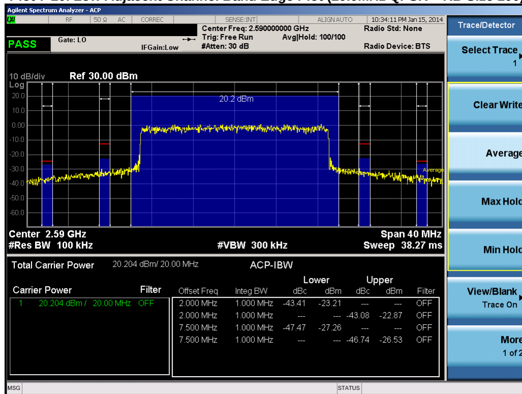
Plot 7-21. Mid Adjacent Channel Band Edge Plot (20.0MHz QPSK – RB Size 100)
