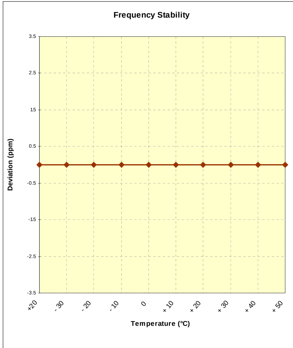
Figure 6-1. Frequency Stability Graph (Band 7)
