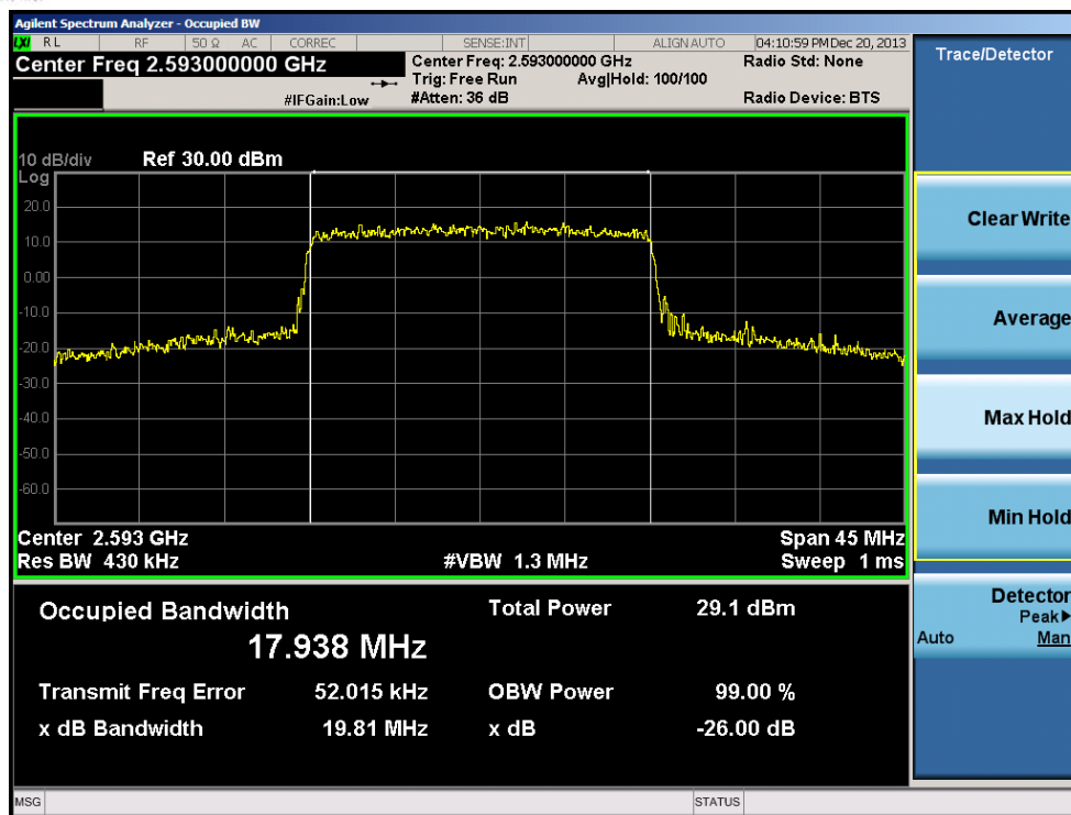
Plot 7-24. Occupied Bandwidth Plot (20.0MHz 16QAM – RB Size 100)
