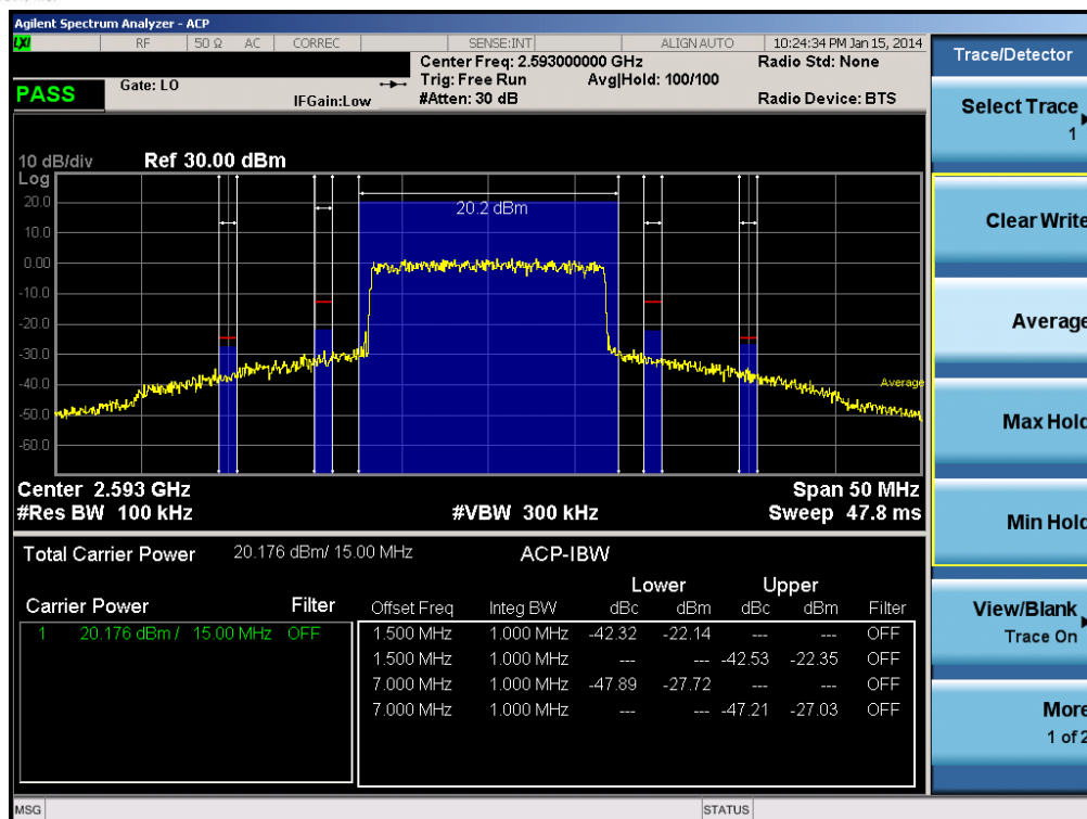
Plot 7-16. Mid Adjacent Channel Band Edge Plot (15.0MHz QPSK – RB Size 75)
