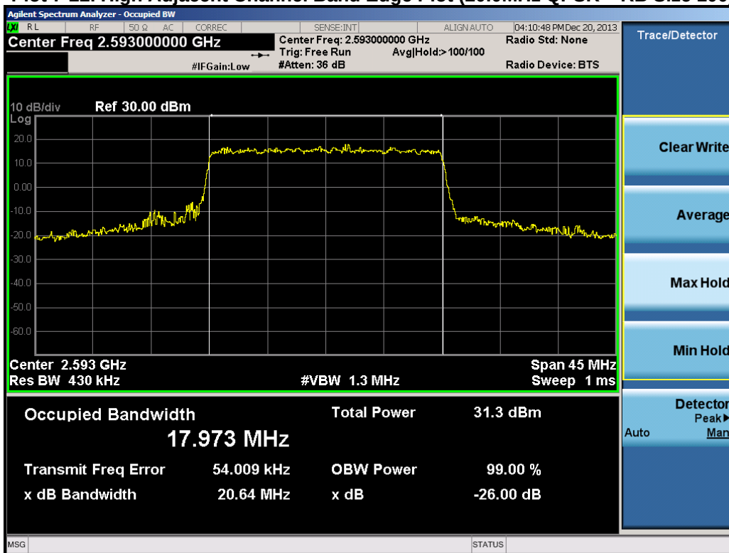
Plot 7-23. Occupied Bandwidth Plot (20.0MHz QPSK – RB Size 100)
