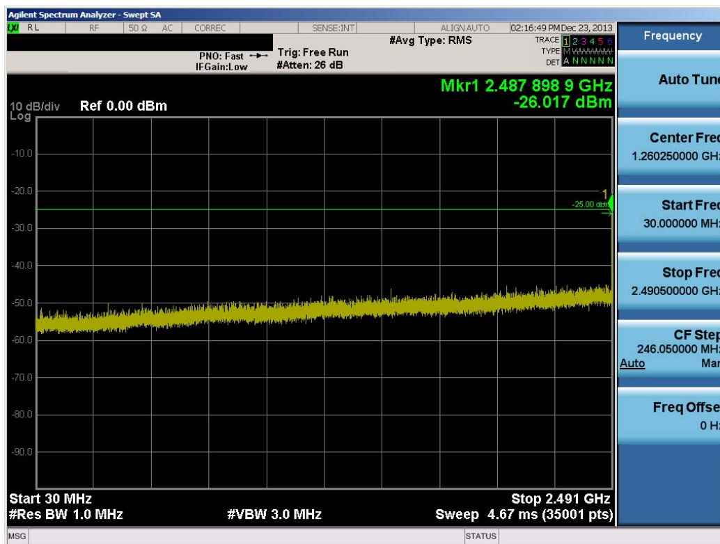
Plot 7-6. Conducted Spurious Plot (10.0MHz QPSK – RB Size 1, RB Offset 0– Low Channel)
