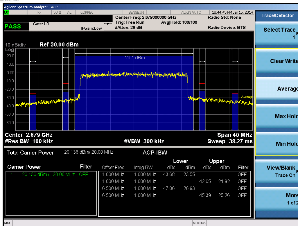
Plot 7-22. High Adjacent Channel Band Edge Plot (20.0MHz QPSK – RB Size 100)
