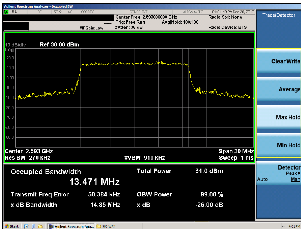
Plot 7-18. Occupied Bandwidth Plot (15.0MHz QPSK – RB Size 75)
