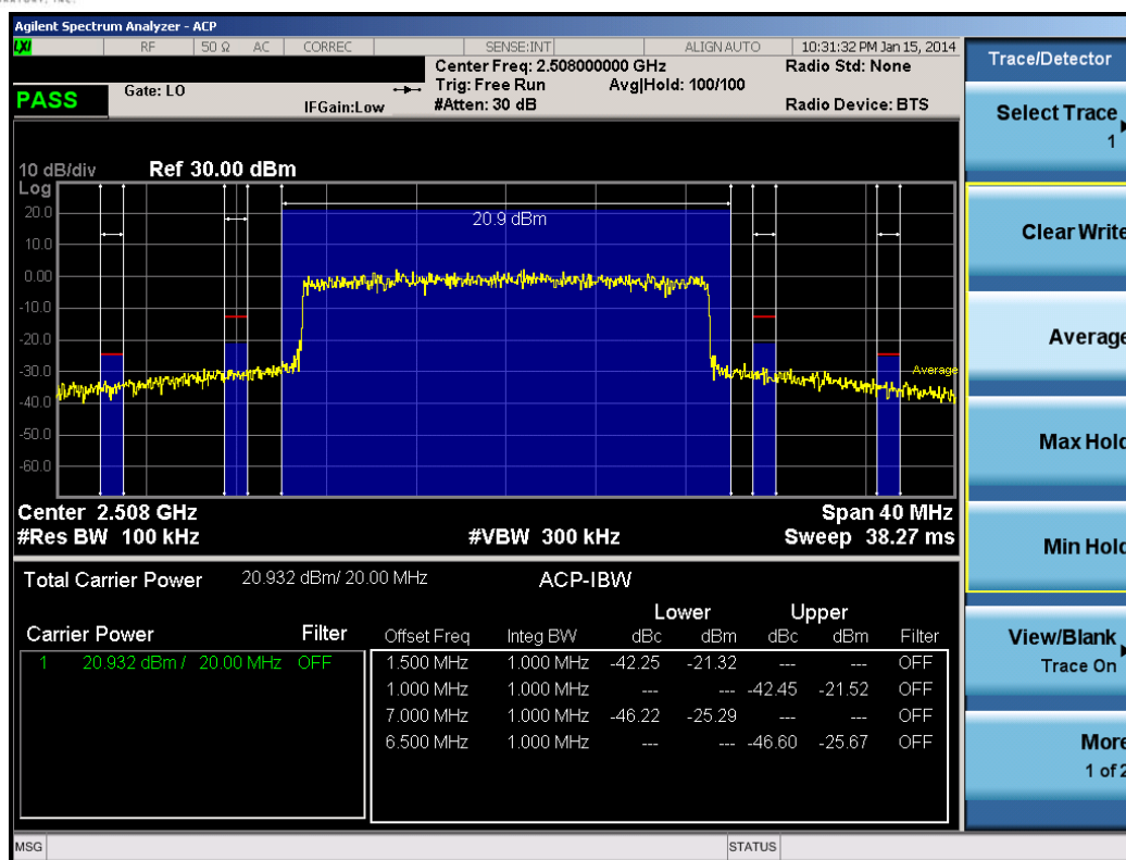
Plot 7-20. Low Adjacent Channel Band Edge Plot (20.0MHz QPSK – RB Size 100)
