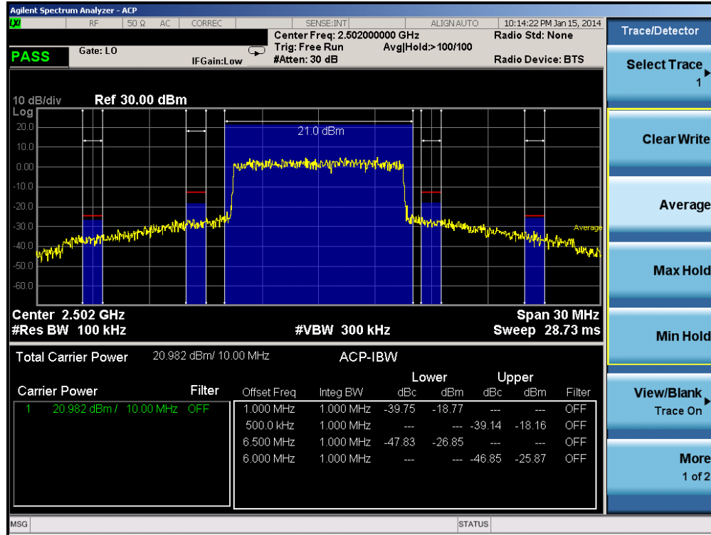
Plot 7-1. Low Adjacent Channel Band Edge Plot (10.0MHz QPSK – RB Size 50)
