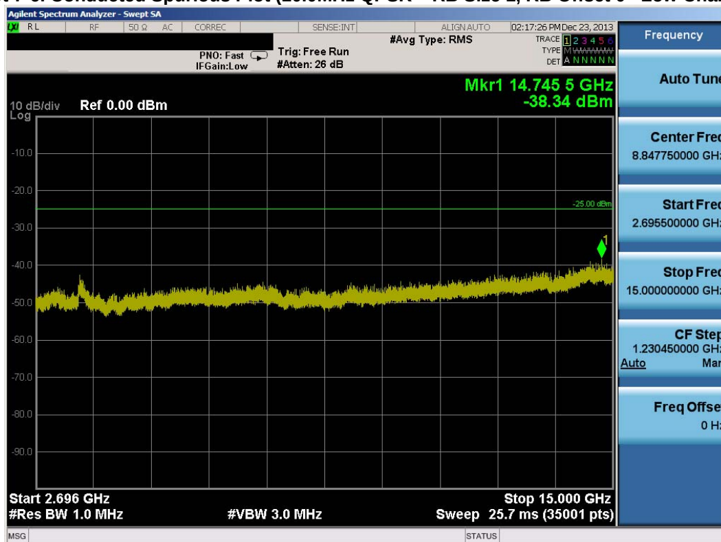
Plot 7-7. Conducted Spurious Plot (10.0MHz QPSK – RB Size 1, RB Offset 0 – Low Channel)
