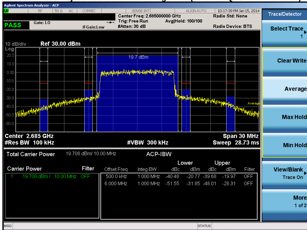
Plot 7-3. High Adjacent Channel Band Edge Plot (10.0MHz QPSK – RB Size 50)
