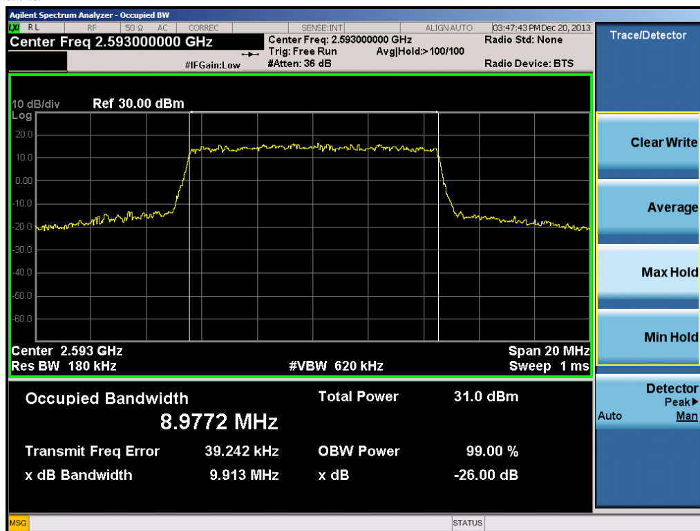
Plot 7-4. Occupied Bandwidth Plot (10.0MHz QPSK – RB Size 50)
