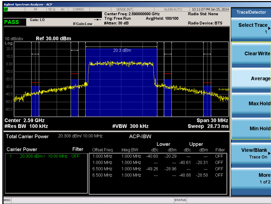
Plot 7-2. Mid Adjacent Channel Band Edge Plot (10.0MHz QPSK – RB Size 50)
