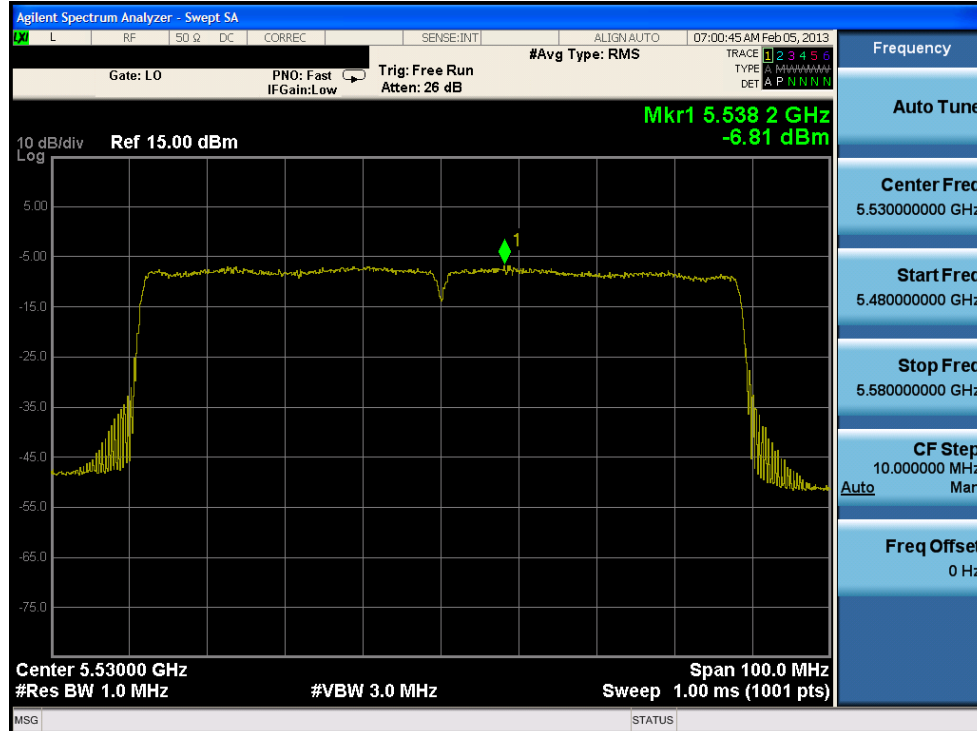
Plot 6-58. Peak Power Spectral Density Plot (80MHz BW 802.11ac (UNII Band 2C) – Ch. 106)
