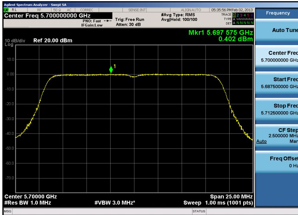
Plot 6-54. Peak Power Spectral Density Plot (20MHz BW 802.11n (UNII Band 2C) – Ch. 140)
