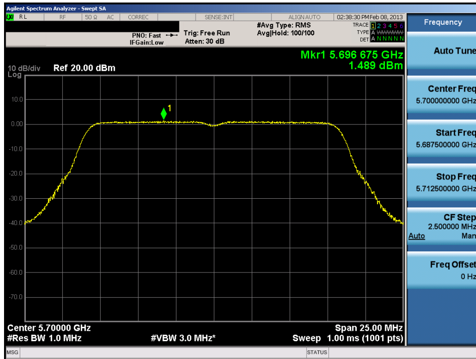
Plot 6-51. Peak Power Spectral Density Plot (802.11a (UNII Band 2C) – Ch. 140)
