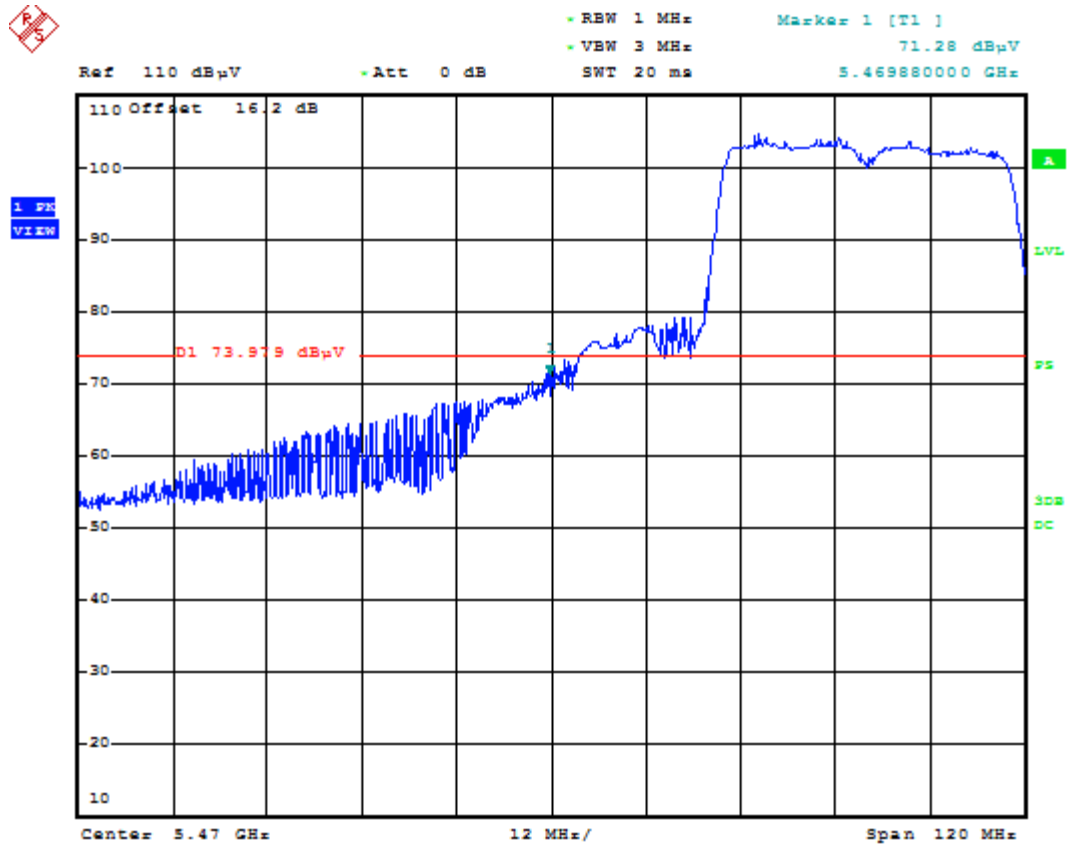
Plot 6-75. Radiated Restricted Lower Band Edge Plot (Peak – UNII Band 2C)
