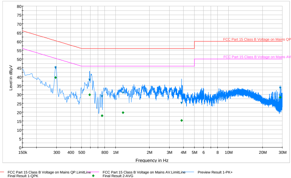
Plot 6-86. Line Conducted Plot with 802.11a UNII Band 2A (N)
