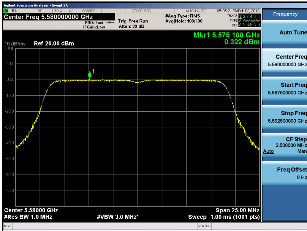
Plot 6-53. Peak Power Spectral Density Plot (20MHz BW 802.11n (UNII Band 2C) – Ch. 116)
