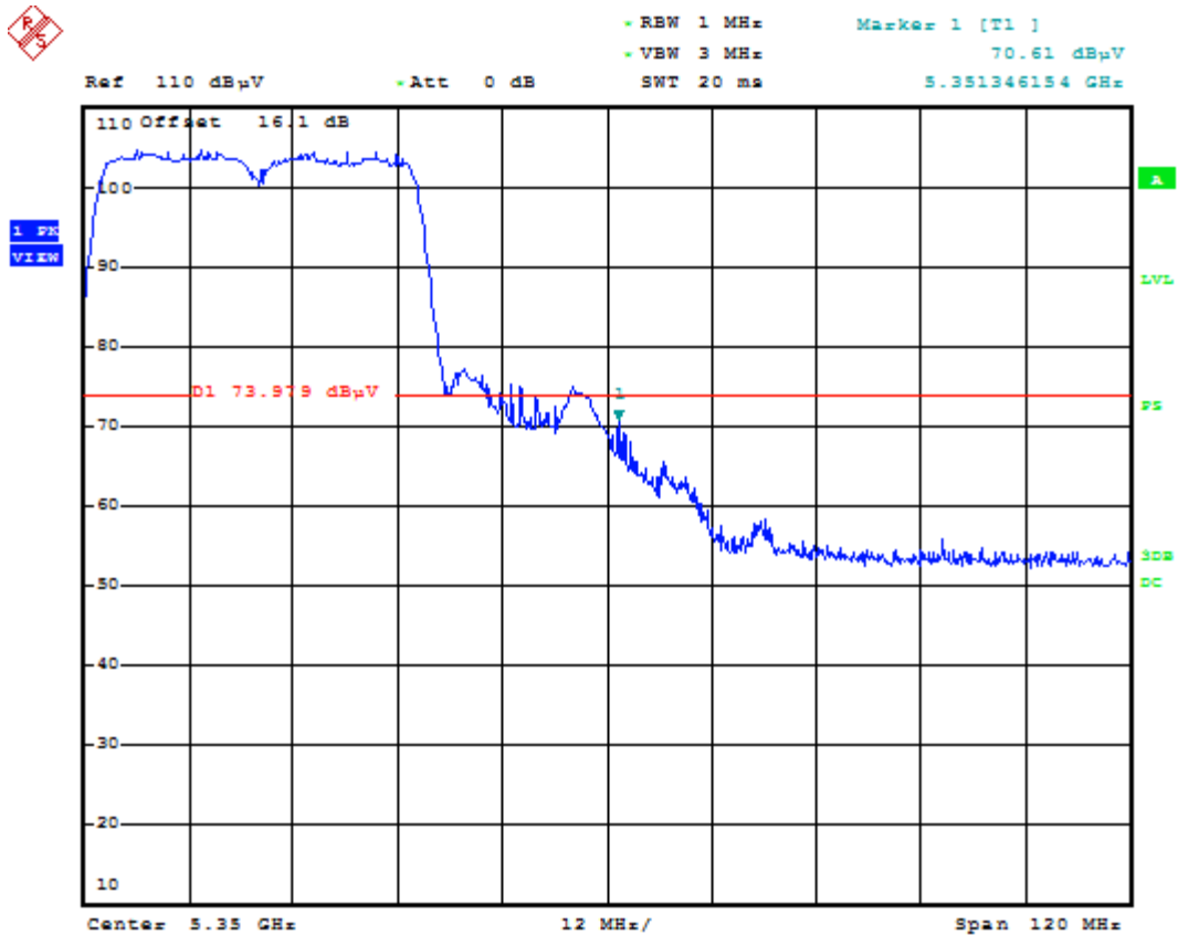
Plot 6-73. Radiated Restricted Upper Band Edge Plot (Peak - UNII Band 2A)
