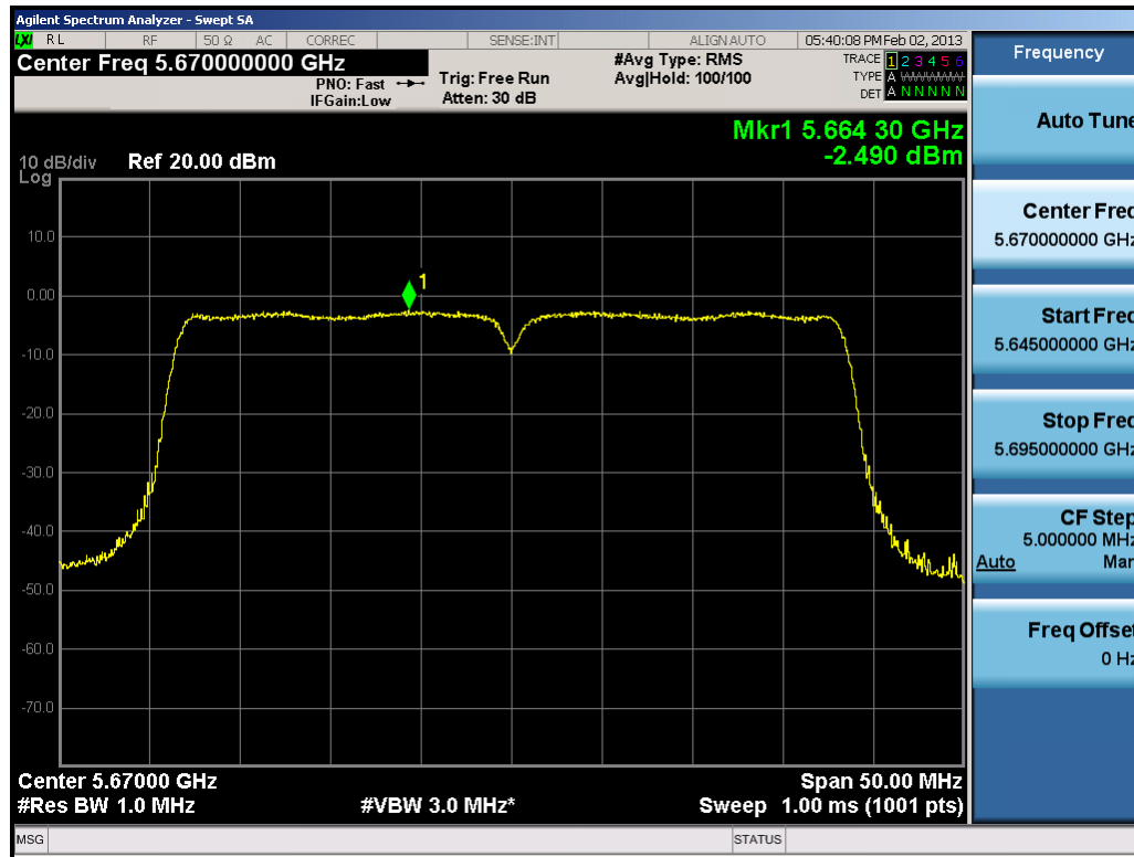
Plot 6-57. Peak Power Spectral Density Plot (40MHz BW 802.11n (UNII Band 2C) – Ch. 134)
