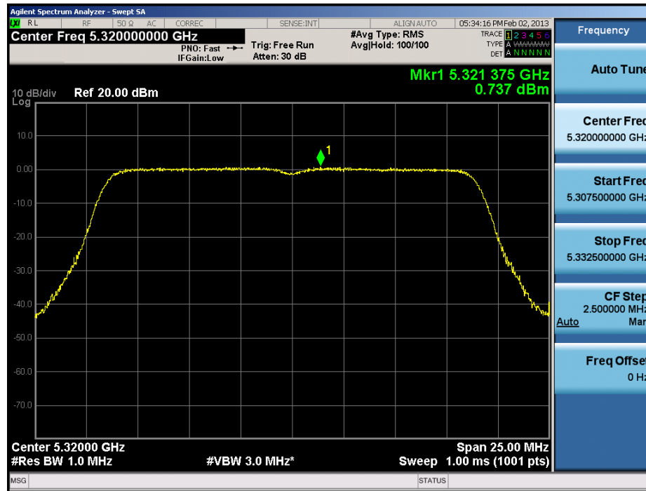
Plot 6-45. Peak Power Spectral Density Plot (20MHz BW 802.11n (UNII Band 2A) – Ch. 64)
