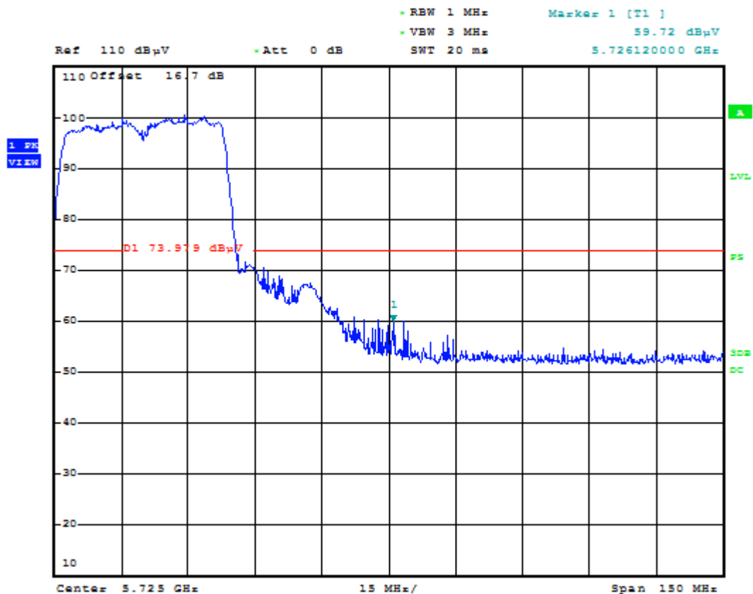
Plot 6-76. Radiated Upper Band Edge Plot (Peak – UNII Band 2C)
