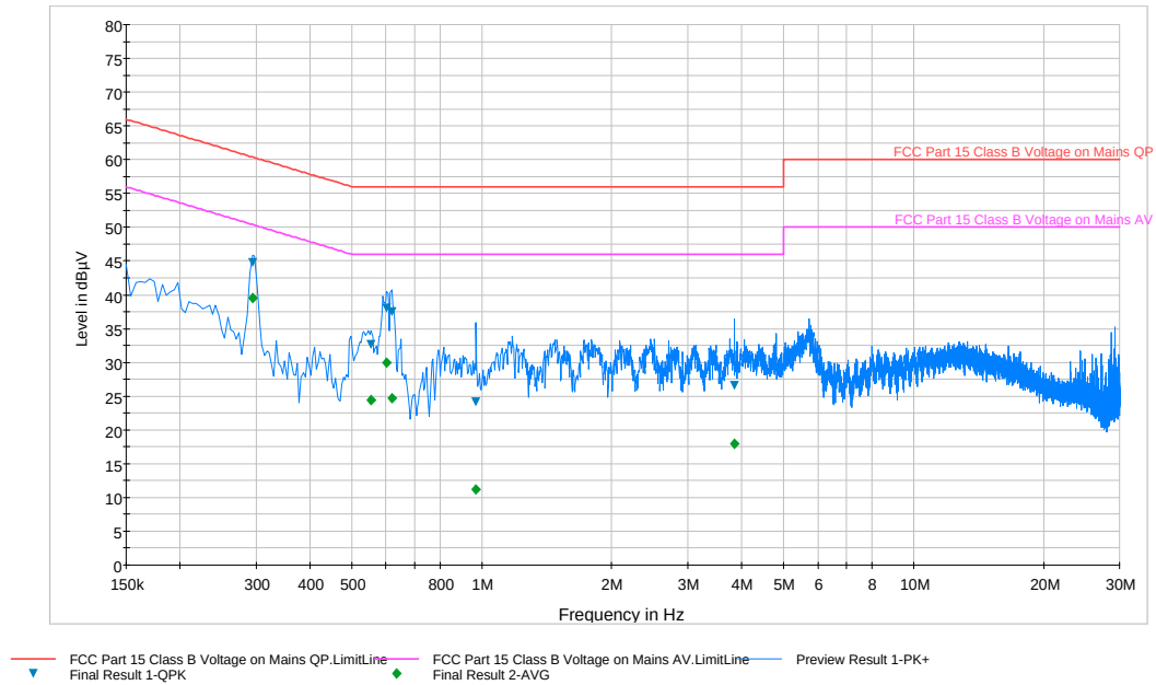
Plot 6-88. Line Conducted Plot with 802.11a UNII Band 2C (N)
