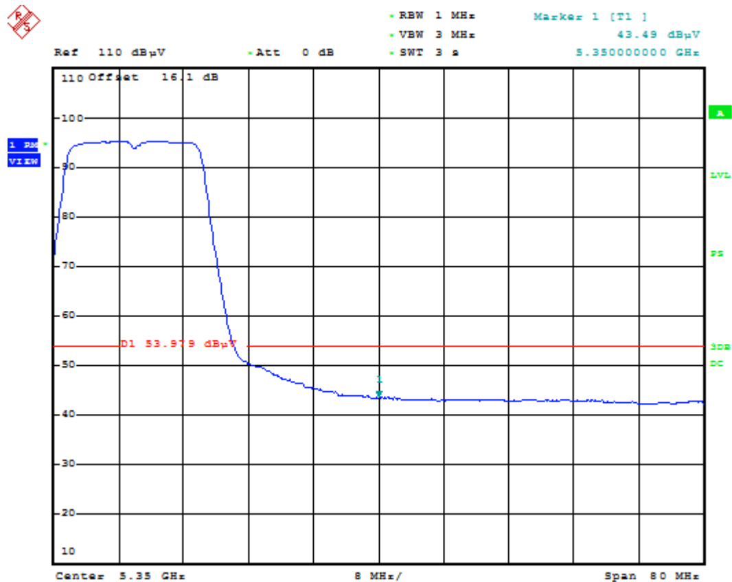
Plot 6-65. Radiated Restricted Upper Band Edge Plot (Average – UNII Band 2A)
