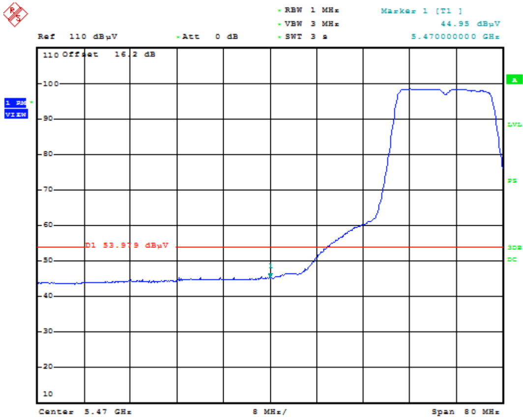
Plot 6-67. Radiated Restricted Lower Band Edge Plot (Average – UNII Band 2C)
