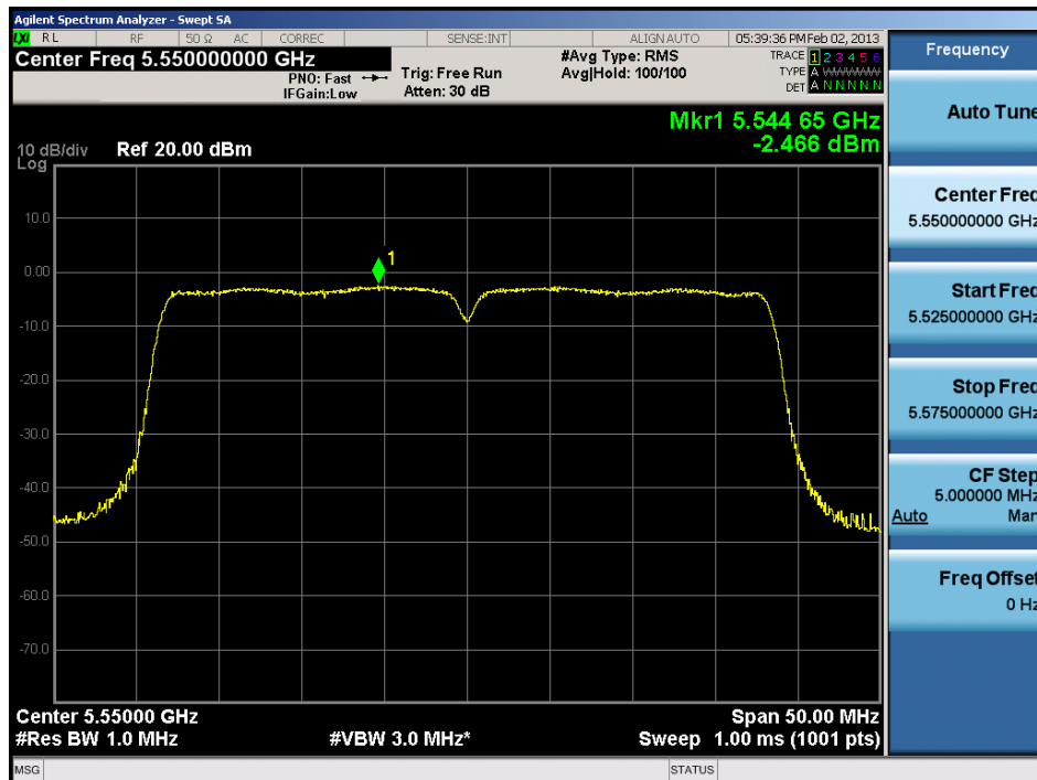
Plot 6-56. Peak Power Spectral Density Plot (40MHz BW 802.11n (UNII Band 2C) – Ch. 110)
