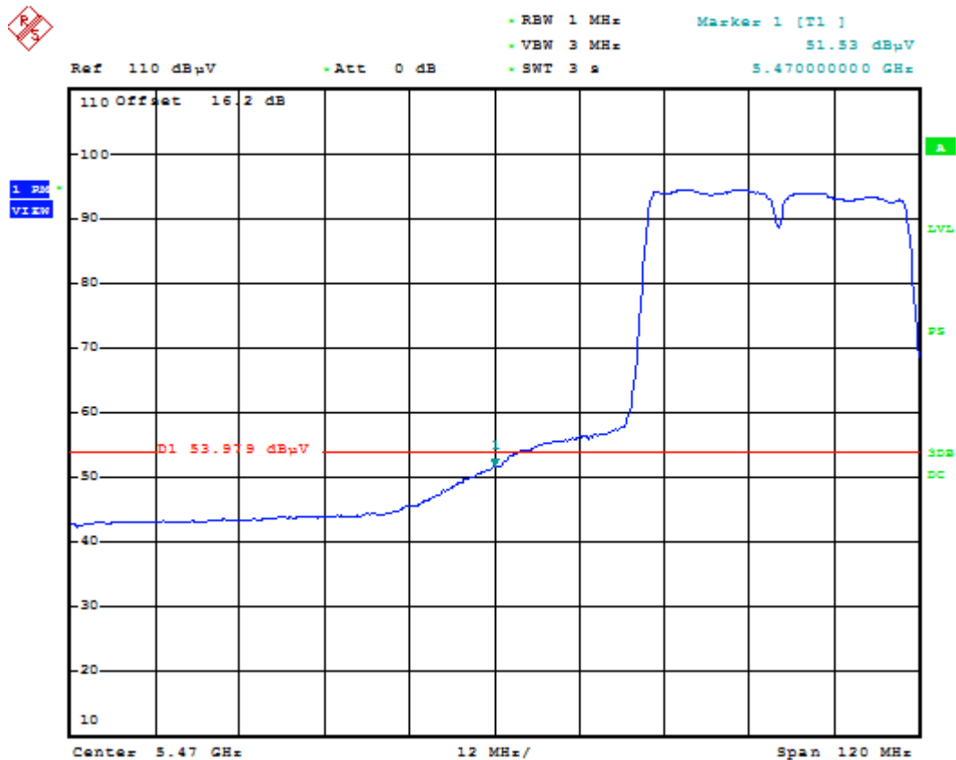
Plot 6-74. Radiated Restricted Lower Band Edge Plot (Average – UNII Band 2C)
