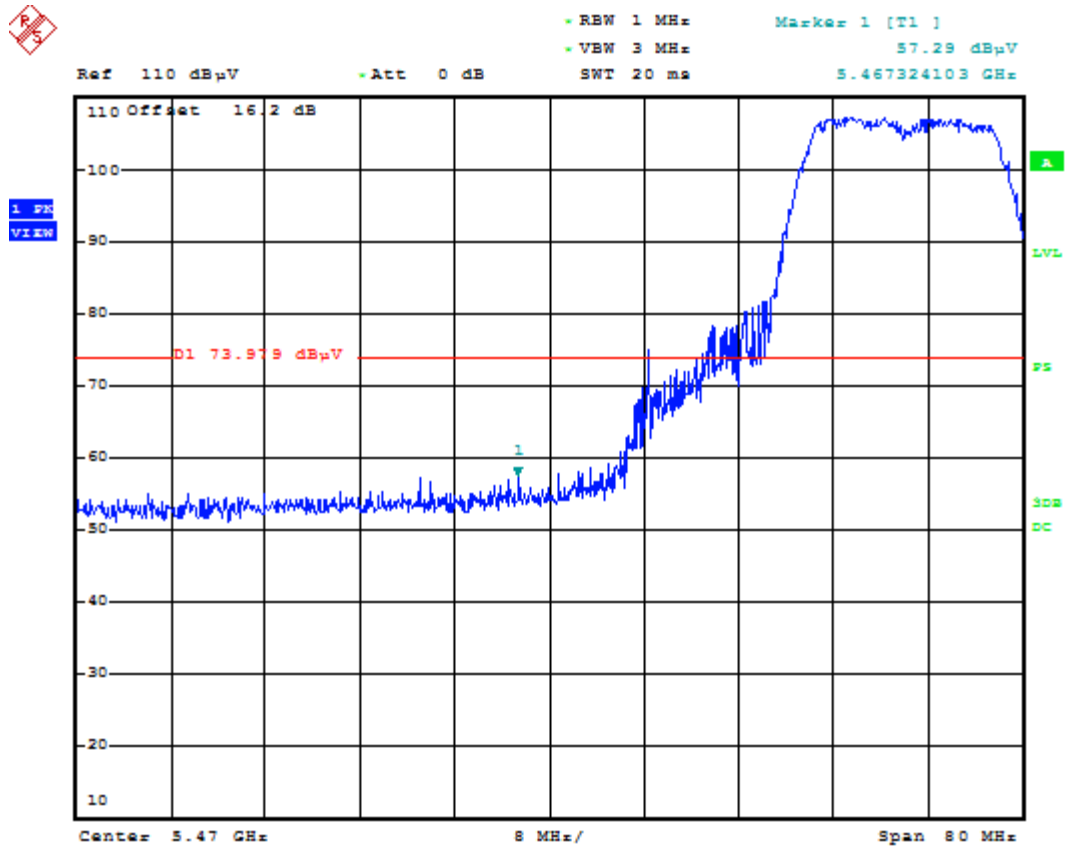
Plot 6-68. Radiated Restricted Lower Band Edge Plot (Peak – UNII Band 2C)
