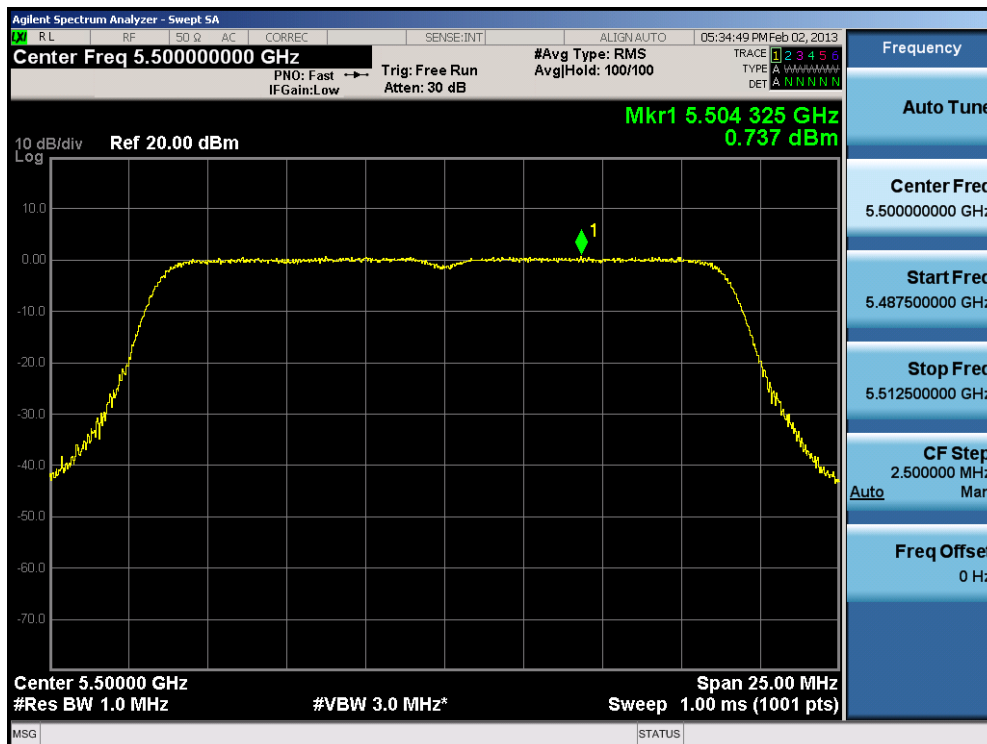
Plot 6-52. Peak Power Spectral Density Plot (20MHz BW 802.11n (UNII Band 2C) – Ch. 100)
