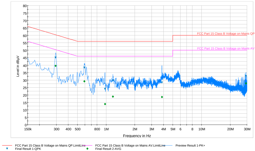
Plot 6-87. Line Conducted Plot with 802.11a UNII Band 2C (L1)
