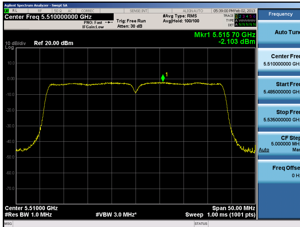
Plot 6-55. Peak Power Spectral Density Plot (40MHz BW 802.11n (UNII Band 2C) – Ch. 102)
