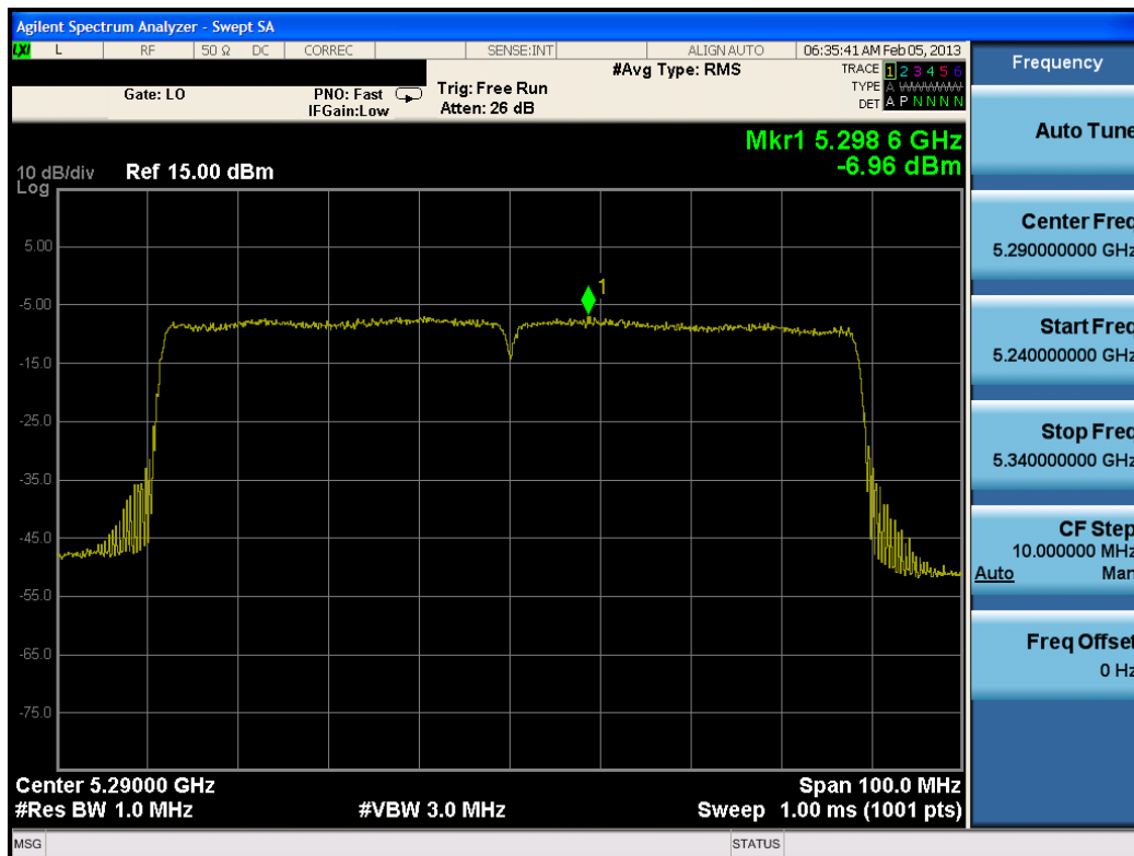
Plot 6-48. Peak Power Spectral Density Plot (80MHz BW 802.11ac (UNII Band 2A) – Ch. 58)
