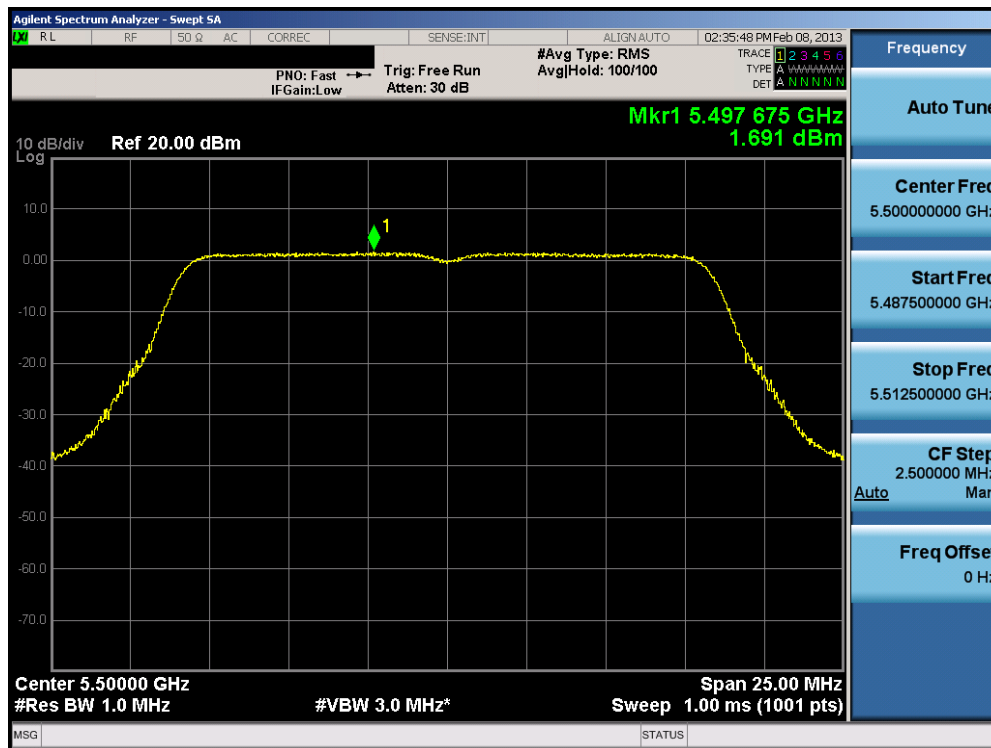
Plot 6-49. Peak Power Spectral Density Plot (802.11a (UNII Band 2C) – Ch. 100)
