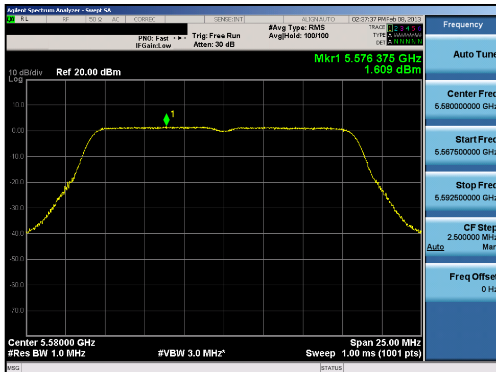
Plot 6-50. Peak Power Spectral Density Plot (802.11a (UNII Band 2C) – Ch. 116)
