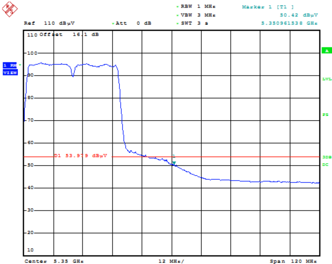
Plot 6-72. Radiated Restricted Upper Band Edge Plot (Average – UNII Band 2A)
