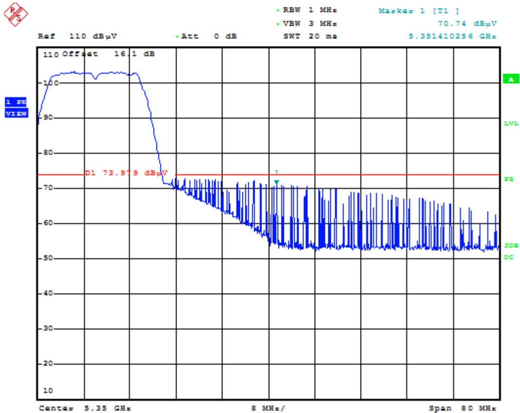
Plot 6-66. Radiated Restricted Upper Band Edge Plot (Peak – UNII Band 2A)
