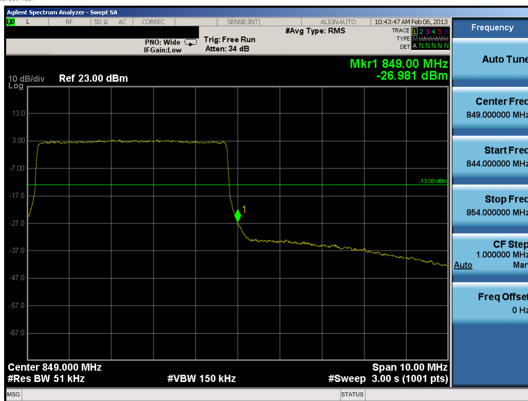
Plot 7-14. Upper Band Edge Plot (5.0MHz QPSK – RB Size 25)
