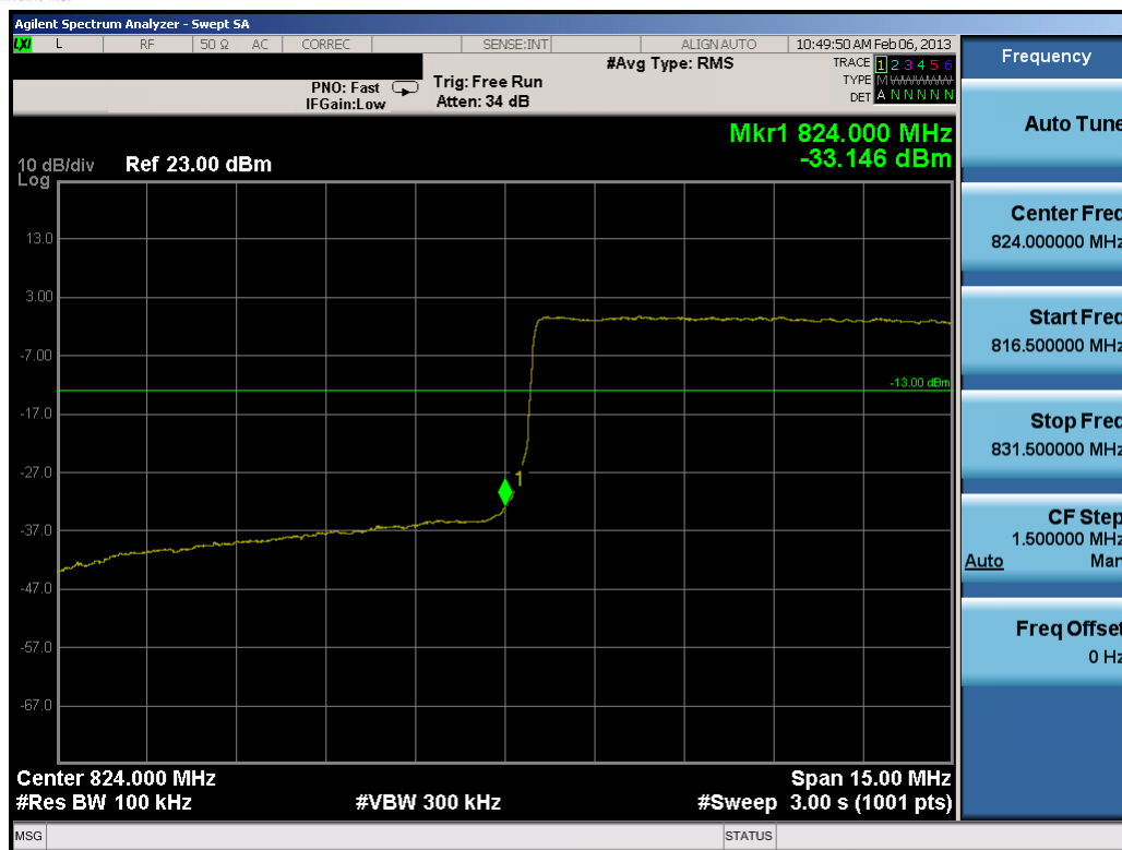
Plot 7-16. Lower Band Edge Plot (10.0MHz QPSK – RB Size 50)
