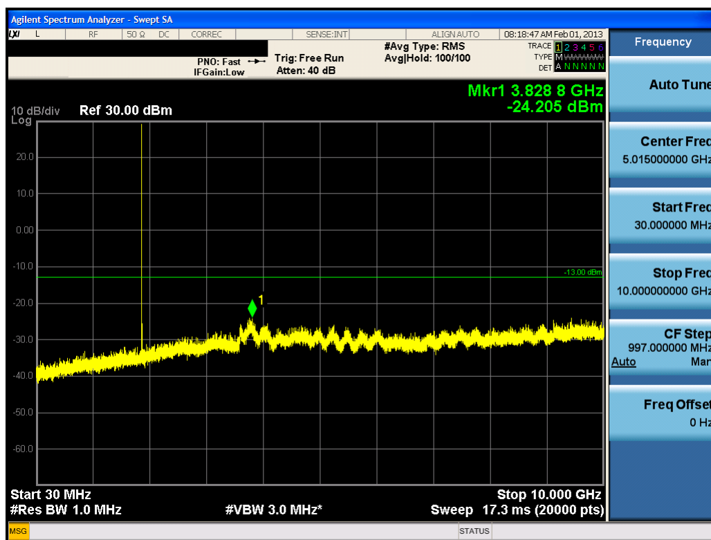
Plot 7-14. Conducted Spurious Plot (PCS GSM Mode – Ch. 661)
