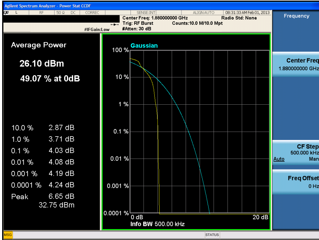
Plot 7-19. Peak-Average Ratio Plot (PCS EDGE Mode – Ch. 661)
