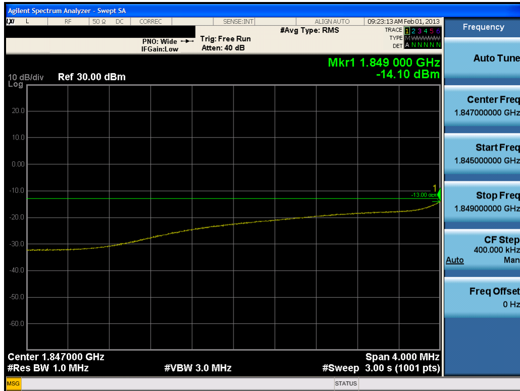
Plot 7-37. 4MHz Span Plot (PCS WCDMA Mode – Ch. 9262)
