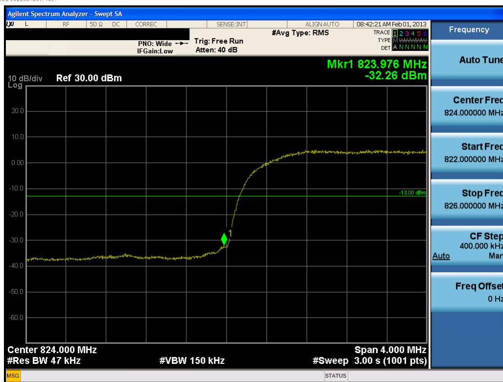
Plot 7-25. Band Edge Plot (Cellular WCDMA Mode – Ch. 4132)
