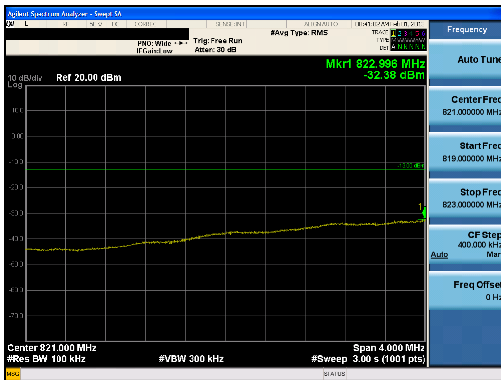
Plot 7-26. 4MHz Span Plot (Cellular WCDMA Mode – Ch. 4132)
