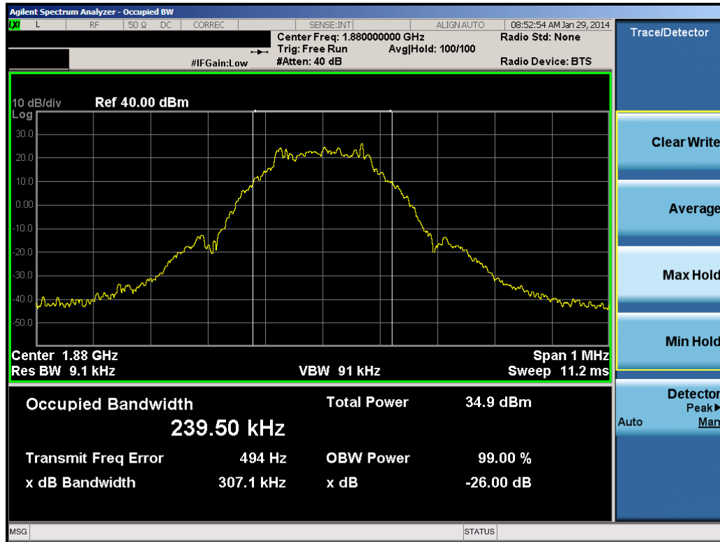
Plot 7-17. Occupied Bandwidth Plot (PCS EDGE Mode – Ch. 661)
