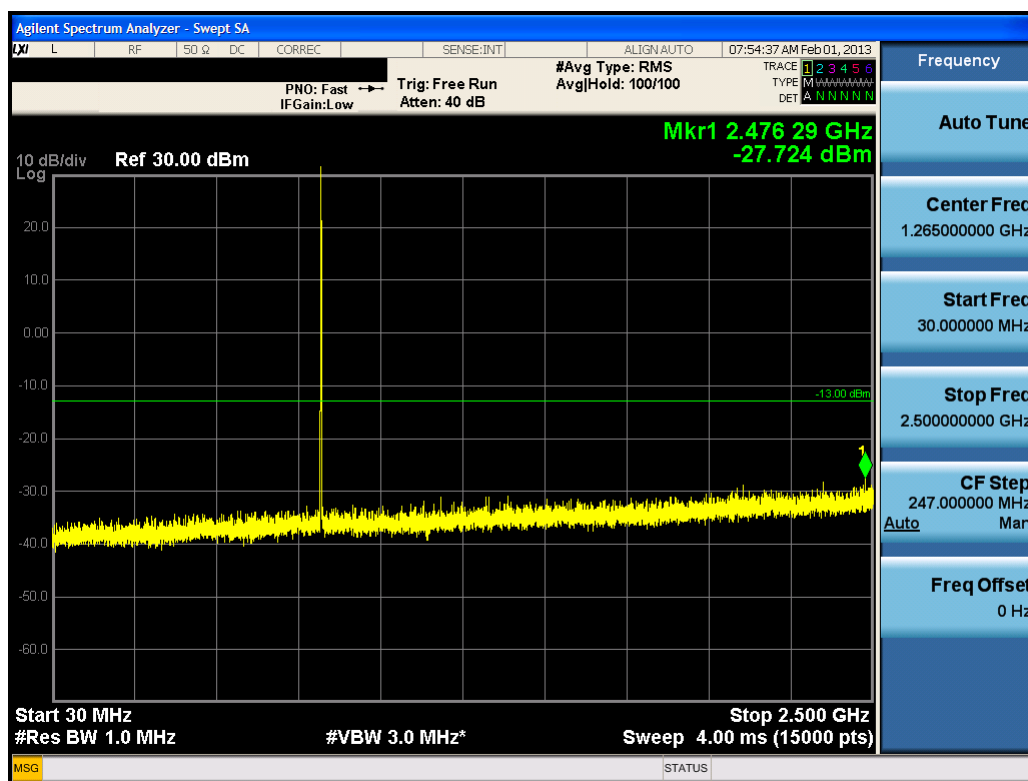
Plot 7-4. Conducted Spurious Plot (Cellular GSM Mode - Ch. 190)
