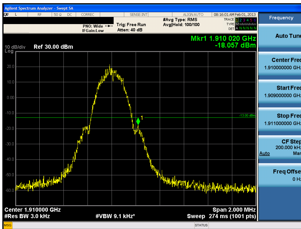
Plot 7-22. Band Edge Plot (PCS GSM Mode – Ch. 810)
