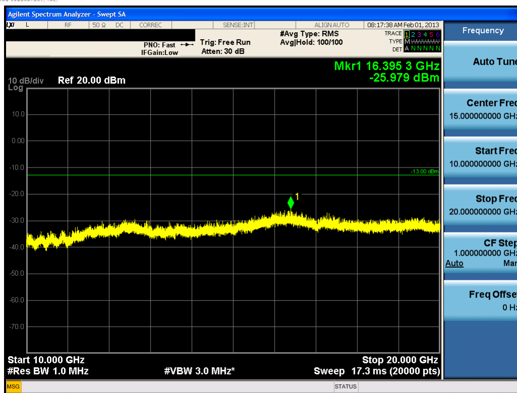
Plot 7-21. Conducted Spurious Plot (PCS GSM Mode – Ch. 810)
