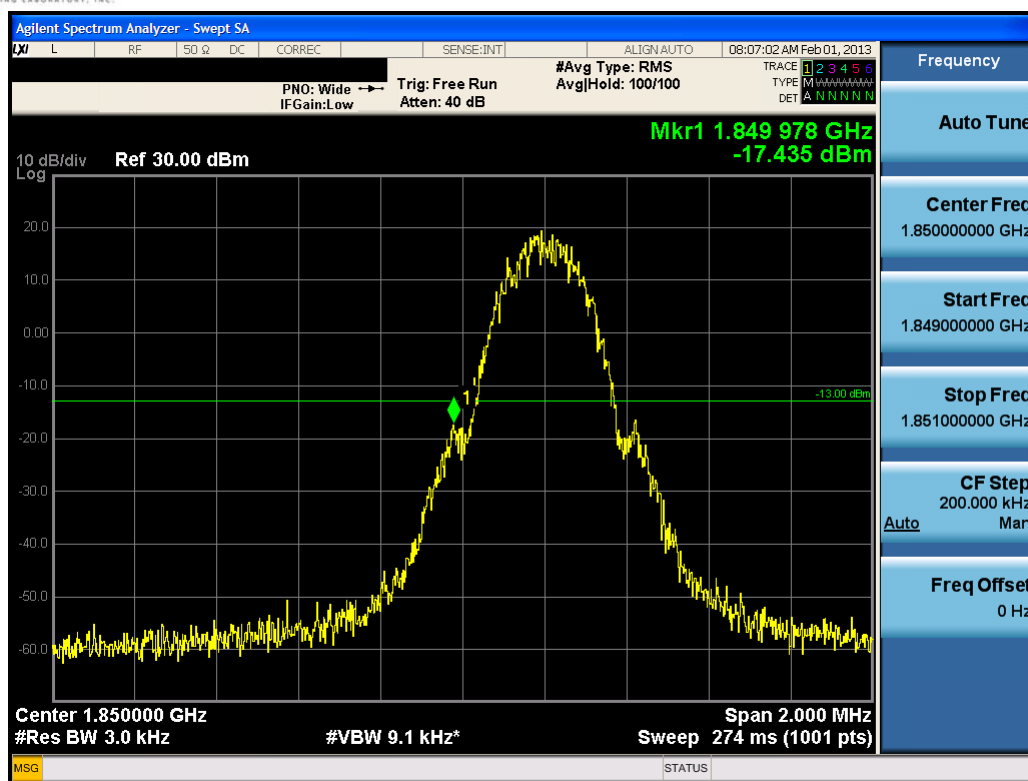
Plot 7-13. Band Edge Plot (PCS GSM Mode – Ch. 512)
