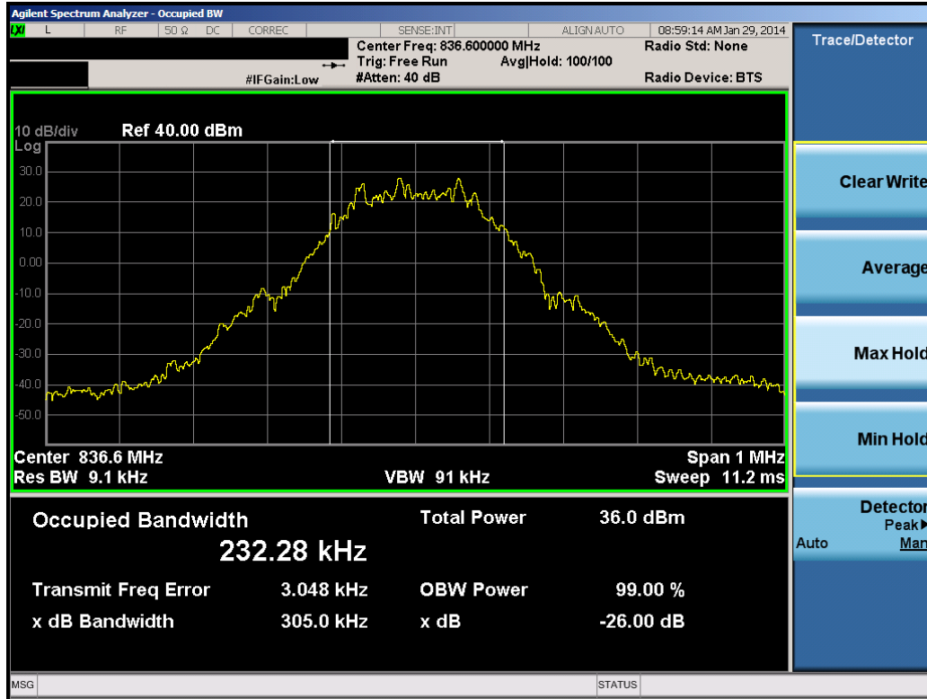
Plot 7-7. Occupied Bandwidth Plot (EDGE850 Mode – Ch. 190)
