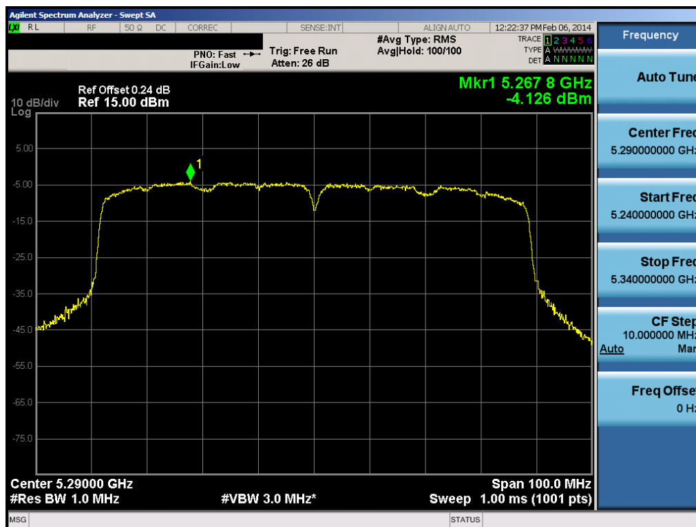
Plot 6-50. Peak Power Spectral Density Plot (80MHz BW 802.11ac (UNII Band 2A) – Ch. 58)
