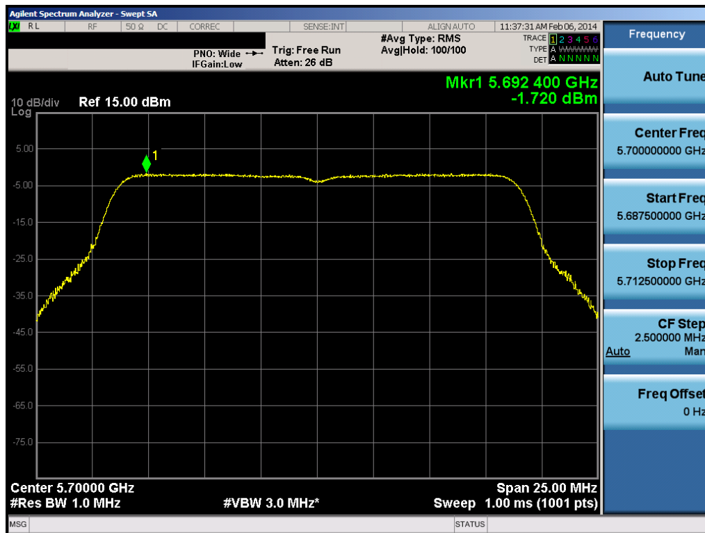
Plot 6-56. Peak Power Spectral Density Plot (20MHz BW 802.11n (UNII Band 2C) – Ch. 140)
