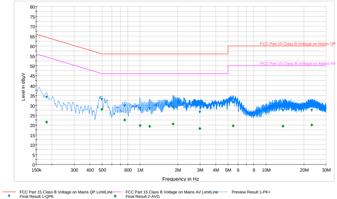
Plot 6-89. Line Conducted Plot with 802.11a UNII Band 2C (L1)
