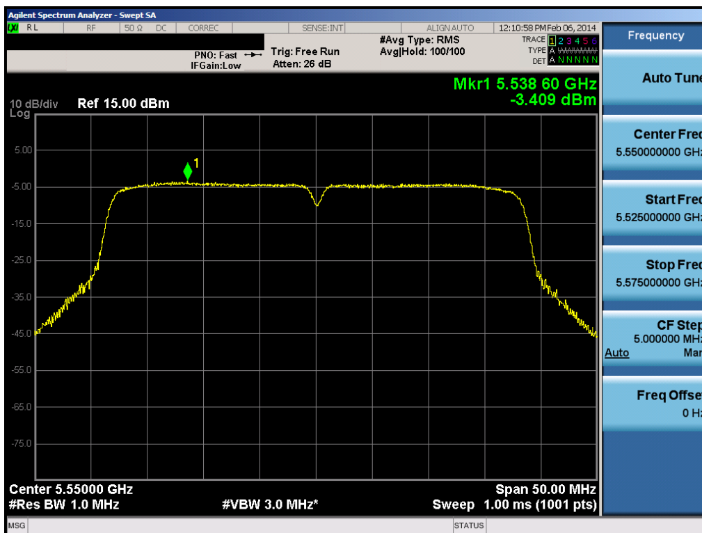
Plot 6-58. Peak Power Spectral Density Plot (40MHz BW 802.11n (UNII Band 2C) – Ch. 110)
