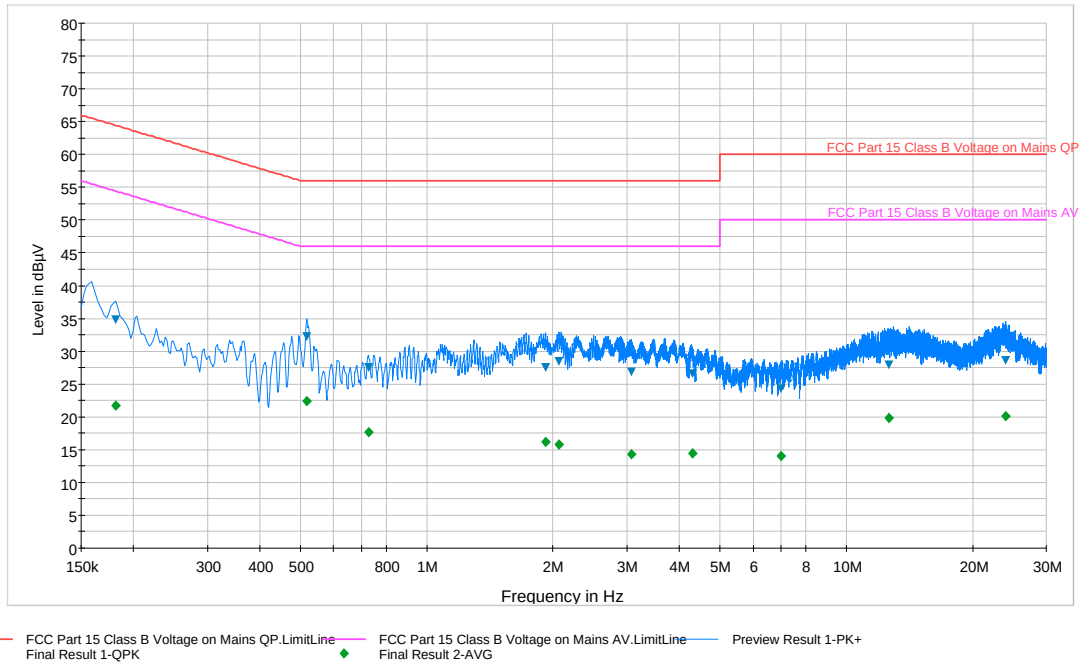
Plot 6-90. Line Conducted Plot with 802.11a UNII Band 2C (N)
