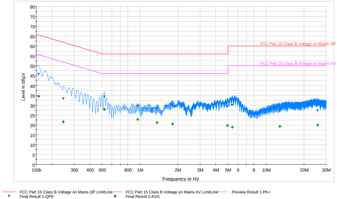
Plot 6-87. Line Conducted Plot with 802.11a UNII Band 2A (L1)
