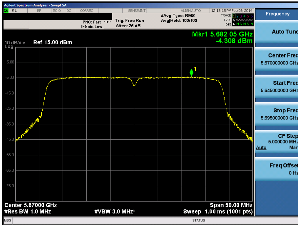
Plot 6-59. Peak Power Spectral Density Plot (40MHz BW 802.11n (UNII Band 2C) – Ch. 134)
