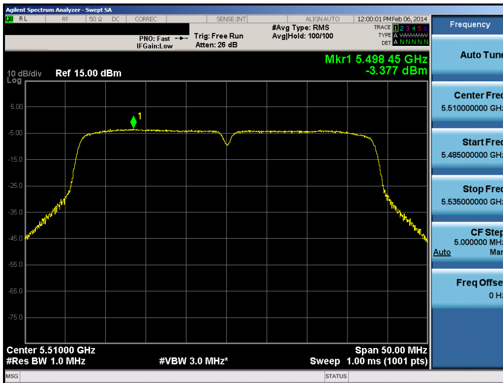
Plot 6-57. Peak Power Spectral Density Plot (40MHz BW 802.11n (UNII Band 2C) – Ch. 102)
