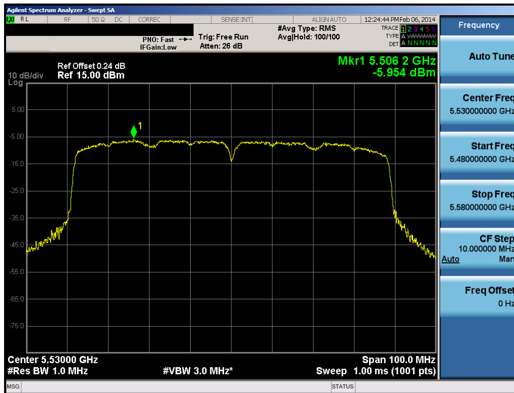
Plot 6-60. Peak Power Spectral Density Plot (80MHz BW 802.11ac (UNII Band 2C) – Ch. 106)
