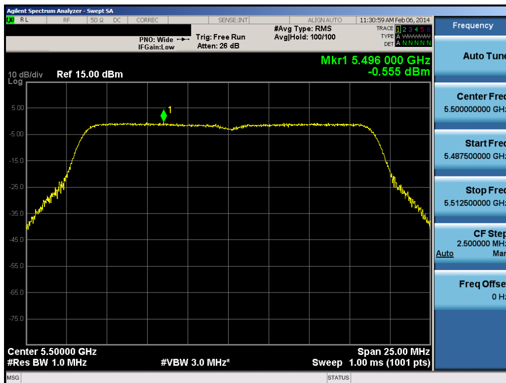
Plot 6-54. Peak Power Spectral Density Plot (20MHz BW 802.11n (UNII Band 2C) – Ch. 100)
