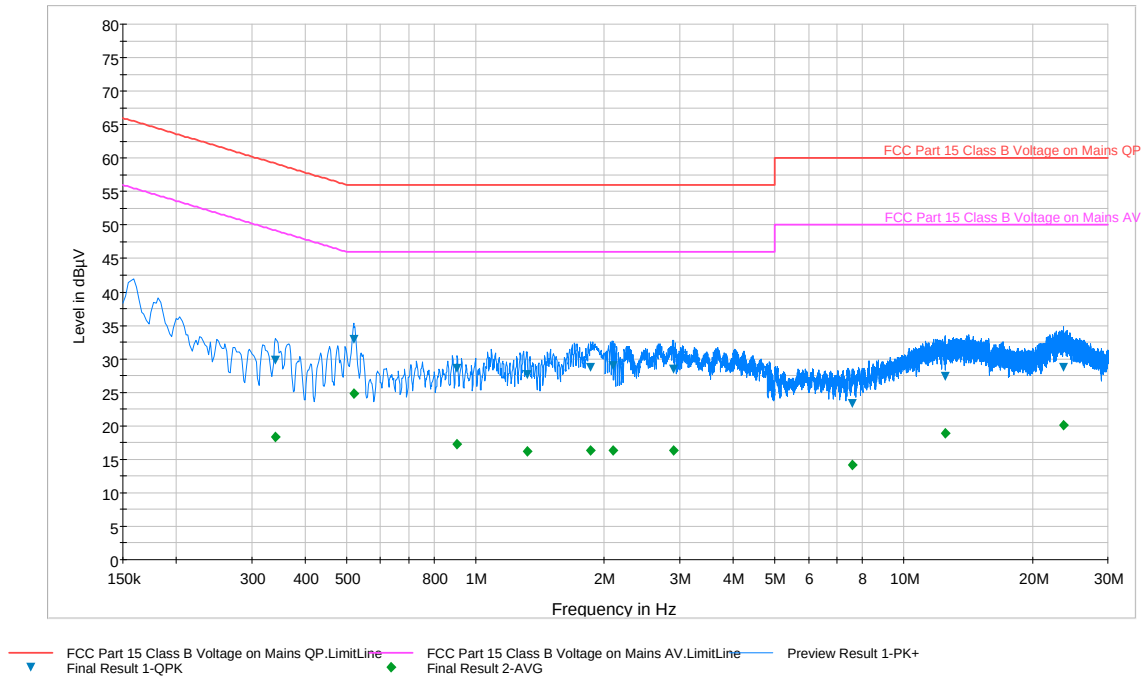
Plot 6-88. Line Conducted Plot with 802.11a UNII Band 2A (N)
