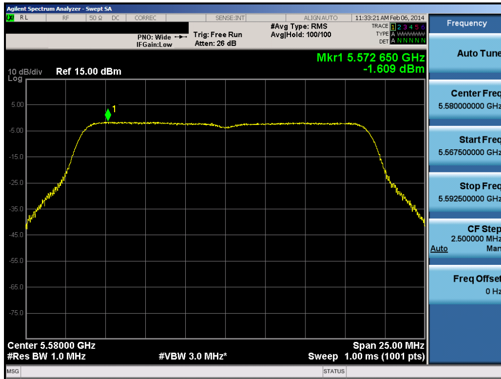
Plot 6-55. Peak Power Spectral Density Plot (20MHz BW 802.11n (UNII Band 2C) – Ch. 116)
