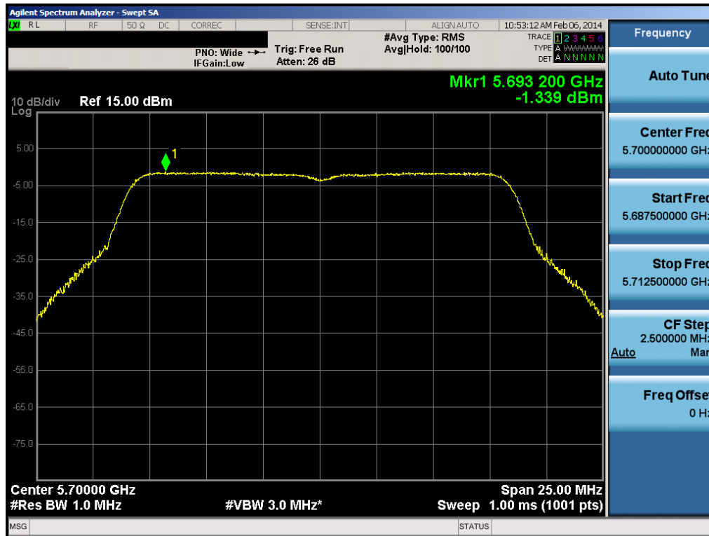
Plot 6-53. Peak Power Spectral Density Plot (802.11a (UNII Band 2C) – Ch. 140)
