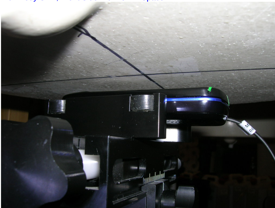
10. Body SAR, Front Side with 15mm Space
