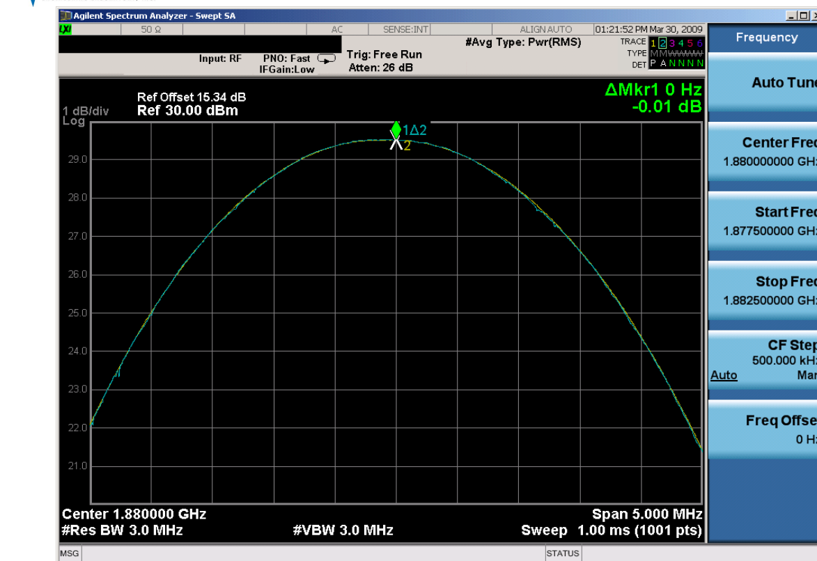
Plot 7-17. Peak-Average Ratio Plot (PCS GSM Mode – Ch. 661)
