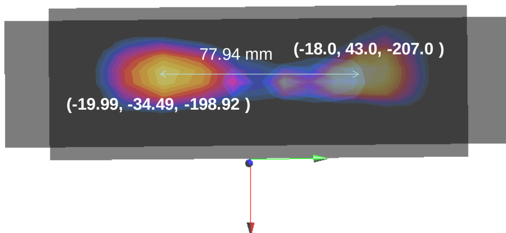
Figure 11-5 Peak SAR Locations of 5 GHz WLAN and UMTS 1900
