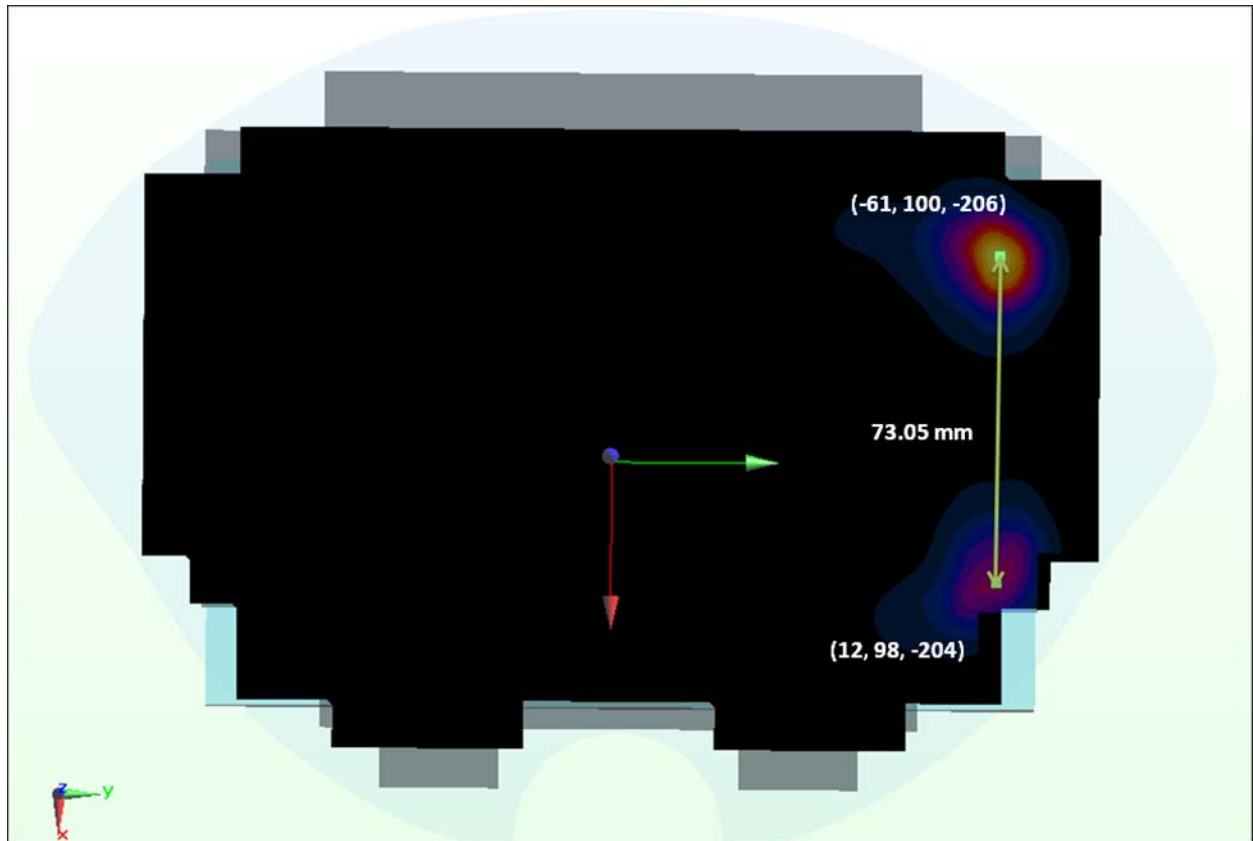
Figure 11-8 Peak SAR Locations of 2.4 GHz WLAN and UMTS 1900
