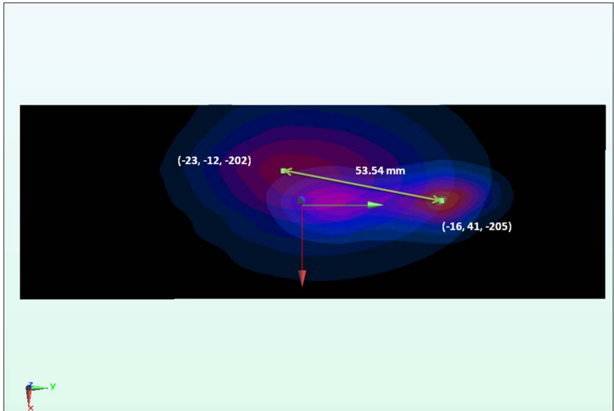
Figure 11-9 Peak SAR Locations of 2.4 GHz WLAN and GPRS 850
