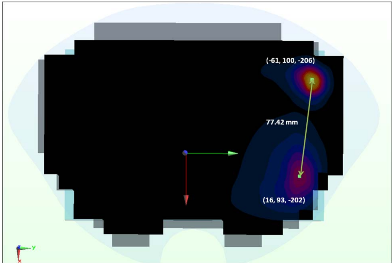
Figure 11-5 Peak SAR Locations of 2.4 GHz WLAN and GPRS 850
