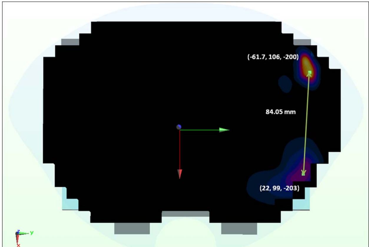
Figure 11-16 Peak SAR Locations of 5 GHz WLAN and GPRS 1900
