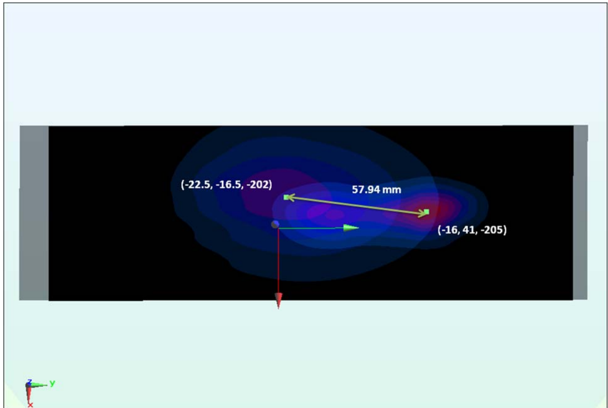
Figure 11-10 Peak SAR Locations of 2.4 GHz WLAN and UMTS 850
