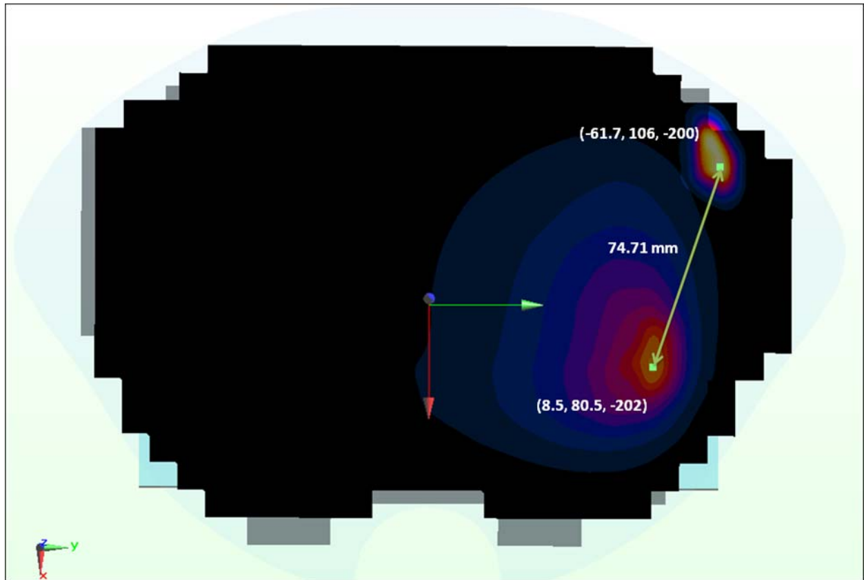
Figure 11-14 Peak SAR Locations of 5 GHz WLAN and GPRS 850
