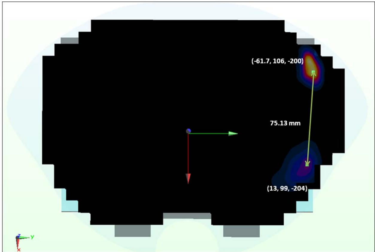
Figure 11-20 Peak SAR Locations of 5 GHz WLAN and GPRS 1900
