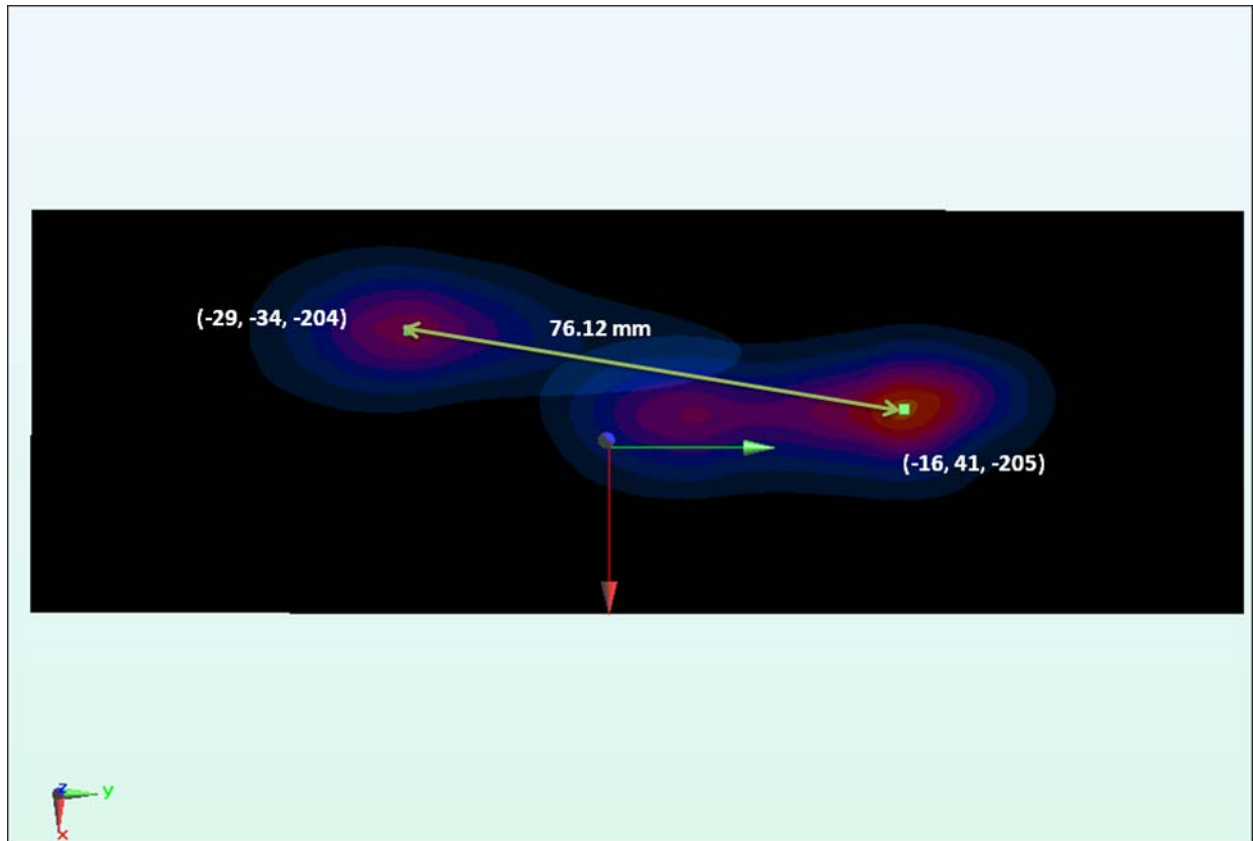
Figure 11-13 Peak SAR Locations of 2.4 GHz WLAN and UMTS 1900
