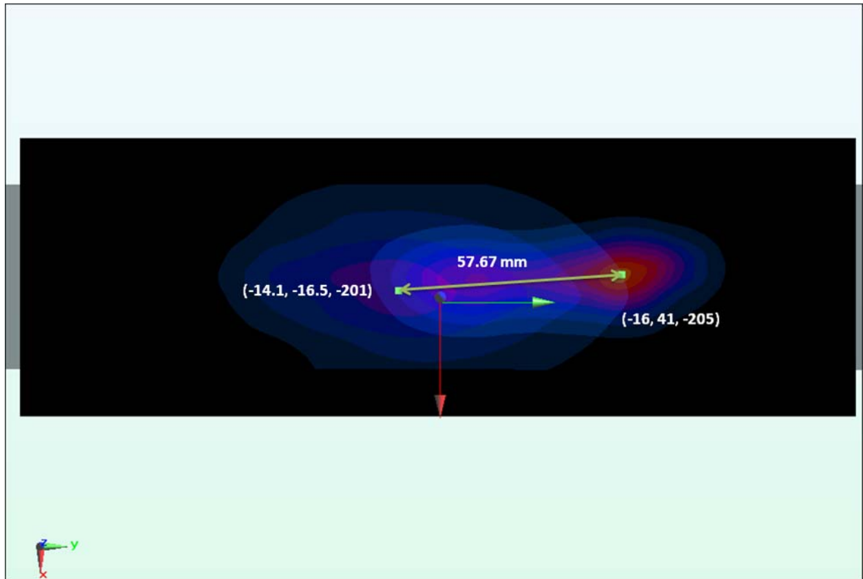
Figure 11-12 Peak SAR Locations of 2.4 GHz WLAN and GPRS 850
