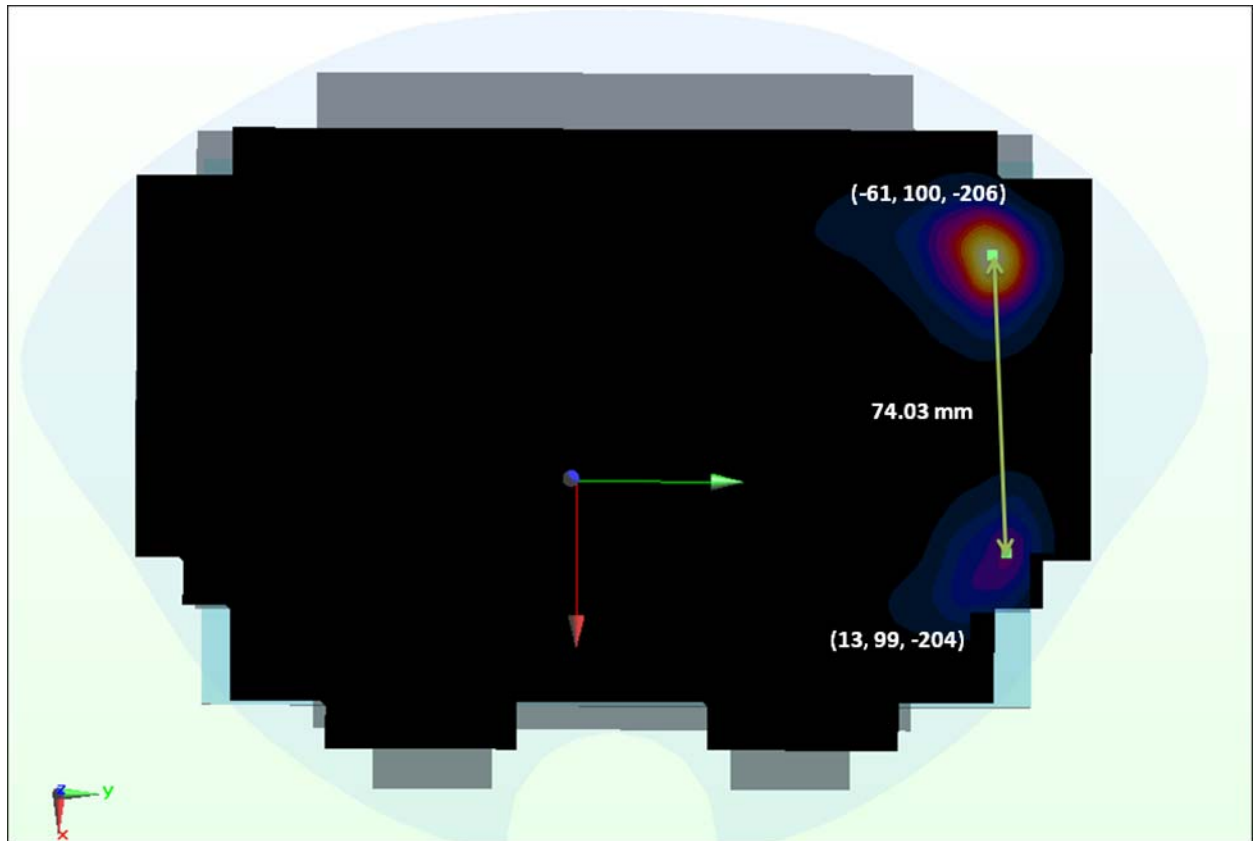
Figure 11-7 Peak SAR Locations of 2.4 GHz WLAN and GPRS 1900
