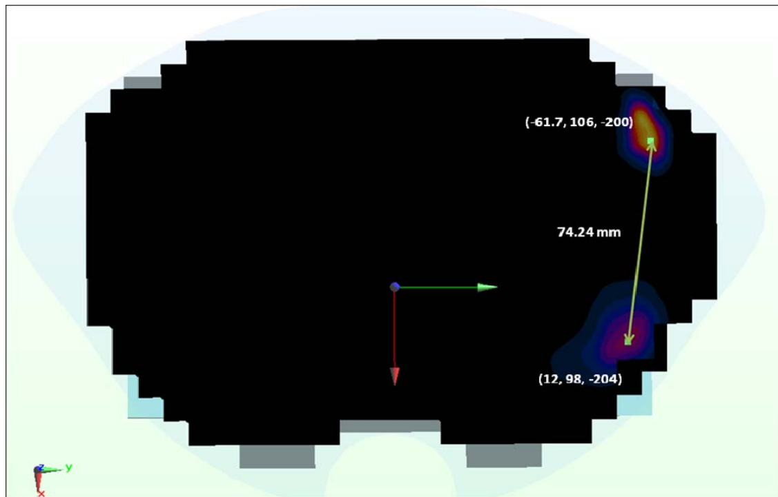
Figure 11-21 Peak SAR Locations of 5 GHz WLAN and UMTS 1900
