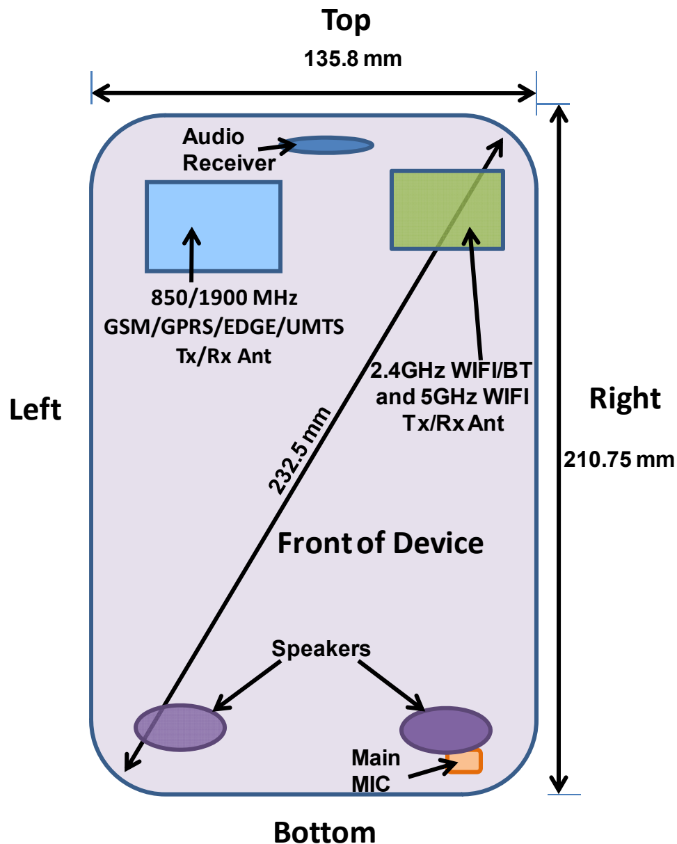
Figure 1-1 DUT Antenna Locations
