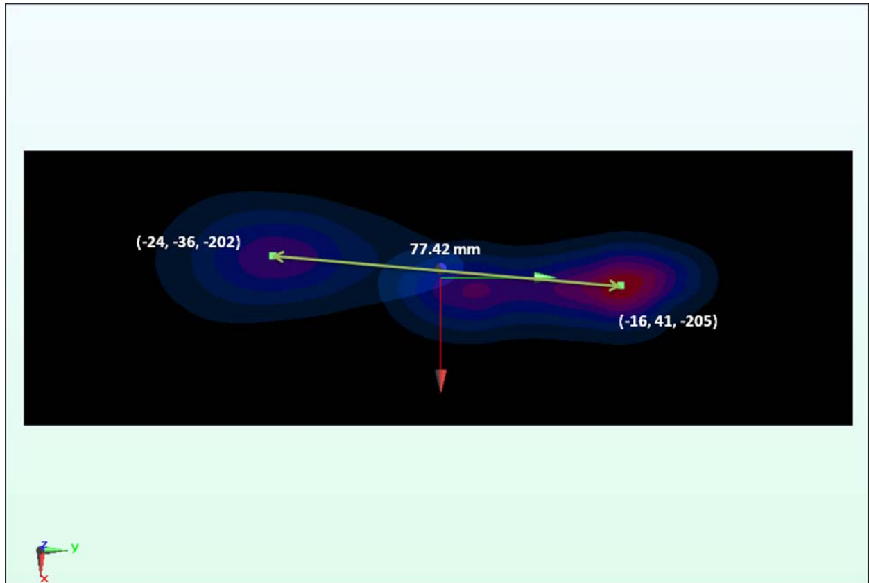
Figure 11-11 Peak SAR Locations of 2.4 GHz WLAN and GPRS 1900
