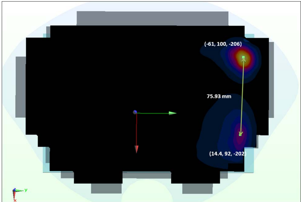
Figure 11-6 Peak SAR Locations of 2.4 GHz WLAN and UMTS 850
