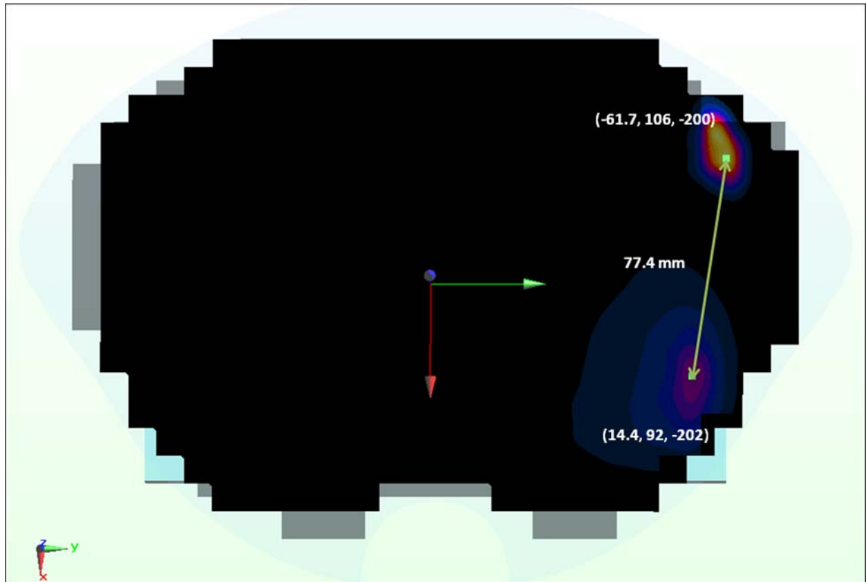
Figure 11-19 Peak SAR Locations of 5 GHz WLAN and UMTS 850
