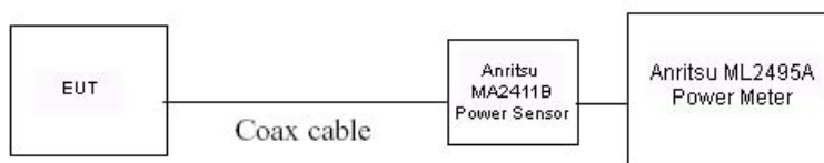
Figure 8-3 Power Measurement Setup
