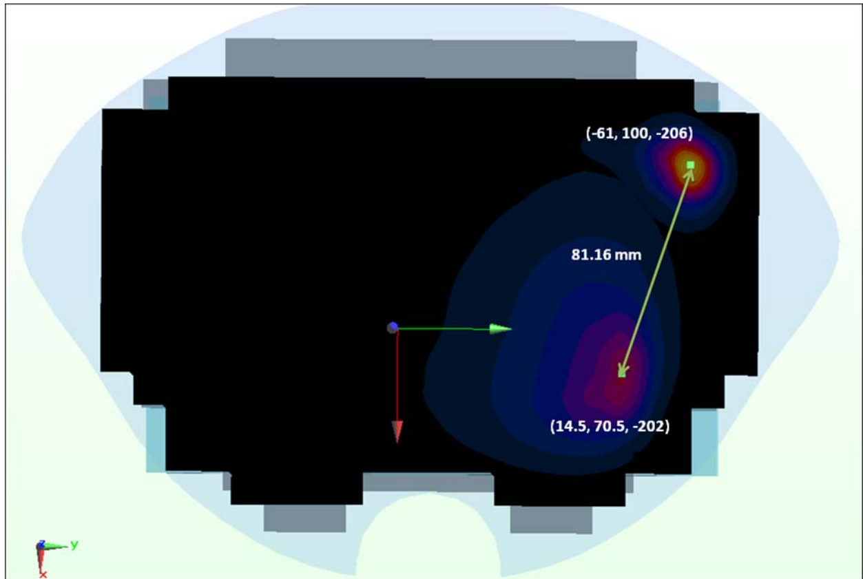
Figure 11-2 Peak SAR Locations of 2.4 GHz WLAN and UMTS 850
