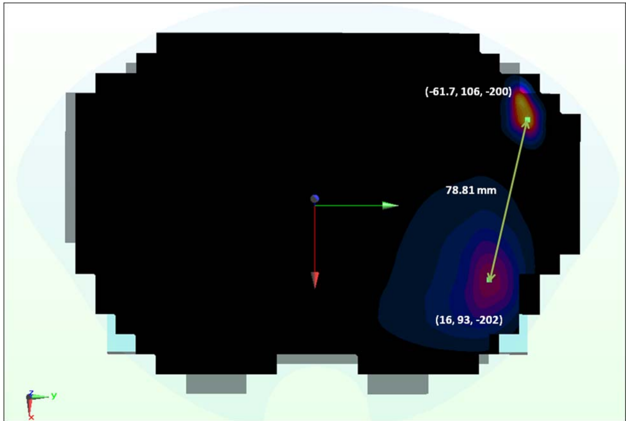
Figure 11-18 Peak SAR Locations of 5 GHz WLAN and GPRS 850
