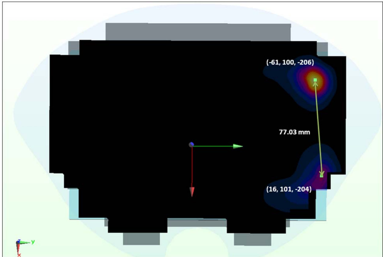
Figure 11-4 Peak SAR Locations of 2.4 GHz WLAN and UMTS 1900
