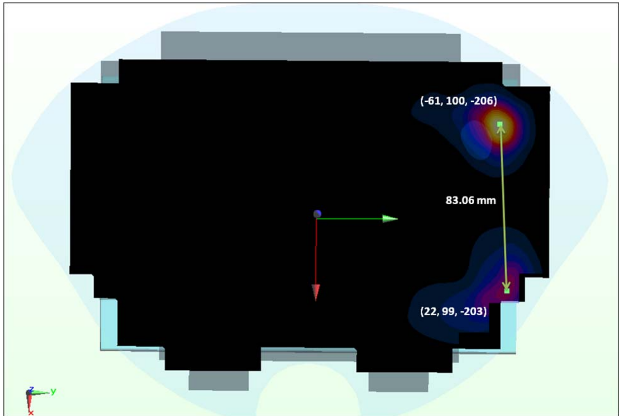
Figure 11-3 Peak SAR Locations of 2.4 GHz WLAN and GPRS 1900
