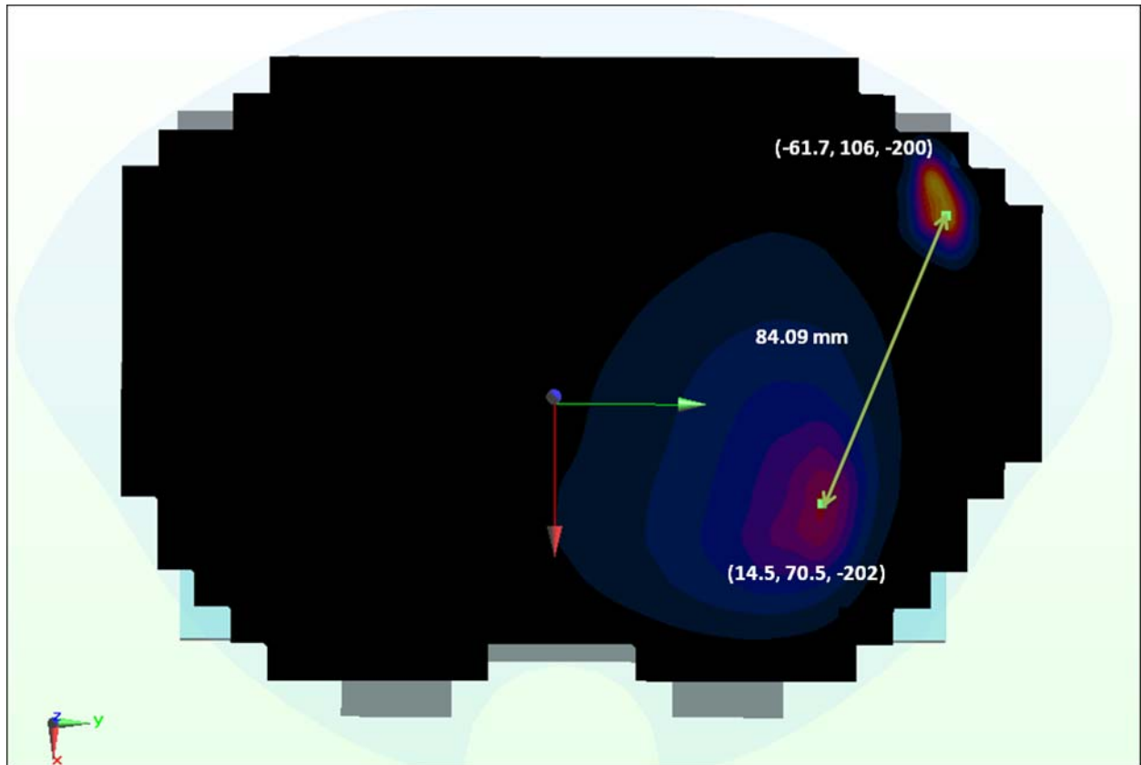
Figure 11-15 Peak SAR Locations of 5 GHz WLAN and UMTS 850
