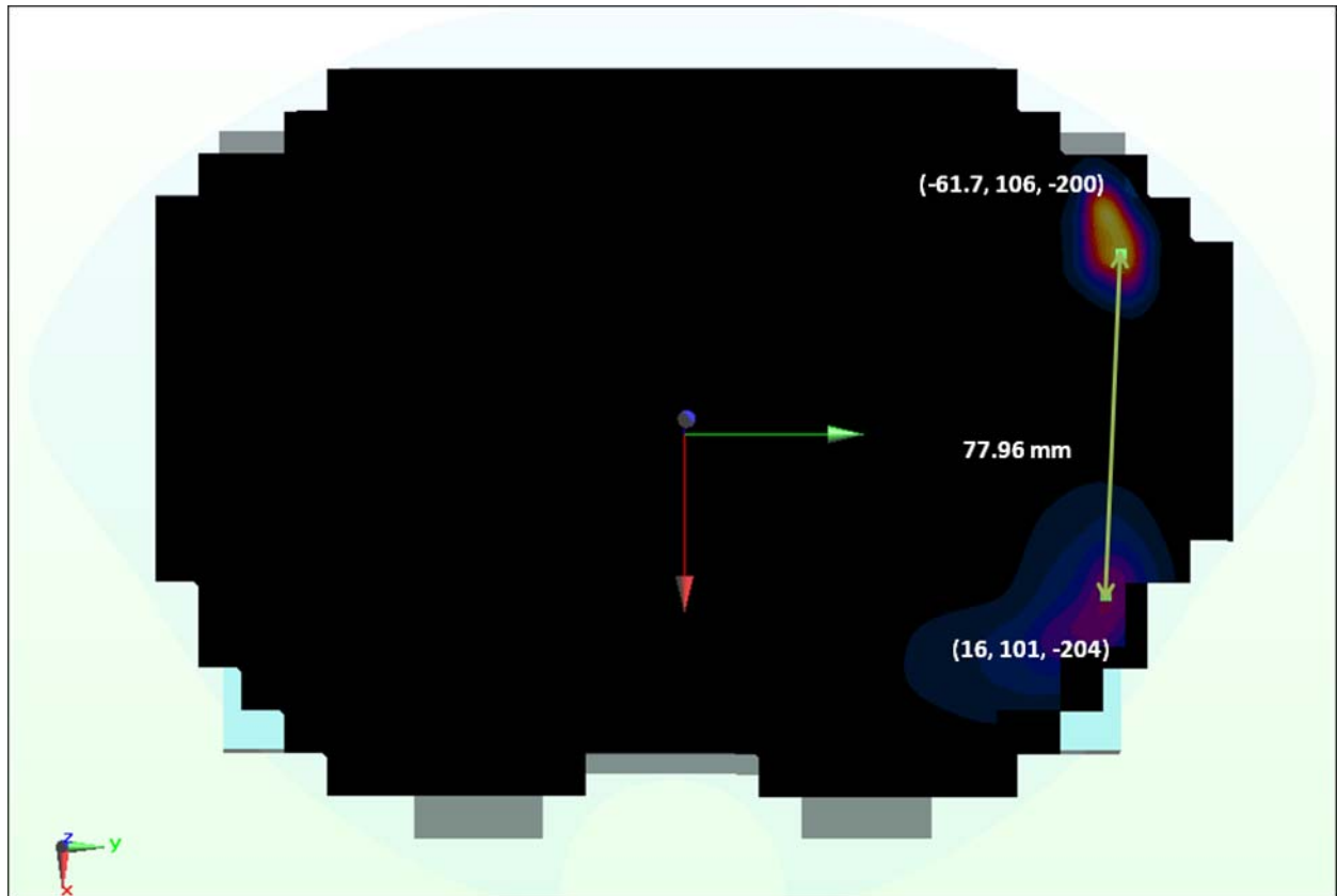
Figure 11-17 Peak SAR Locations of 5 GHz WLAN and UMTS 1900
