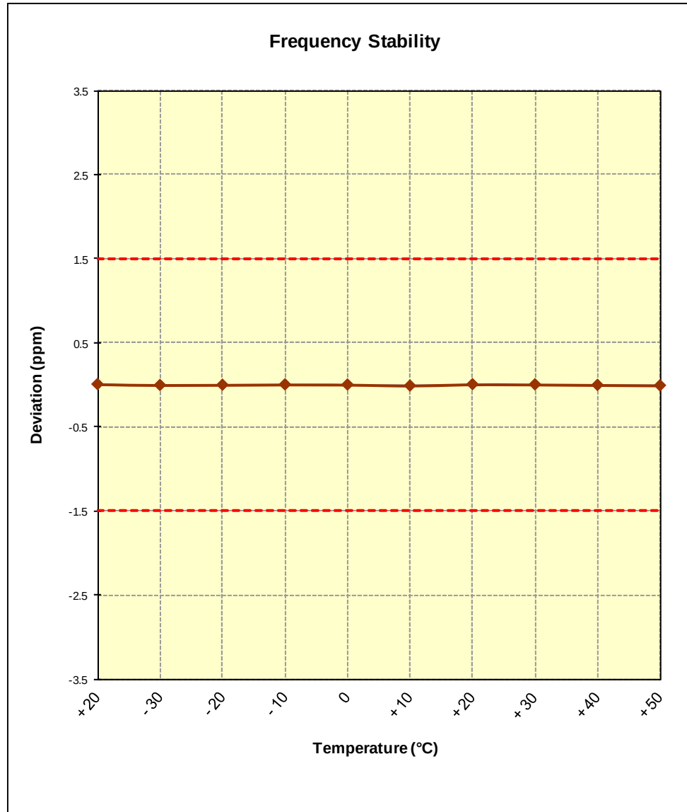
Figure 6-4. Frequency Stability Graph (PCS WCDMA Mode – Ch. 9400)
