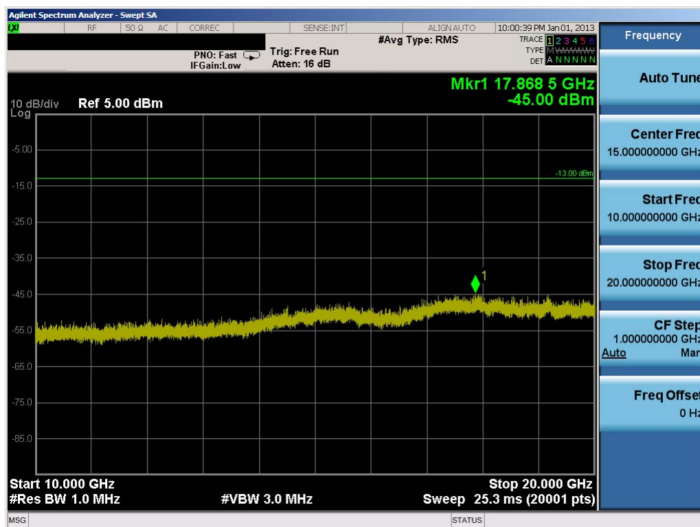
Plot 7-43. Conducted Spurious Plot (PCS WCDMA Mode – Ch. 9538)
