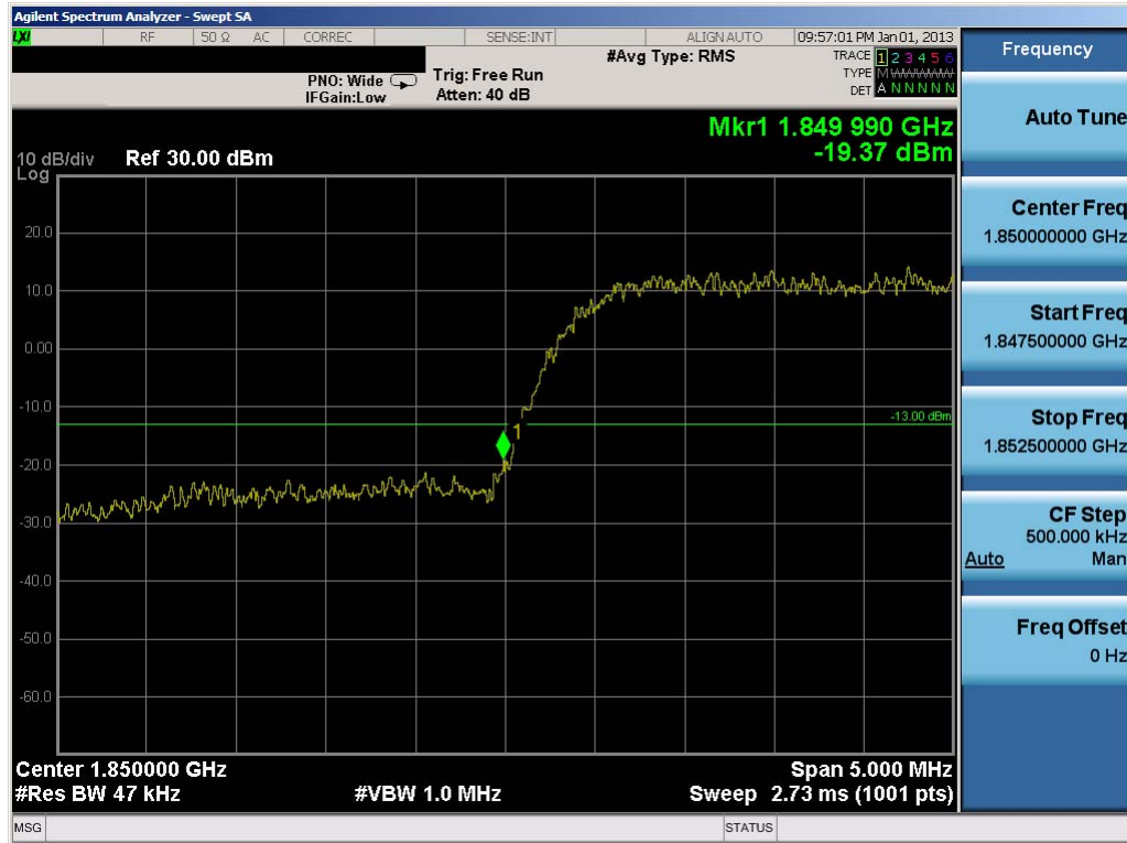
Plot 7-36. Band Edge Plot (PCS WCDMA Mode – Ch. 9262)
