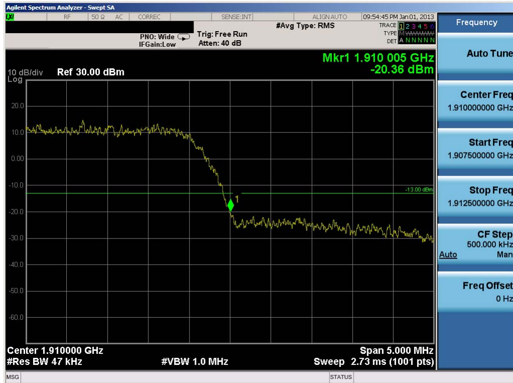
Plot 7-44. Band Edge Plot (PCS WCDMA Mode – Ch. 9538)
