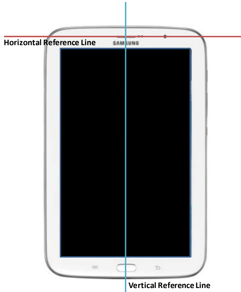
SAR Test Setup Photo 11 – DUT Reference Lines
