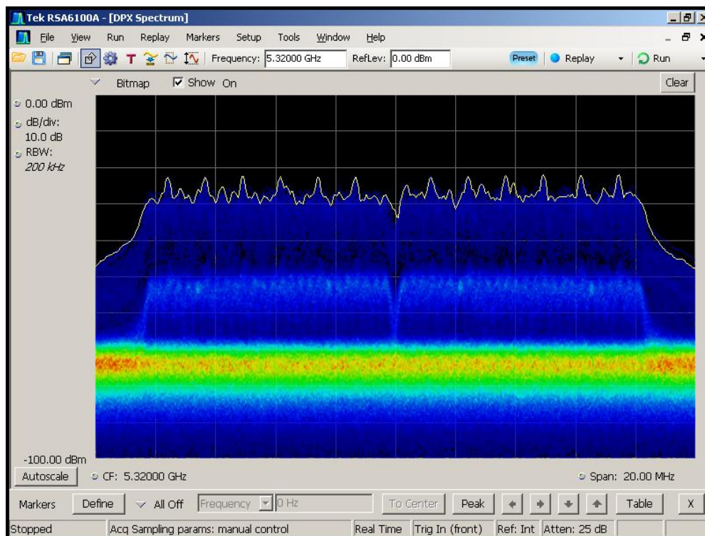
Figure 5-2. Real-Time Spectrum Display WLAN Channel Traffic (Streaming Video)
