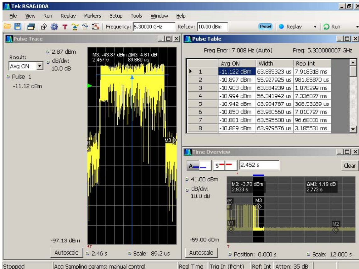
Figure 5-5. Aggregate Time using Pulse Table Capability
