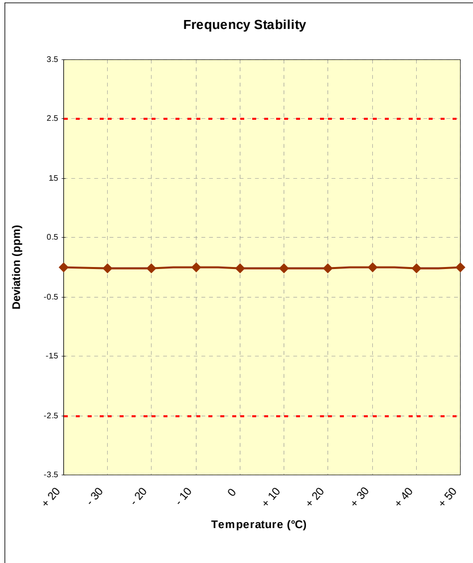
Figure 6-2. Frequency Stability Graph (Cellular WCDMA Mode – Ch. 384)
