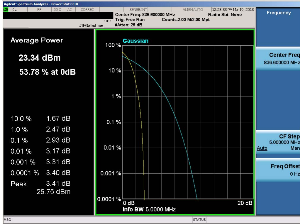
Plot 7-32. Peak-Average Ratio Plot (Cellular WCDMA Mode – Ch. 4183)
