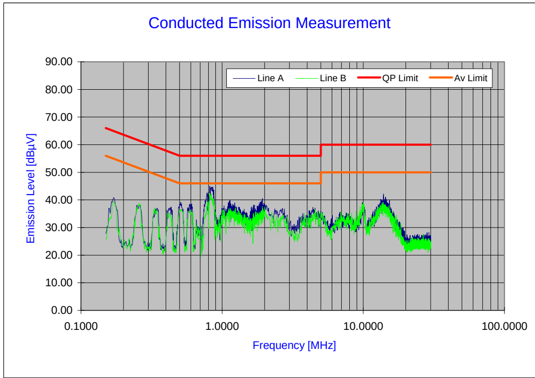
Plot 6-57. Line Conducted Plot with 802.11a UNII Band 1
