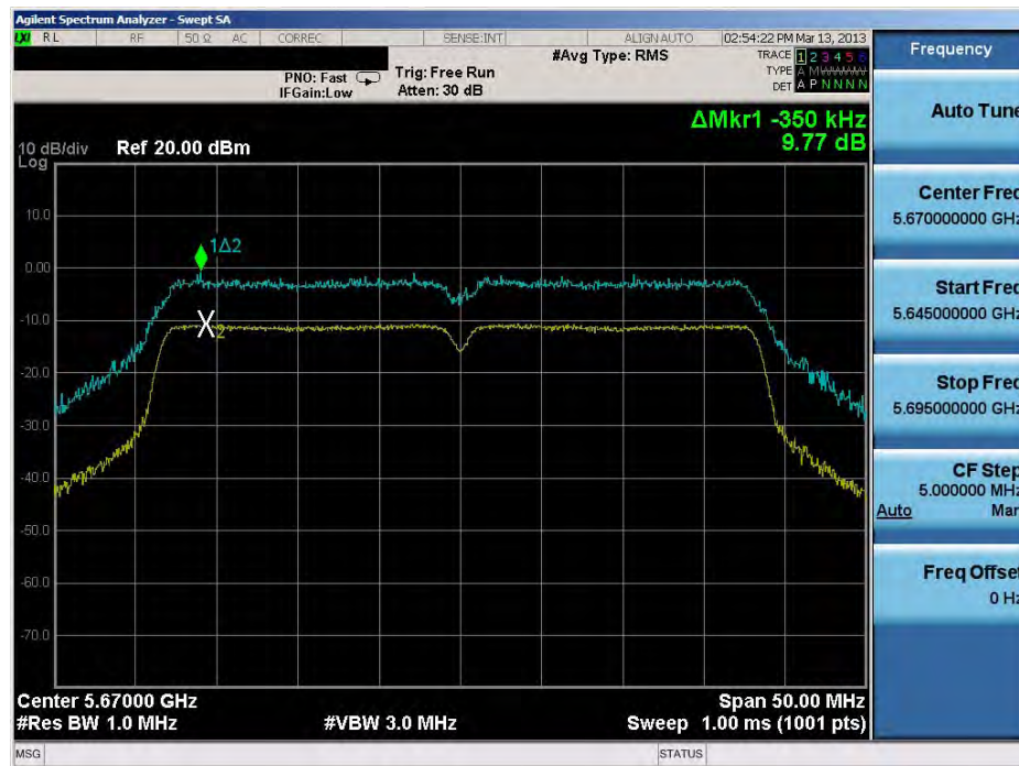
Plot 6-56. Peak Excursion Ratio Plot (40MHz BW 802.11n)
