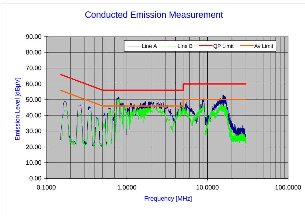
Plot 6-58. Line Conducted Plot with 802.11a UNII Band 2
