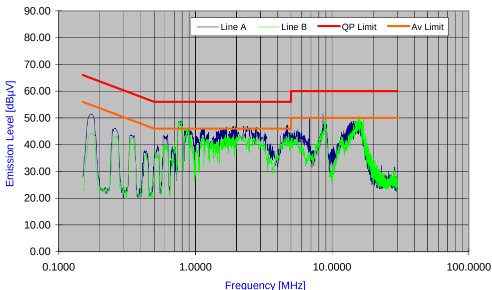
Plot 6-59. Line Conducted Plot with 802.11a UNII Band 3
