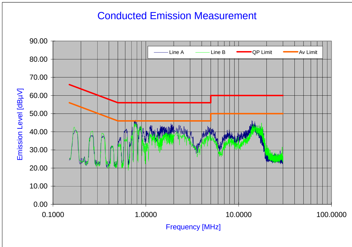
Plot 6-61. Line Conducted Plot with 802.11b
