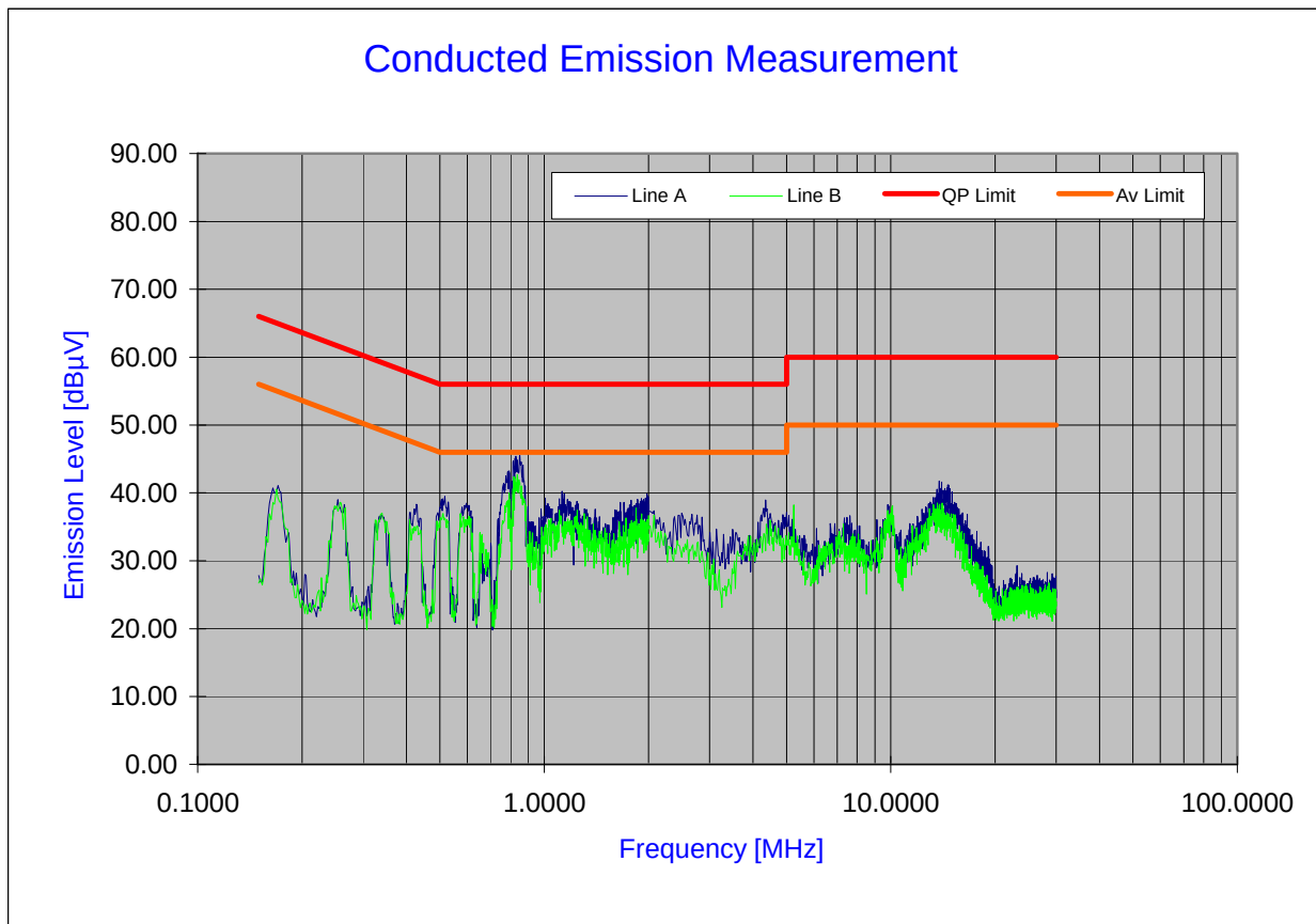
Plot 6-62. Line Conducted Plot with 802.11a
