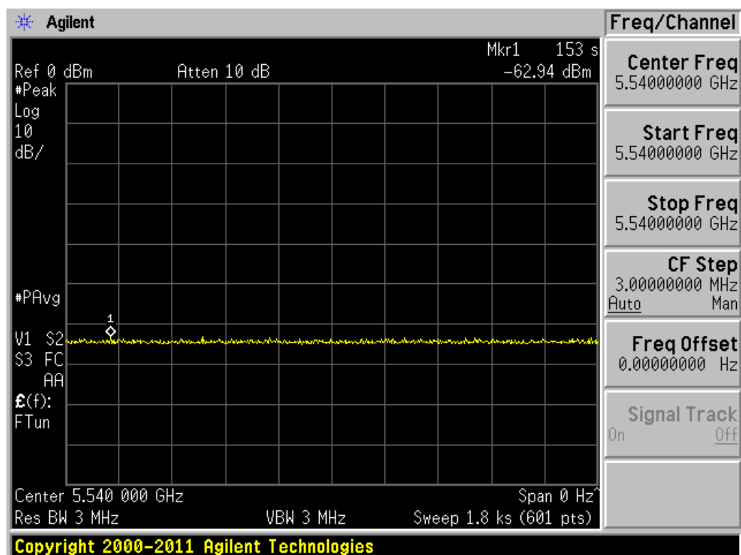
Figure 6-6. Non-occupancy Period - Monitoring live spectrum - Elapsed time 30 minutes
