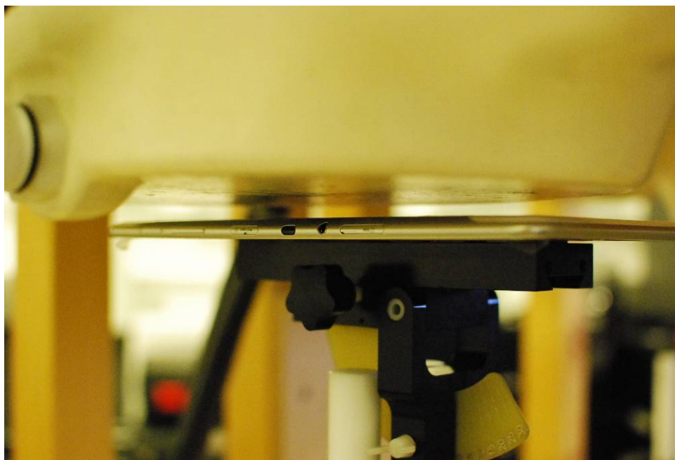
SAR Test Setup Photo 2 - Back Side at 1.0 cm
