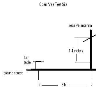
Figure 3-1. Diagram of 3-meter outdoor test range
