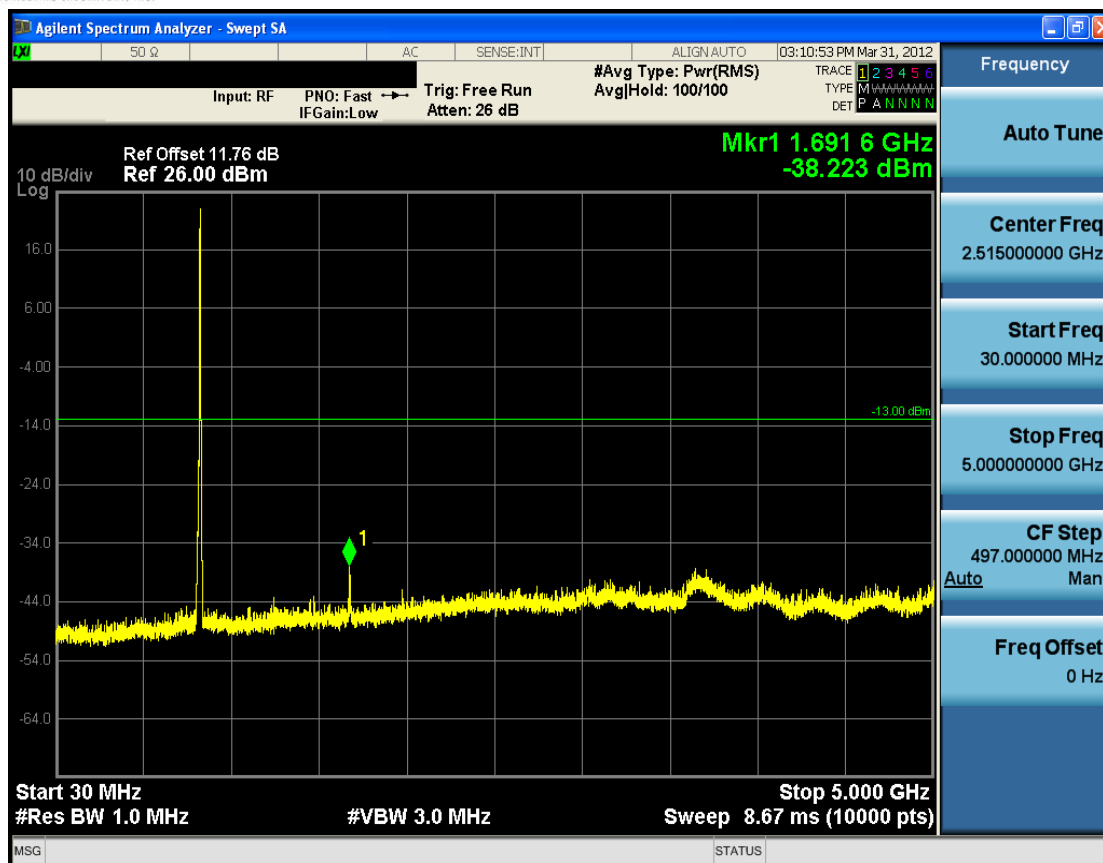
Plot 7-27. Conducted Spurious Plot (Cellular WCDMA Mode – Ch. 4183)
