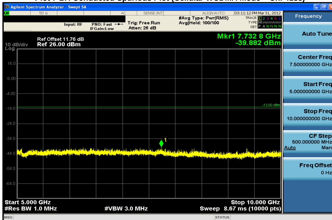
Plot 7-28. Conducted Spurious Plot (Cellular WCDMA Mode – Ch. 4183)
