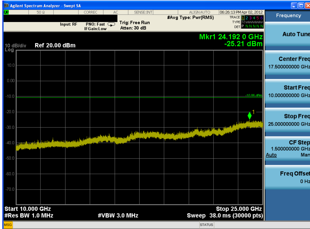
Plot 6-19. Conducted Spurious Plot (Bluetooth, 1Mbps – Ch. 0)
