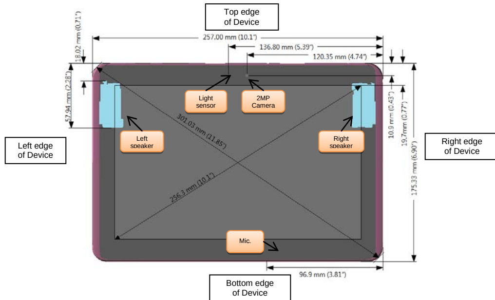
Figure 9-1 Front View of Device
