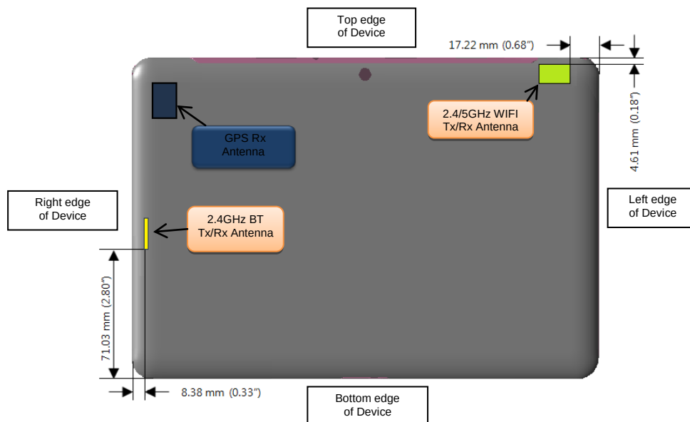
Figure 9-2 Back View of Device
