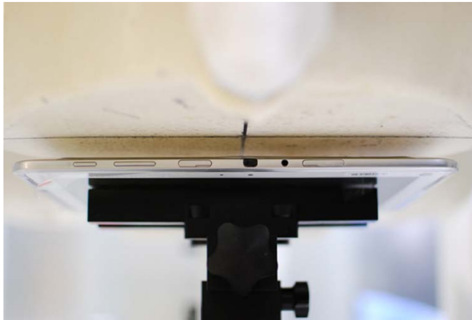
SAR Test Setup Photo 2: Back at 1.2 cm
