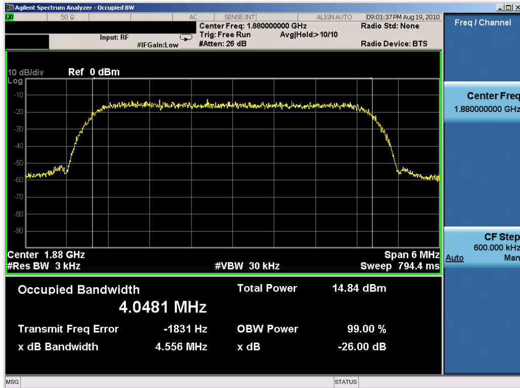
Plot 7-29. Occupied Bandwidth Plot (PCS WCDMA Mode – Ch. 9400)
