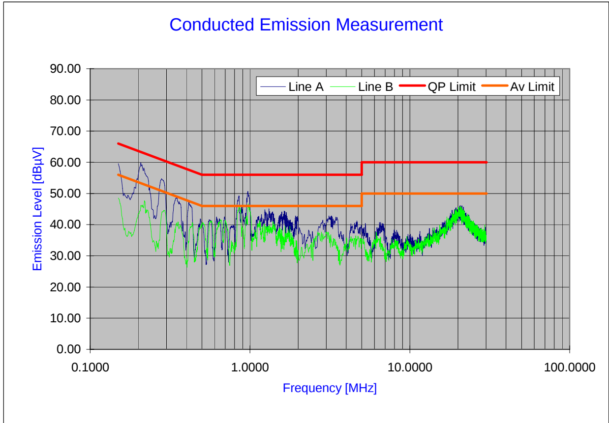
Plot 6-59. Line Conducted Plot with 802.11n (UNII-II Band)
