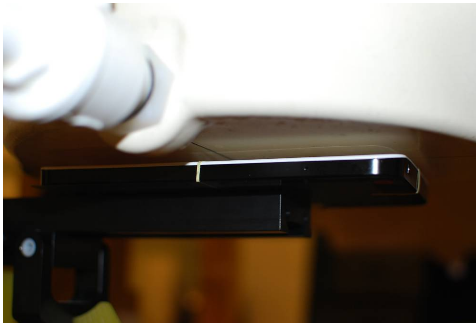
Figure 20-1 SAR Test Setup Photo 1 – Back Side at 0.5 cm (with power back-off active)
