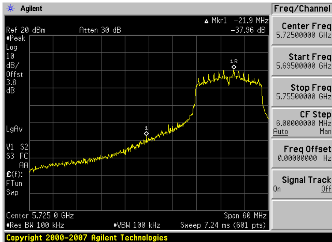
Plot 6-35. Band Edge Plot (802.11a – Ch. 149)
