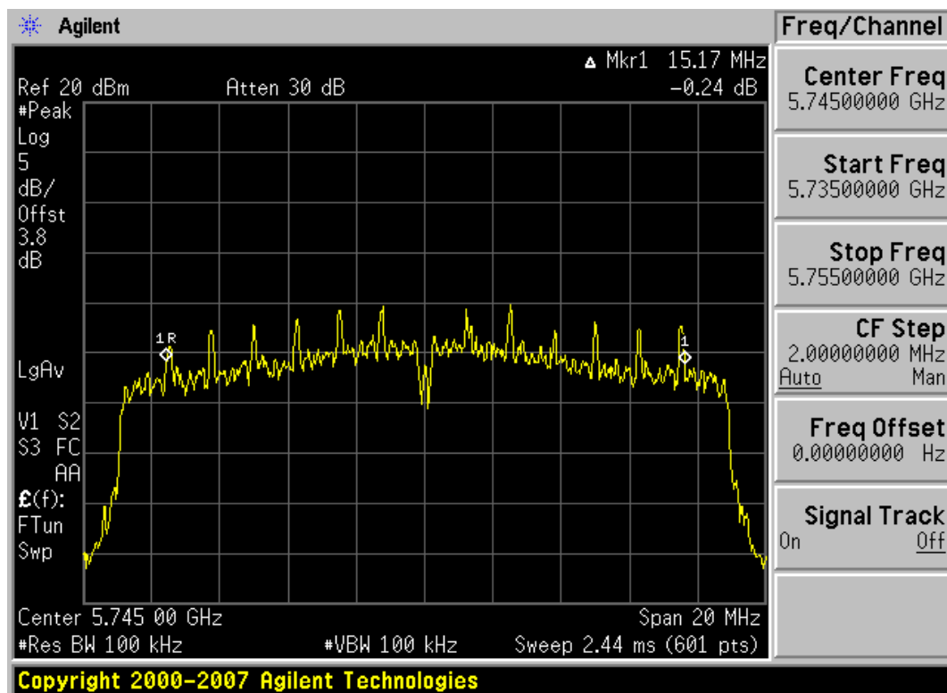
Plot 6-13. 6dB Bandwidth Plot (802.11n (5.8GHz) - Ch. 149)
