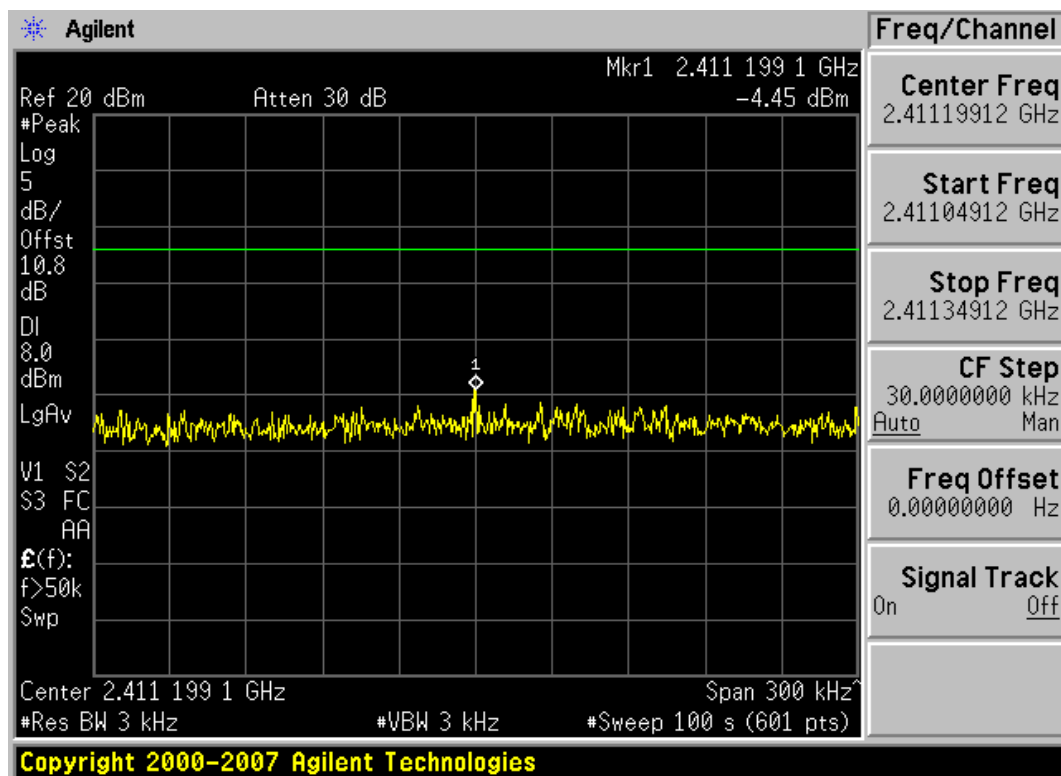
Plot 6-16. Power Spectral Density Plot (802.11b – Ch. 1)
