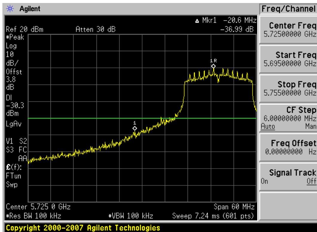
Plot 6-39. Band Edge Plot (802.11n (5.8GHz) – Ch. 149)
