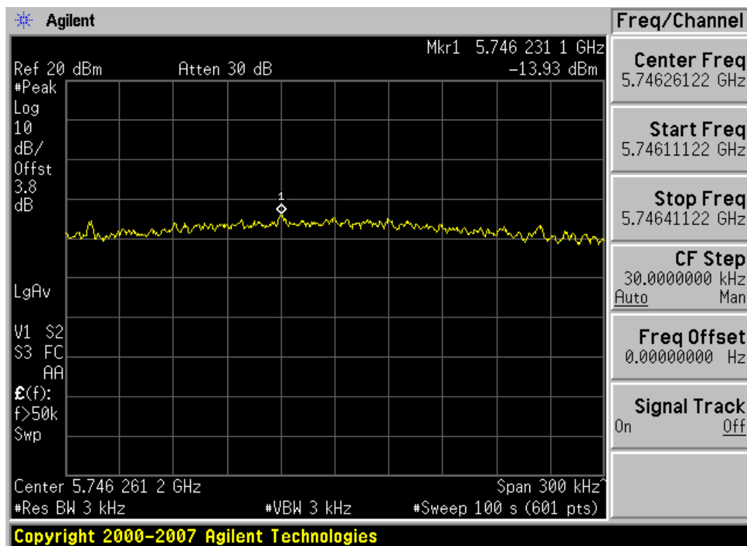
Plot 6-22. Power Spectral Density Plot (802.11a – Ch. 149)
