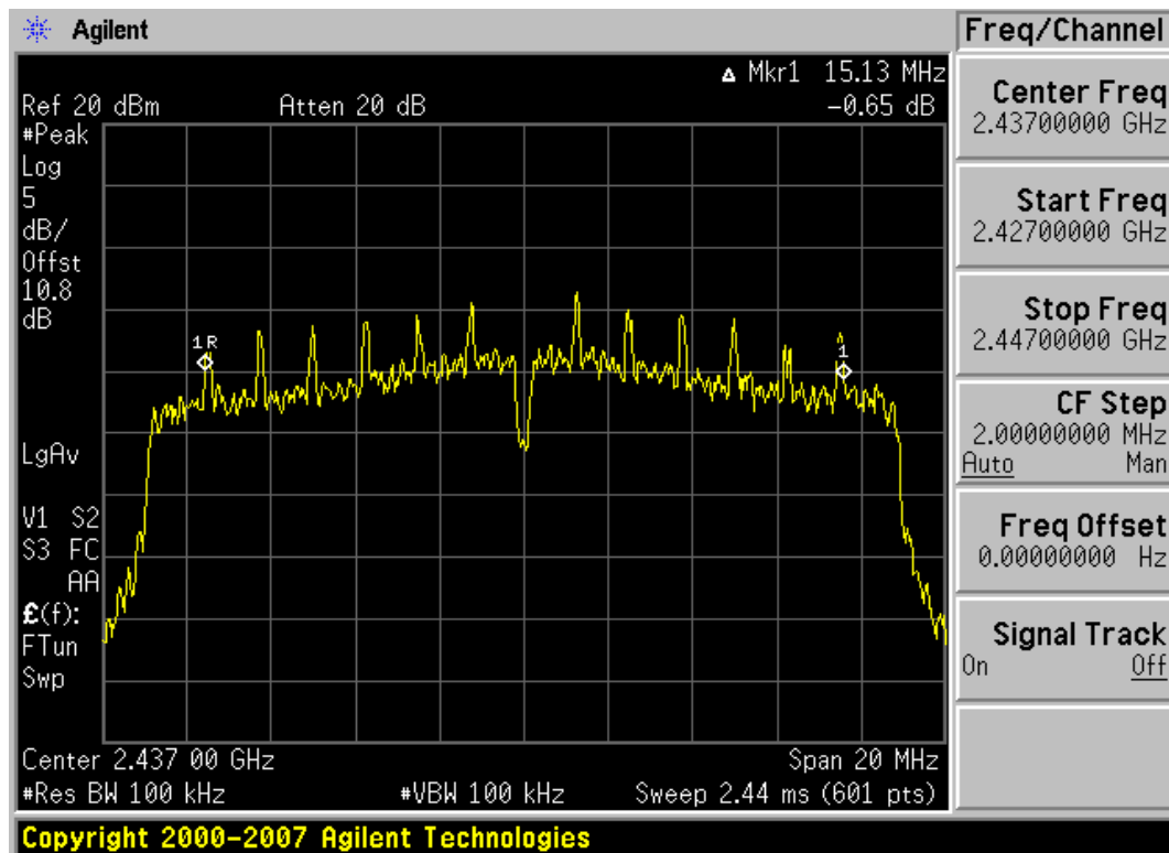
Plot 6-11. 6dB Bandwidth Plot (802.11n (2.4GHz) – Ch. 6)
