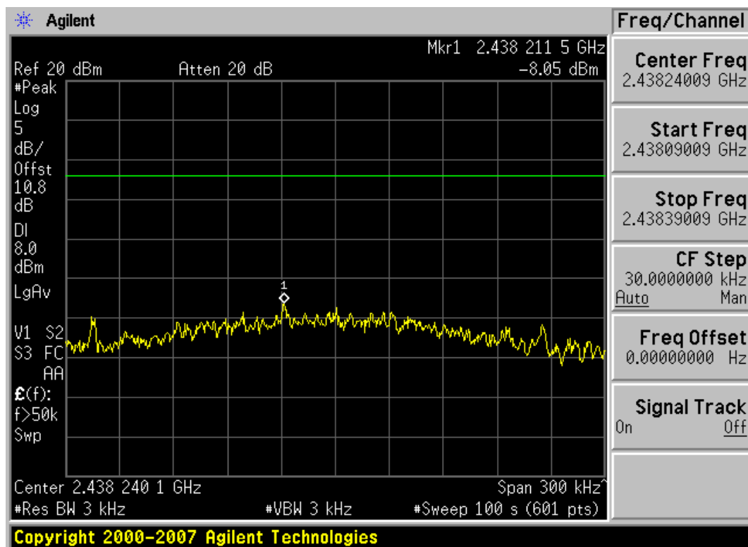
Plot 6-20. Power Spectral Density Plot (802.11g - Ch. 6)
