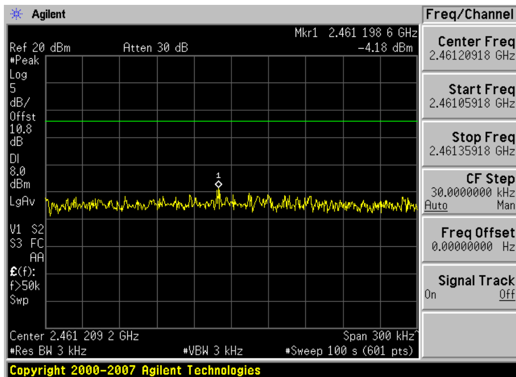
Plot 6-18. Power Spectral Density Plot (802.11b – Ch. 11)
