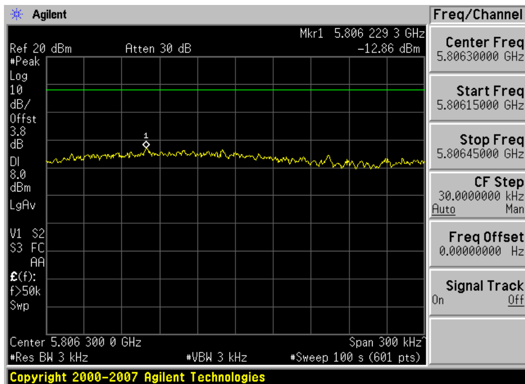
Plot 6-24. Power Spectral Density Plot (802.11a – Ch. 161)
