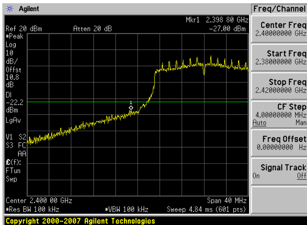
Plot 6-37. Band Edge Plot (802.11n (2.4GHz) – Ch. 1)
