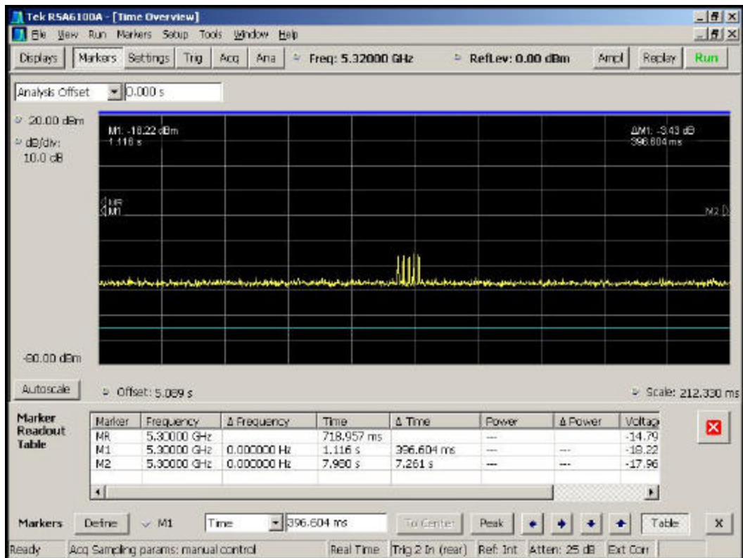
Figure 5-9. Pulse grouping 3
