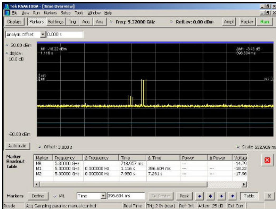
Figure 5-7. Pulse grouping 1
