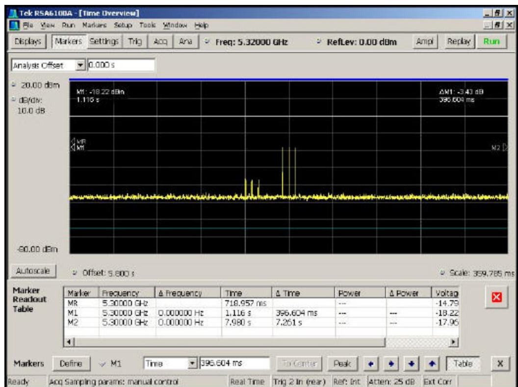
Figure 5-10. Pulse grouping 4
