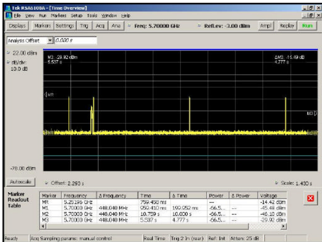
Figure 6-7. Pulse Grouping 2
