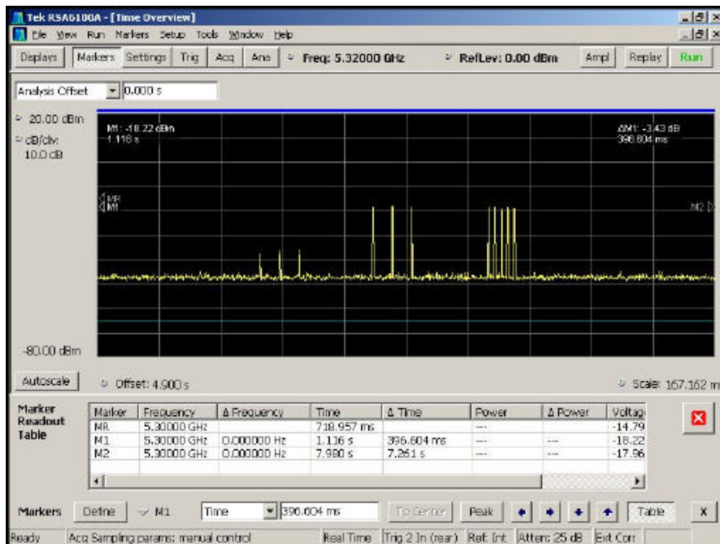
Figure 5-8. Pulse grouping 2
