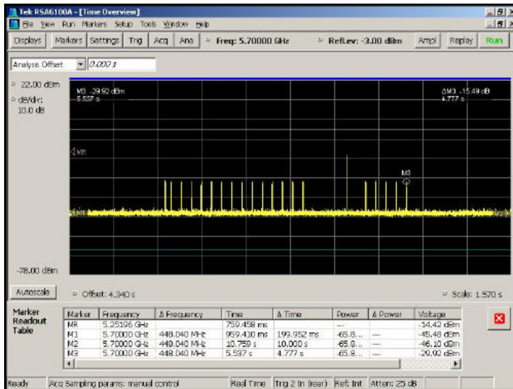
Figure 6-8. Pulse Grouping 3
