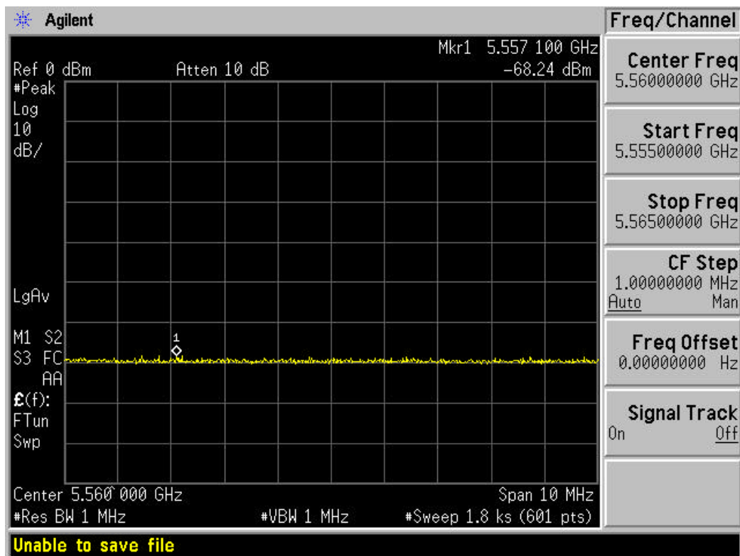
Figure 6-10 Non-occupancy Period - Monitoring live real time spectrum - Elapse time 30 minutes
