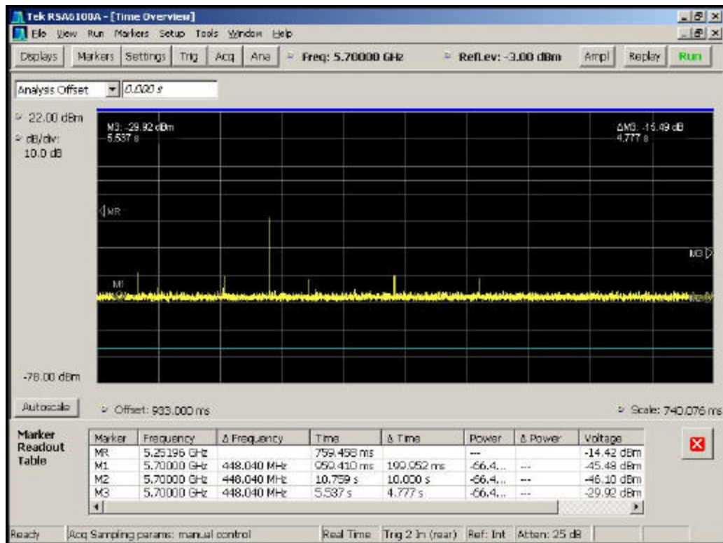
Figure 6-6. Pulse Grouping 1
