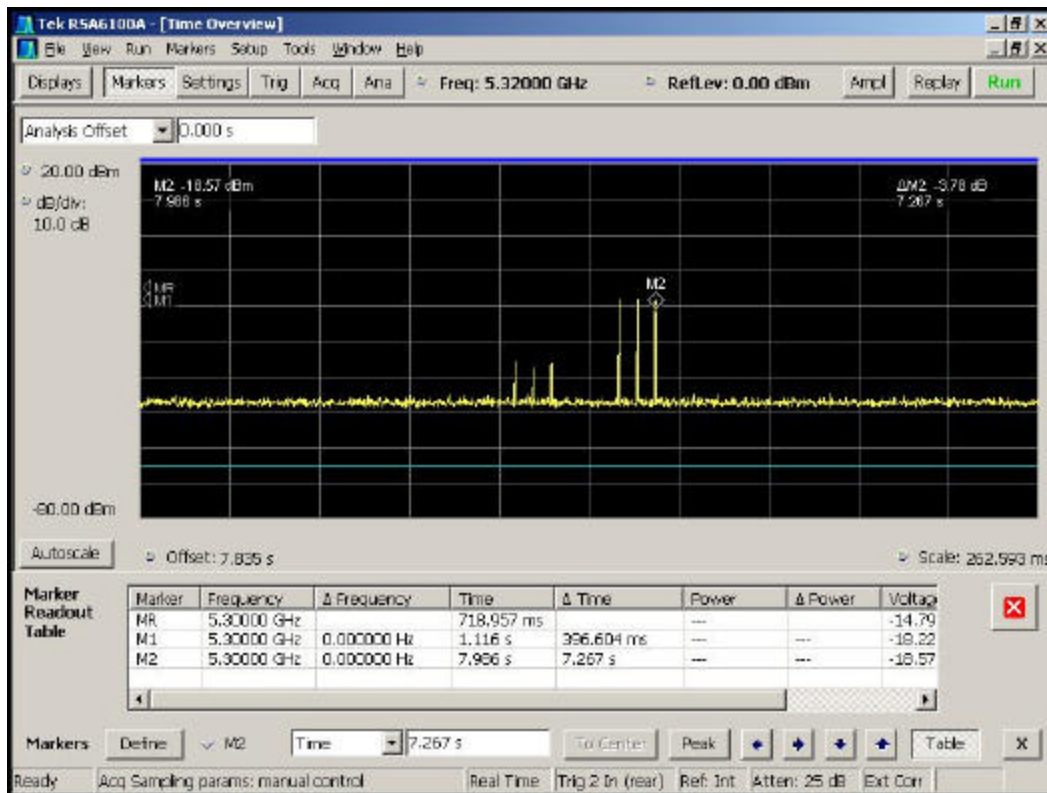
Figure 5-11. Pulse grouping 5
