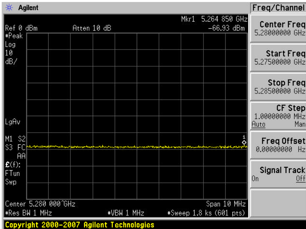
Figure 5-13 Non-occupancy Period - Monitoring live real time spectrum - Elapse time 30 minutes
