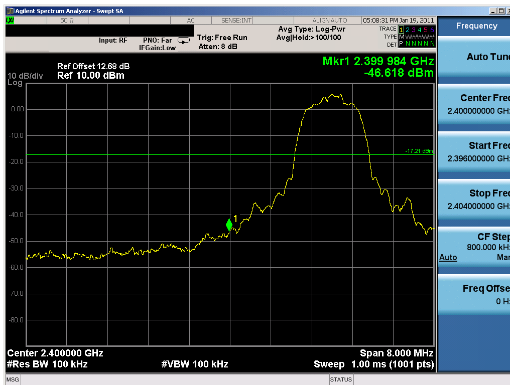
Plot 6-12. Band Edge Plot (Bluetooth, 2Mbps – Ch. 0)
