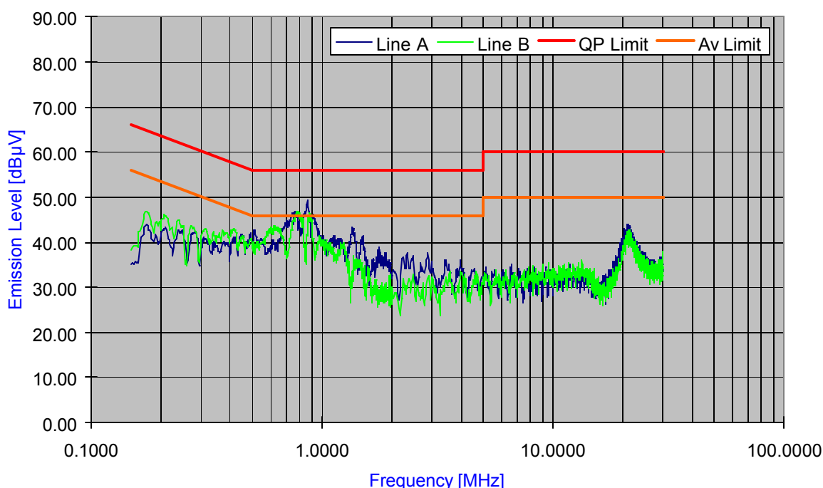
Plot 6-58. Line Conducted Plot with 802.11n (UNII-I Band)
