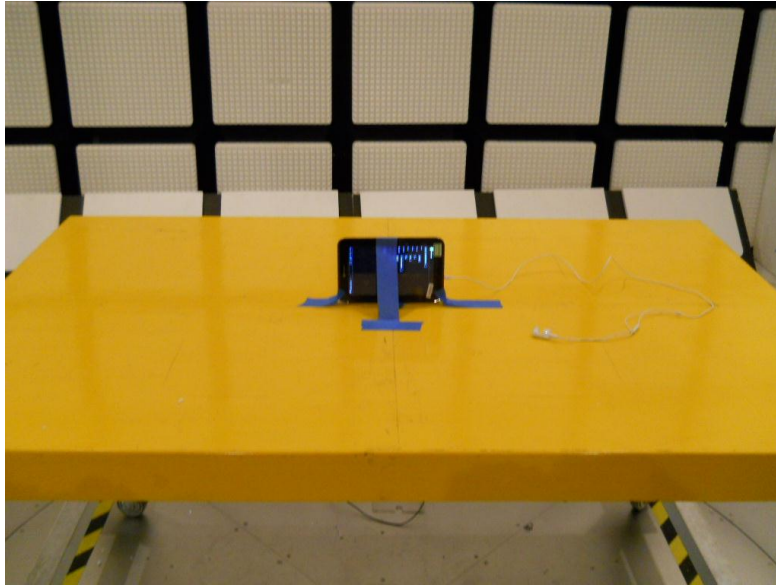
Y-AXIS WITH HEADSET FRONT PHOTO
