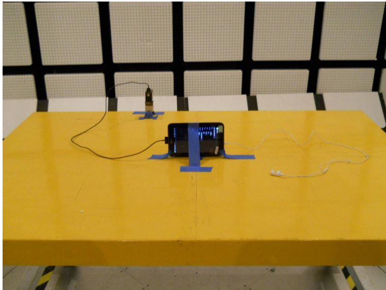
Y-AXIS WITH HEADSET AND AC ADAPTER FRONT PHOTO
