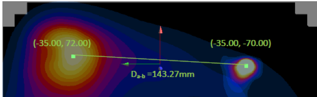
Figure 11-11 Peak SAR Locations of GPRS 850 and 5 GHz WLAN
