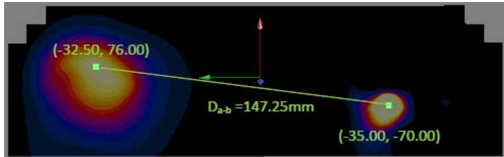
Figure 11-8 Peak SAR Locations of LTE Band 5 and 5 GHz WLAN
