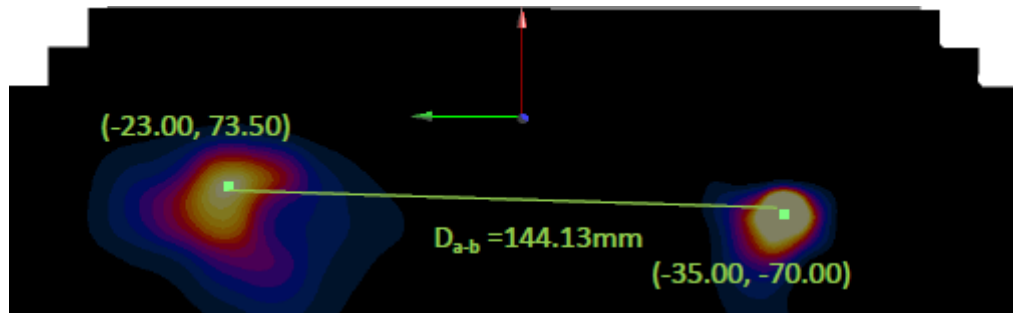
Figure 11-6 Peak SAR Locations of GPRS 1900 and 5 GHz WLAN
