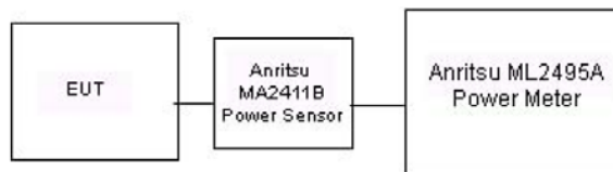
Figure 8-3 Power Measurement Setup
