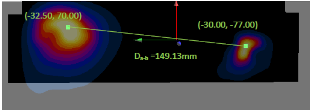
Figure 11-2 Peak SAR Locations of UMTS 850 and 2.4 GHz WLAN
