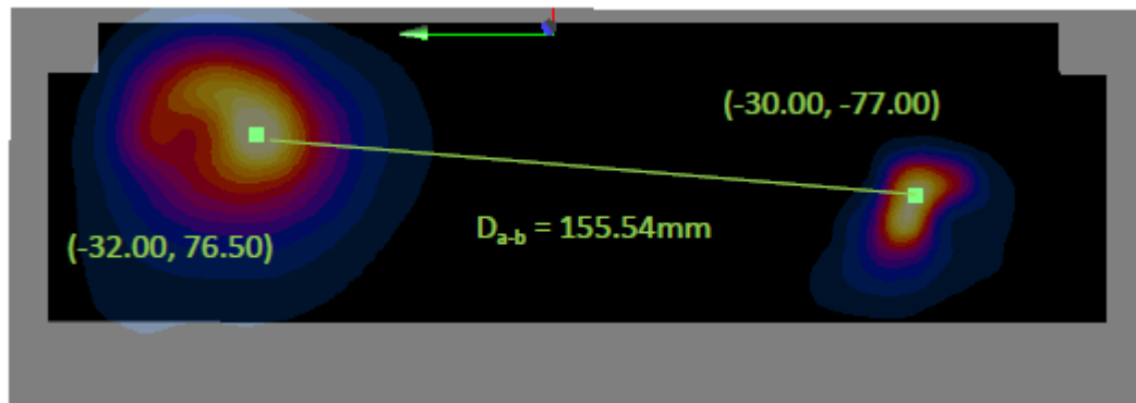
Figure 11-1 Peak SAR Locations of GPRS 850 and 2.4 GHz WLAN
