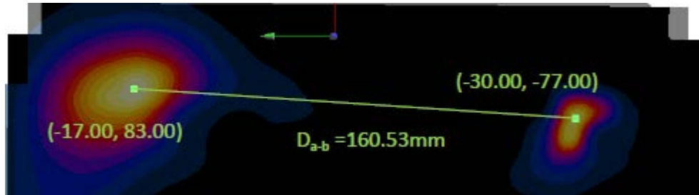
Figure 11-9 Peak SAR Locations of GPRS 1900 and 2.4 GHz WLAN
