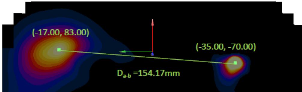
Figure 11-12 Peak SAR Locations of GPRS 1900 and 5 GHz WLAN
