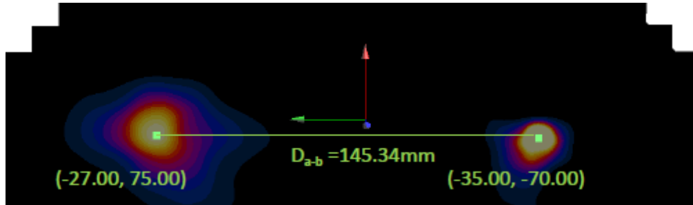
Figure 11-7 Peak SAR Locations of UMTS 1900 and 5 GHz WLAN
