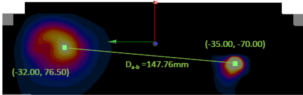
Figure 11-4 Peak SAR Locations of GPRS 850 and 5 GHz WLAN
