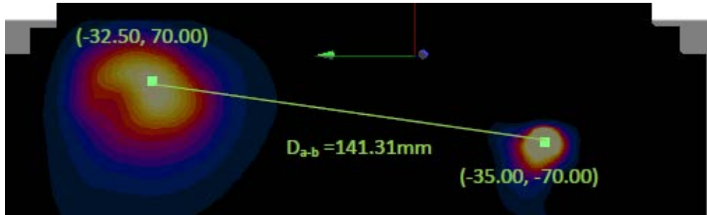
Figure 11-5 Peak SAR Locations of UMTS 850 and 5 GHz WLAN
