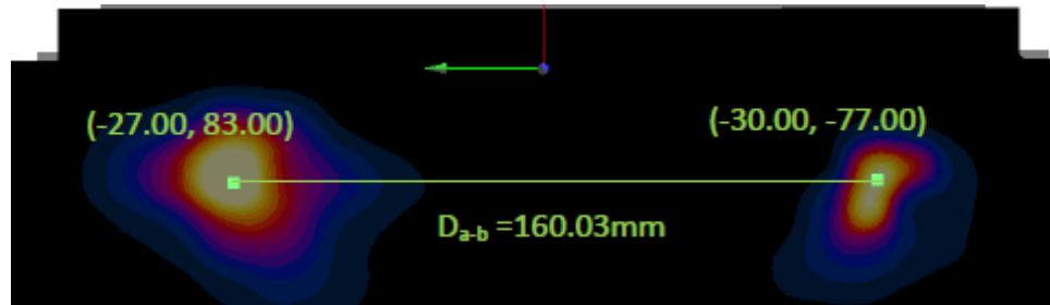
Figure 11-10 Peak SAR Locations of UMTS 1900 and 2.4 GHz WLAN
