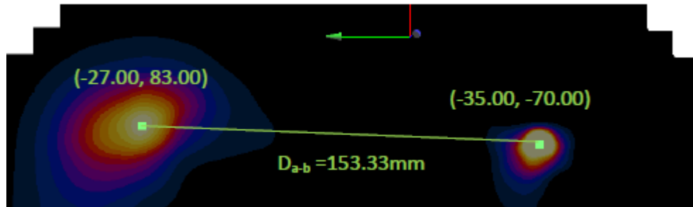
Figure 11-13 Peak SAR Locations of UMTS 1900 and 5 GHz WLAN
