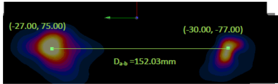
Figure 11-3 Peak SAR Locations of UMTS 1900 and 2.4 GHz WLAN
