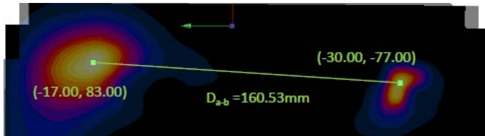
Figure 11-9 Peak SAR Locations of GPRS 1900 and 2.4 GHz WLAN
