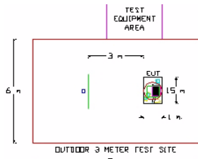
Figure 3-6. Dimensions of Outdoor Test Site
