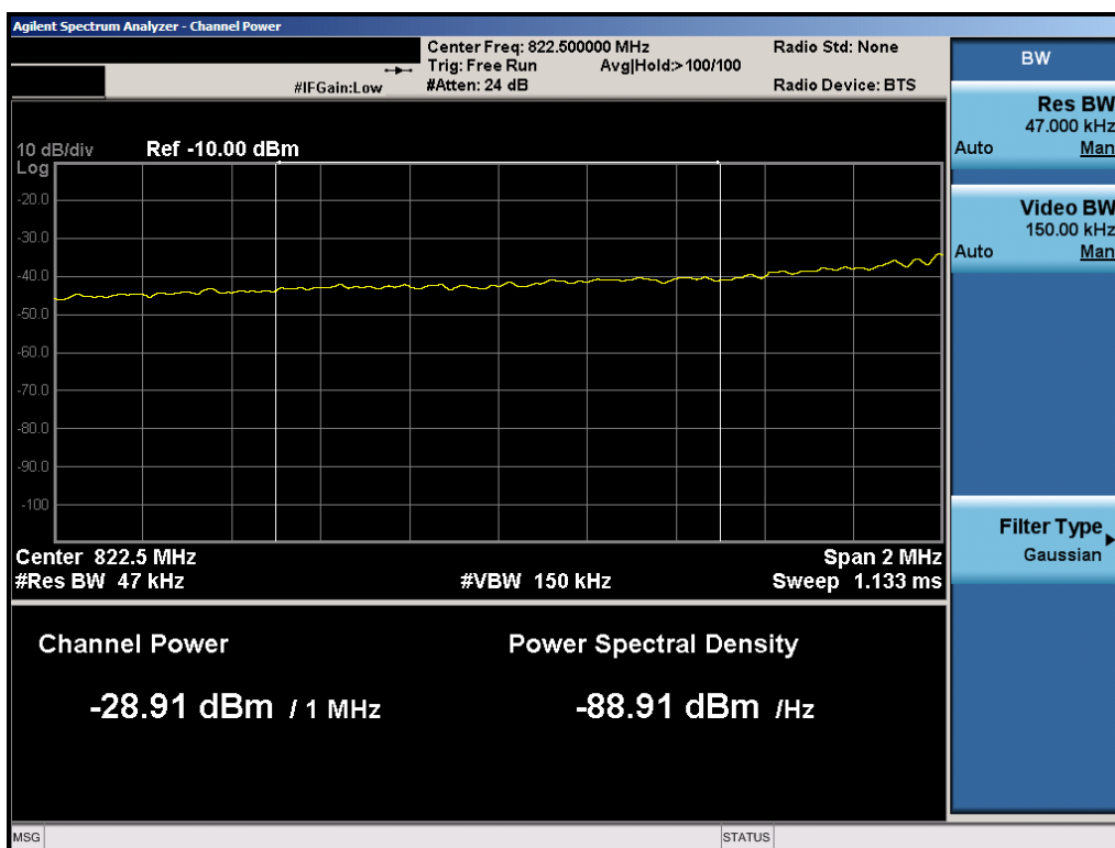
Plot 7-26. Lower Extended Band Edge Plot (5.0MHz QPSK – RB Size 25)
