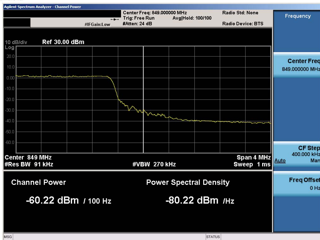
Plot 7-47. Upper Band Edge Plot (10.0MHz QPSK – RB Size 50)
