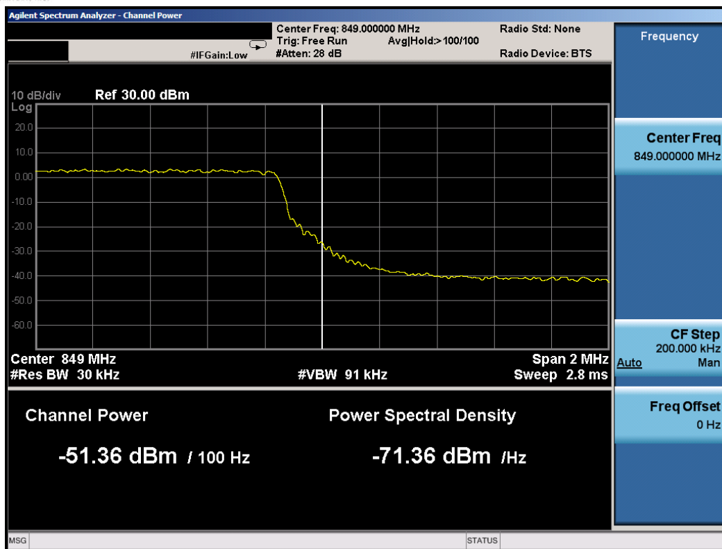
Plot 7-23. Upper Band Edge Plot (3.0MHz QPSK – RB Size 15)
