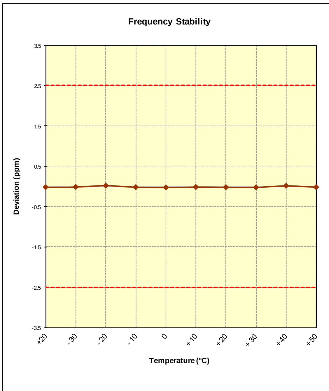
Figure 6-1. Frequency Stability Graph (Band 5)
