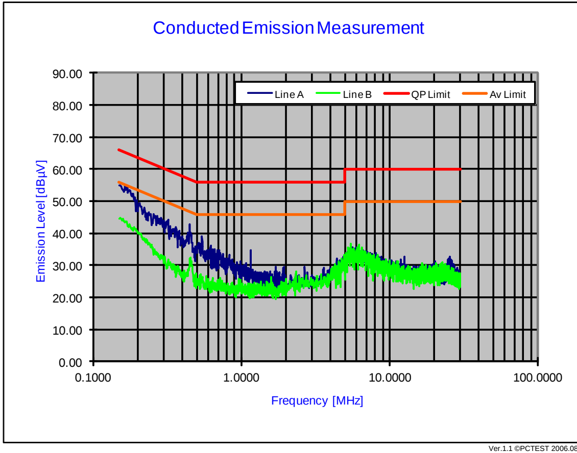
Plot 6-42. Line Conducted Plot with Bluetooth
