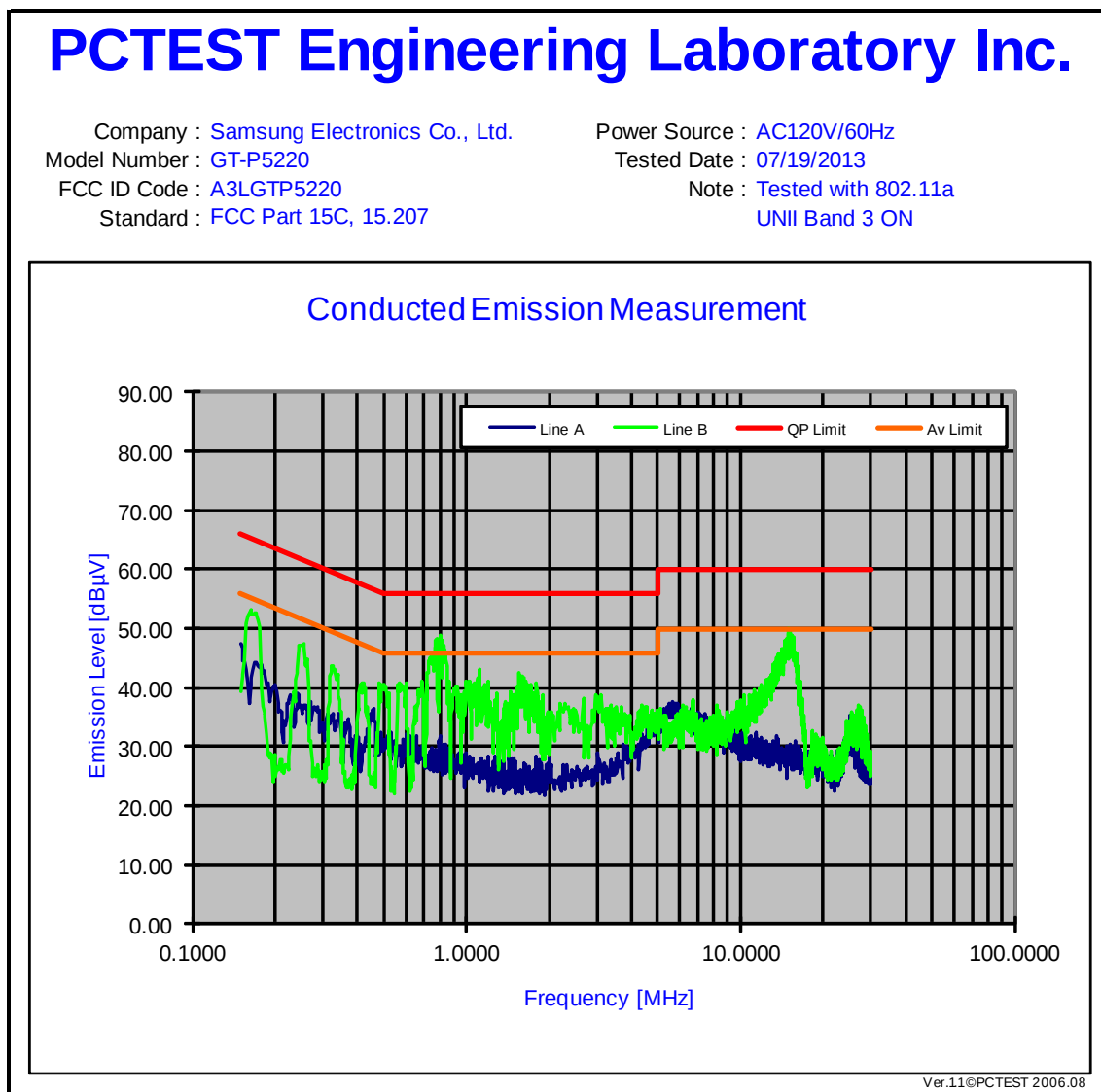
Plot 6-56. Line Conducted Plot with 802.11a (UNII Band 3)
