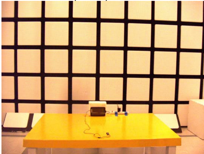
RADIATED EMISSIONS (FRONT)
