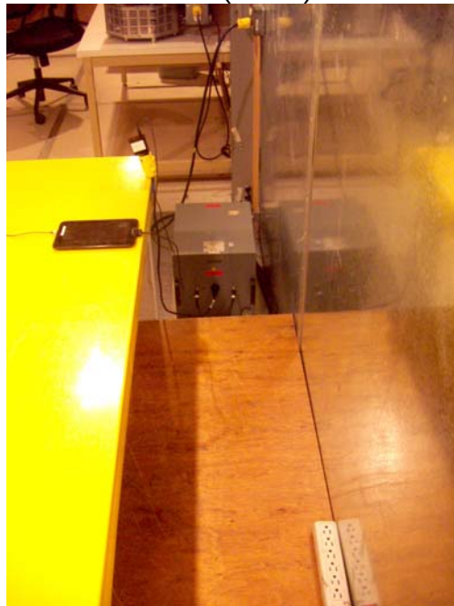
LINE CONDUCTED EMISSION (BACK)
