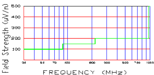
Figure 6-5. 3-Meter Limits
