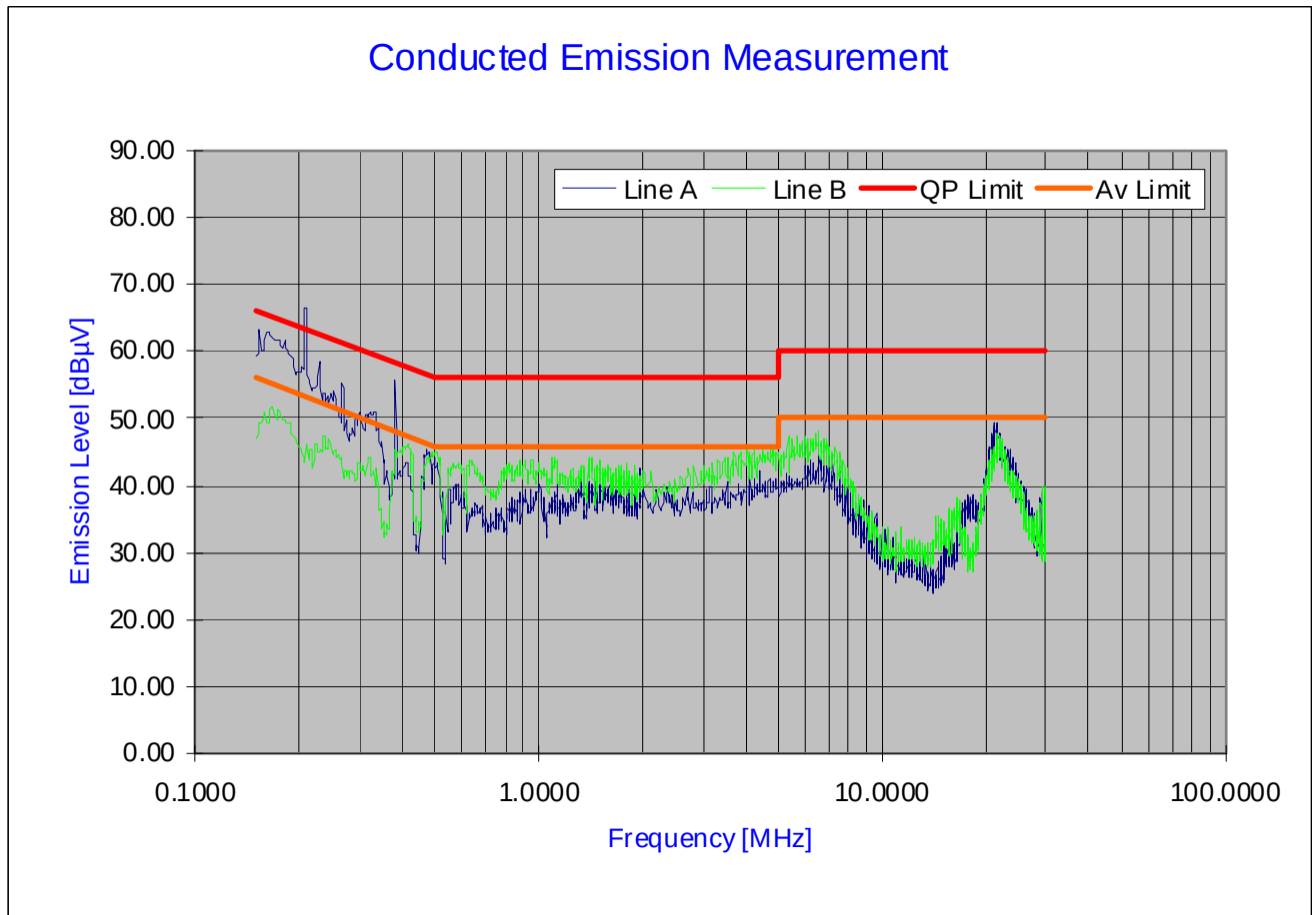
Plot 6-49. Line Conducted Plot with 802.11b
