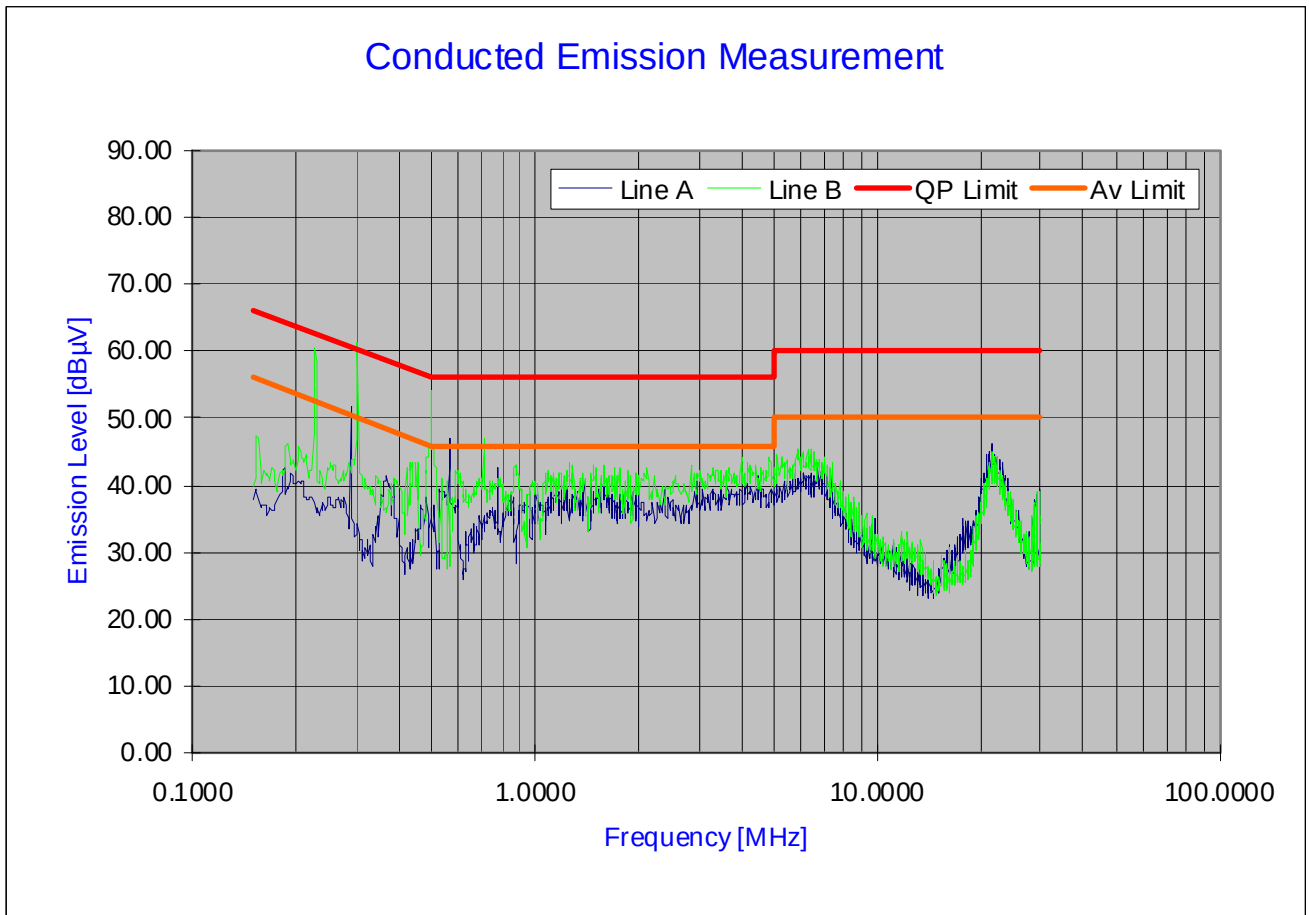
Plot 6-53. Line Conducted Plot with 802.11n (5.8GHz)
