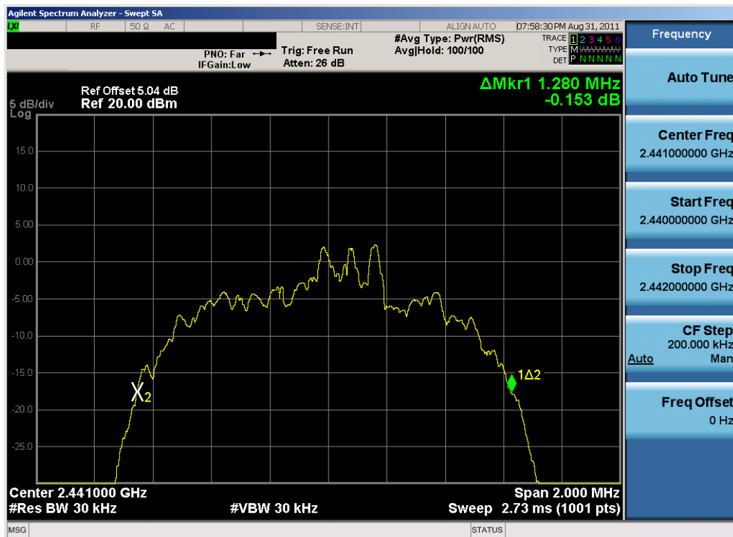
Plot 6-8. 20dB Bandwidth Plot (Bluetooth, 3Mbps – Ch. 39)
