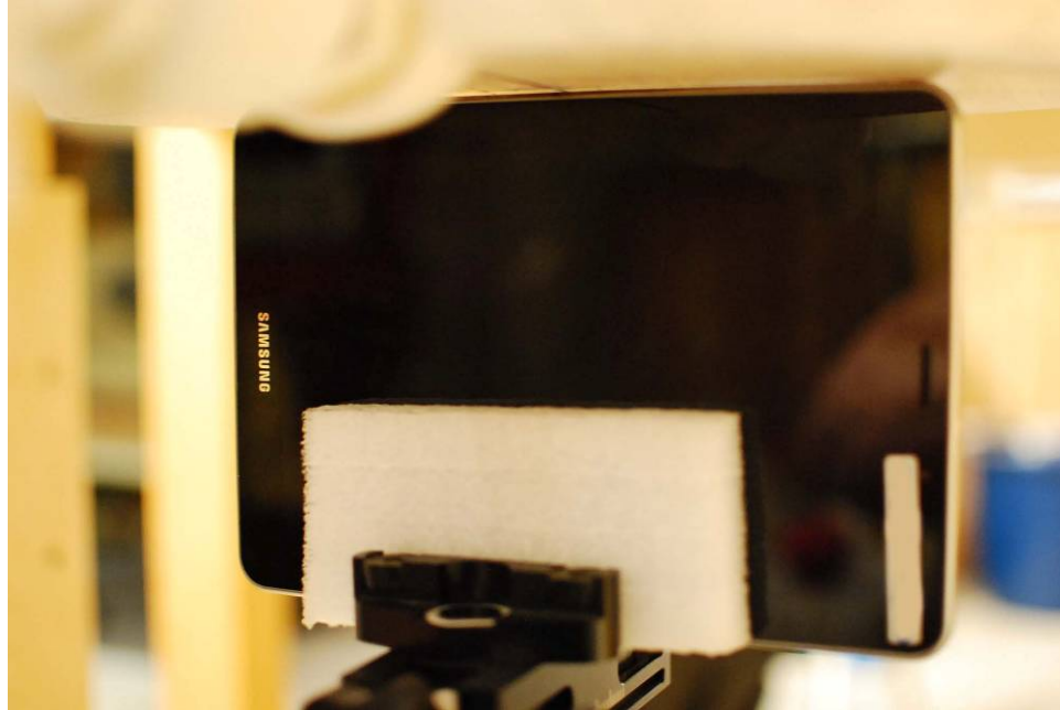
SAR Test Setup Photo 10 – Left at 0.0 cm
