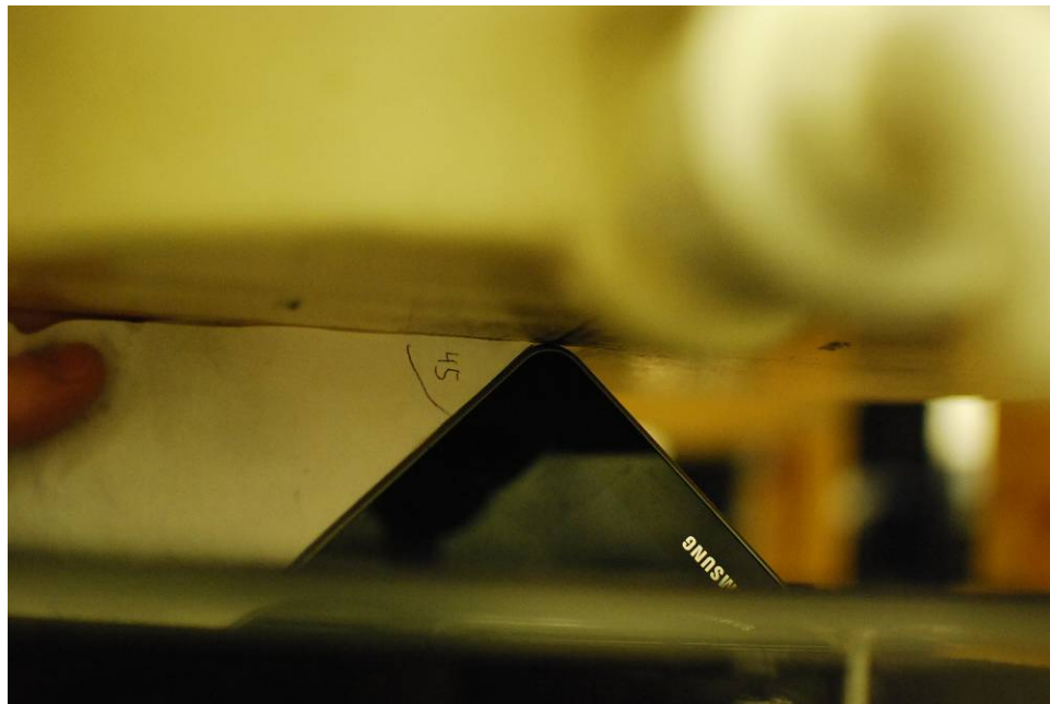
SAR Test Setup Photo 11 – 45° Vertex at 0.0 cm
