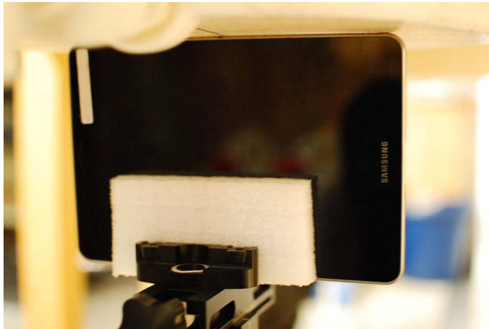
SAR Test Setup Photo 9 – Right at 0.0 cm
