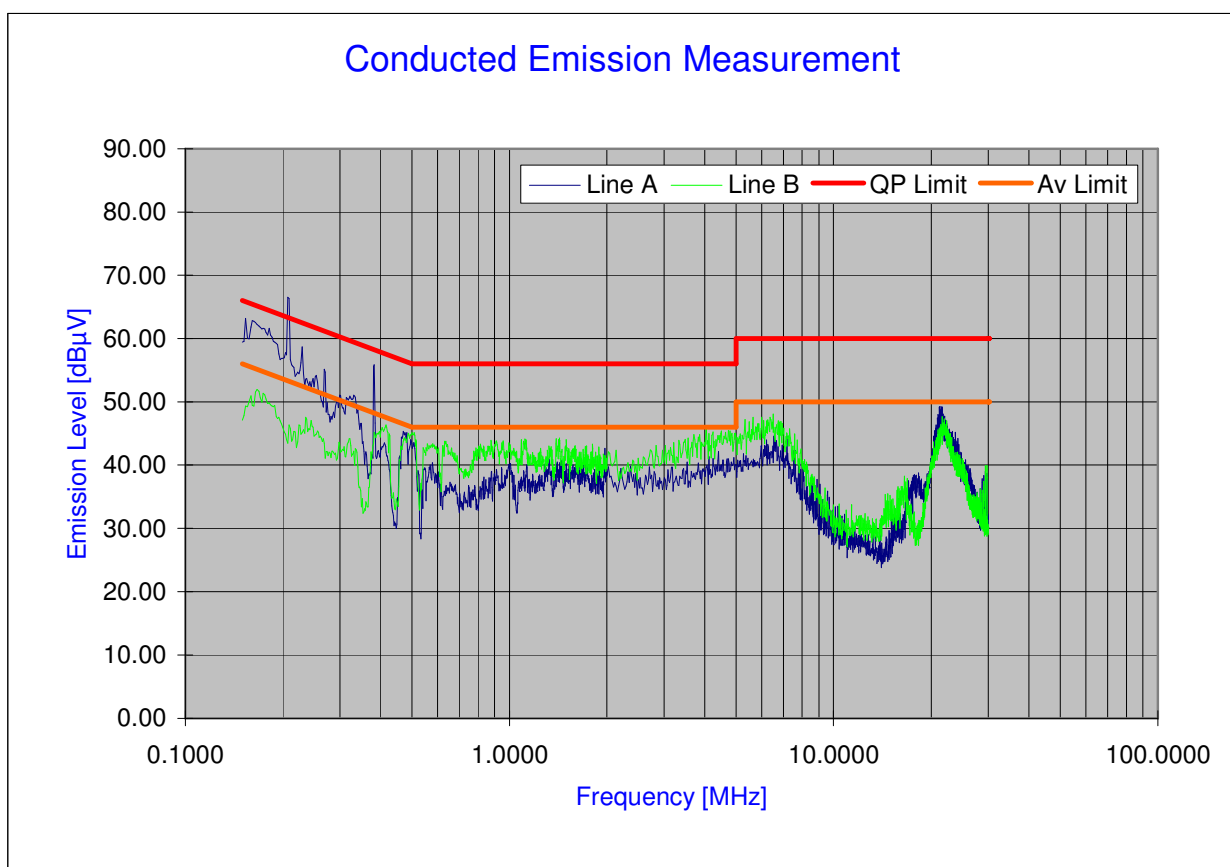
Plot 6-49. Line Conducted Plot with 802.11b
