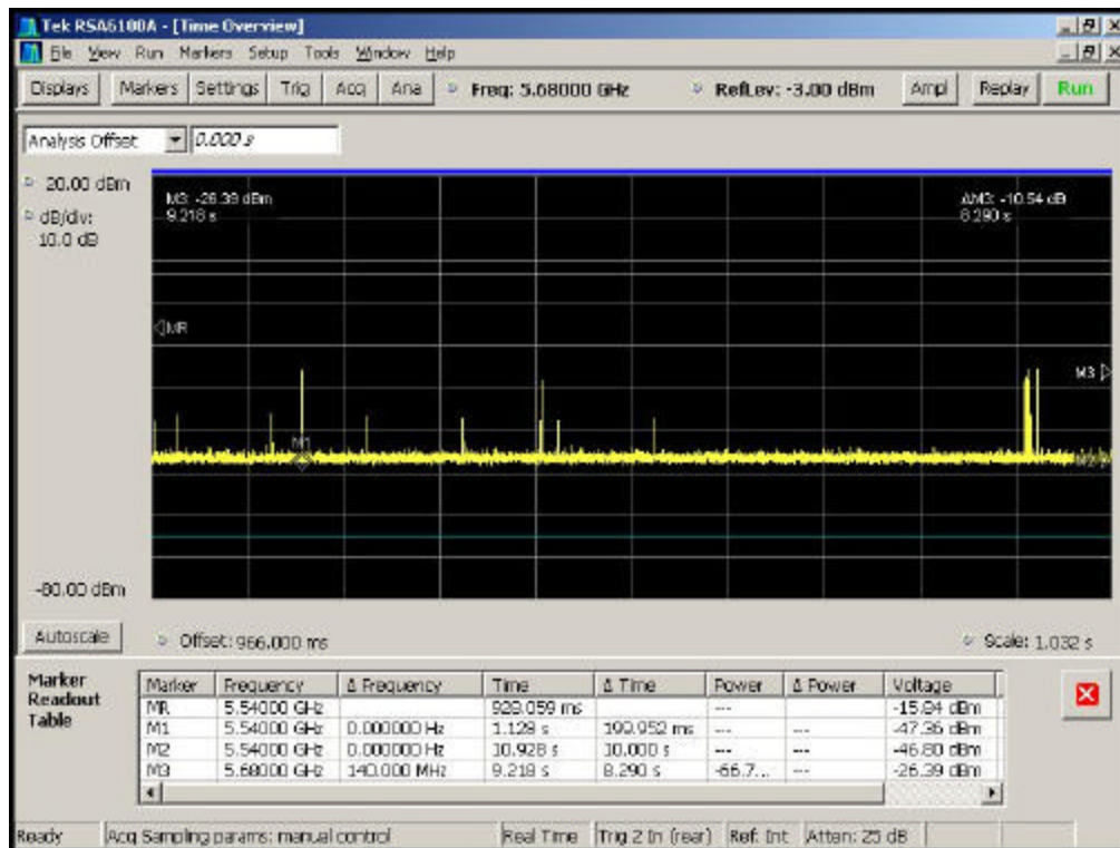
Figure 6-6. Pulse Grouping 1
