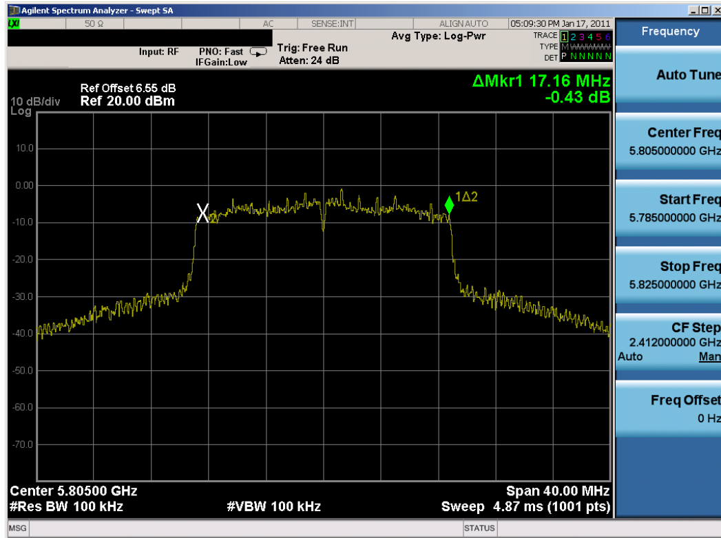
Plot 6-15. 6dB Bandwidth Plot (802.11n (5.8GHz) - Ch. 161)
