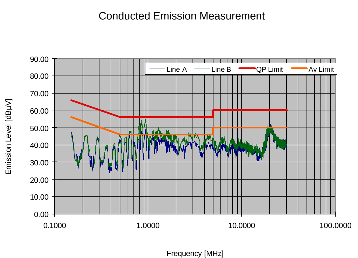
Plot 6-54. Line Conducted Plot with 802.11g
