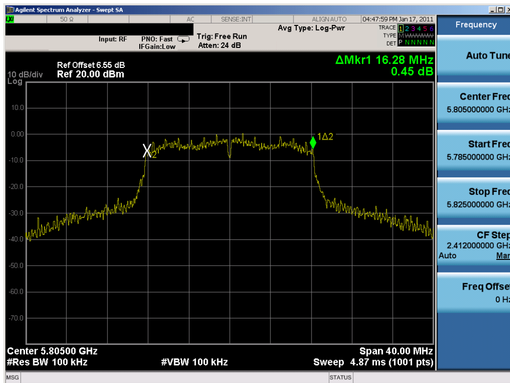
Plot 6-9. 6dB Bandwidth Plot (802.11a – Ch. 161)
