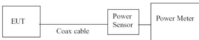
Figure 6-2. Test Instrument & Measurement Setup
