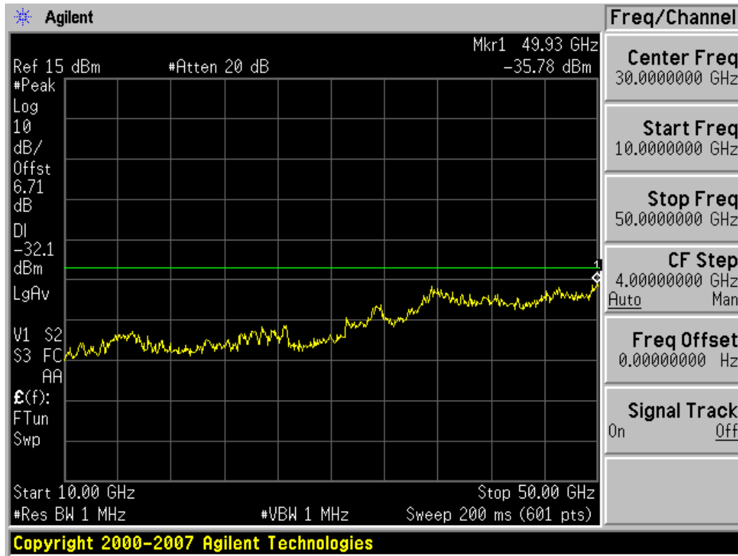
Plot 6-52. Conducted Spurious Plot (802.11a – Ch. 161)
