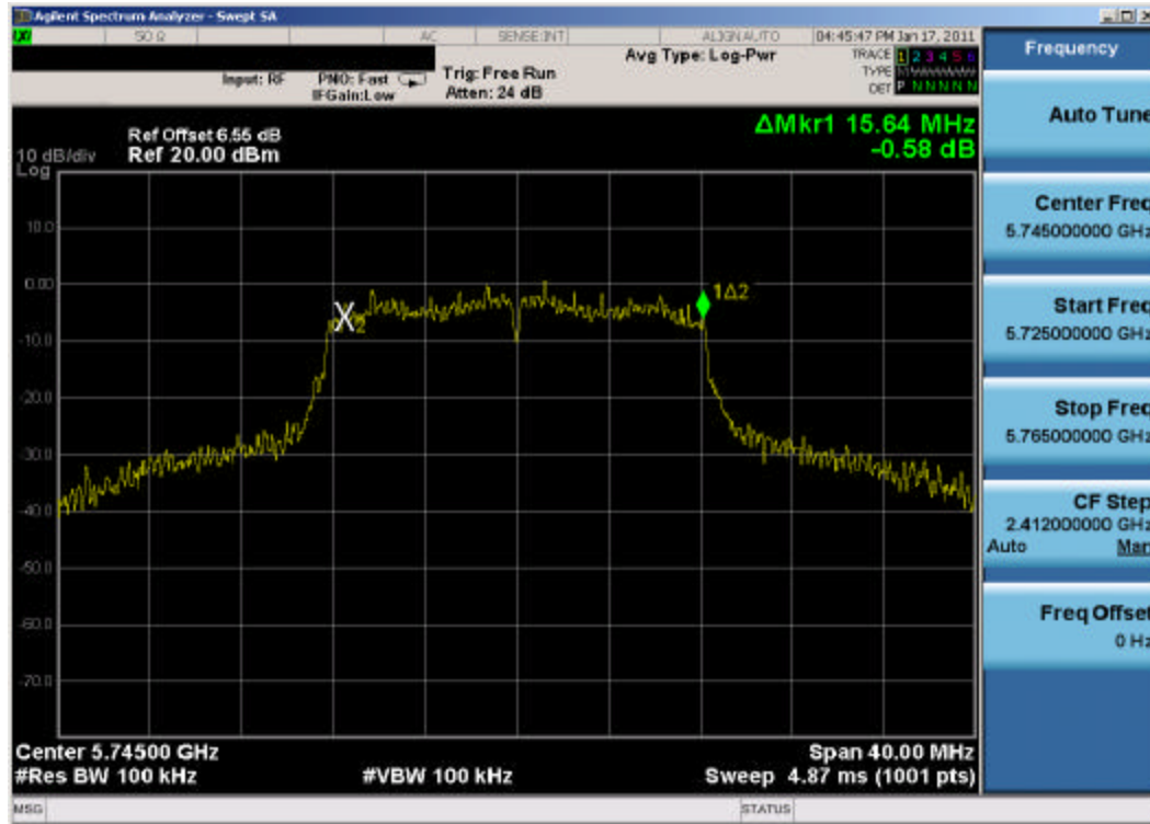
Plot 6-7. 6dB Bandwidth Plot (802.11a – Ch. 149)
